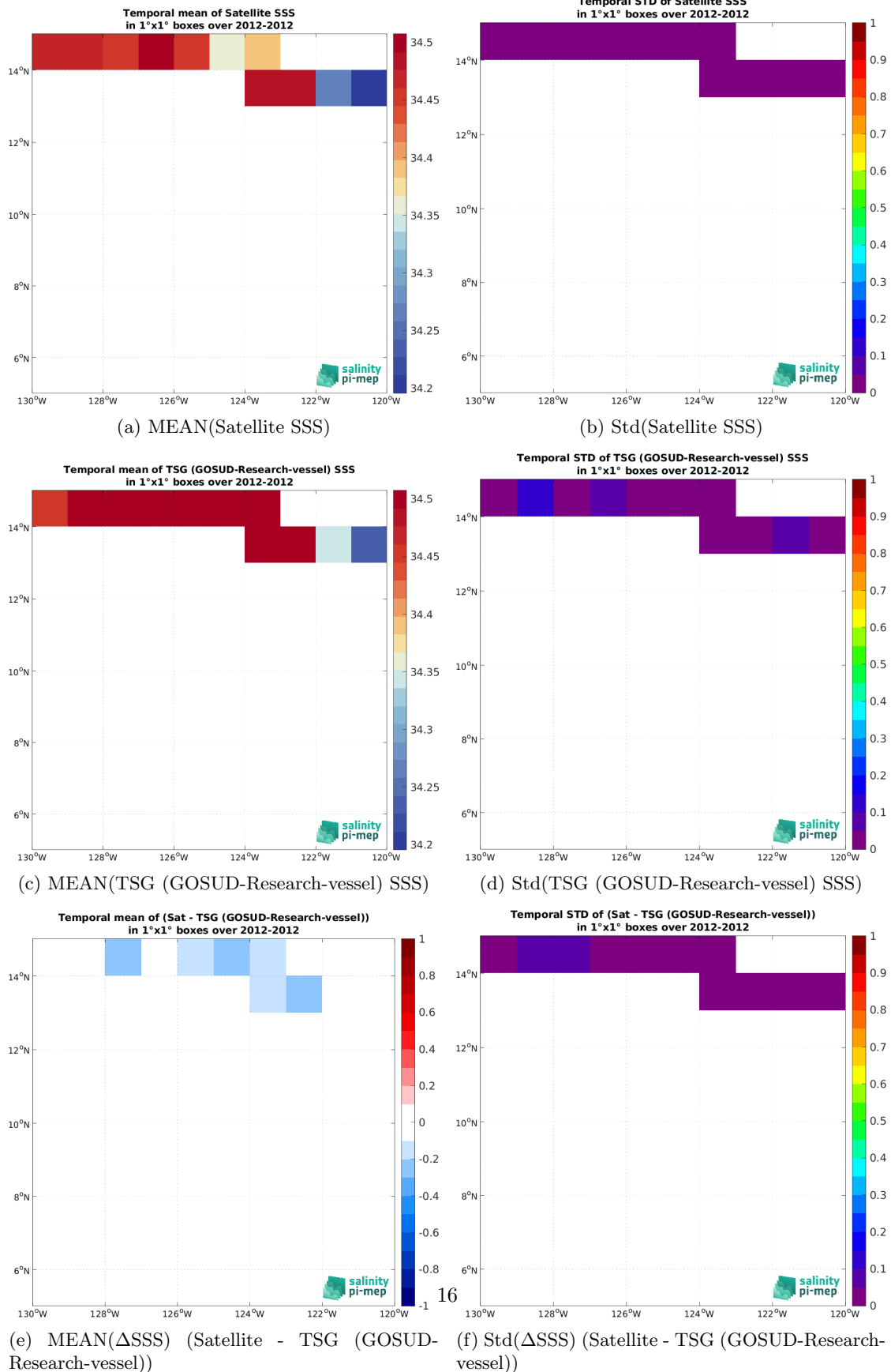
Figure 6: Temporal mean (left) and Std (right) of SSS from SMAP SSS L4 OI v2 - 7 Days (ESR) (top), TSG (GOSUD-Research-vessel) (middle), and of \Delta SSS (Satellite - TSG (GOSUD-Research-vessel)). Only match-up pairs are used to generate these maps.
