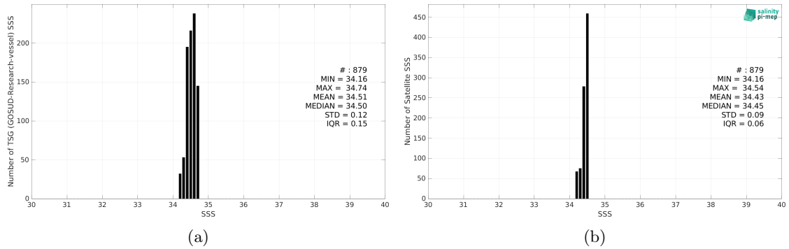
Figure 2: Histograms of SSS from TSG (GOSUD-Research-vessel) (a) and SMAP SSS L4 OI v2 - 7 Days (ESR) (b) considering all match-up pairs per bins of 0.1 over the SPURS 2 Pi-MEP region and for the full satellite product period.
