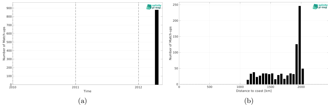
Figure 1: Number of match-ups between TSG (GOSUD-Research-vessel) and SMAP SSS L4 OI v2 - 7 Days (ESR) SSS as a function of time (a) and as function of the distance to coast (b) over the SPURS 2 Pi-MEP region and for the full satellite product period.
