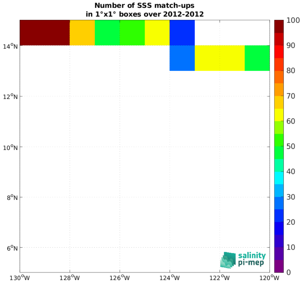
Figure 4: Number of SSS match-ups between TSG (GOSUD-Research-vessel) SSS and the SMAP SSS L4 OI v2 - 7 Days (ESR) SSS product for the SPURS 2 Pi-MEP region over 1^\circ \times 1^\circ boxes and for the full satellite product period.
