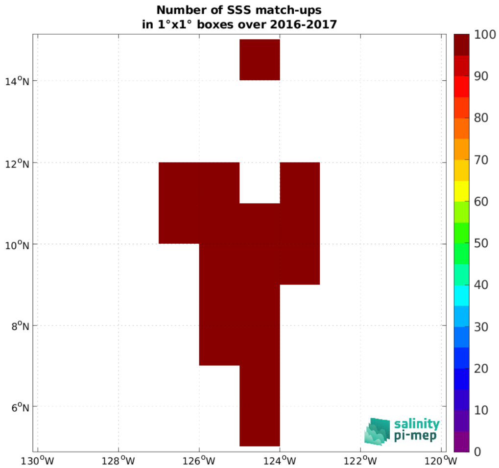
Figure 4: Number of SSS match-ups between Salinity Snake (SPURS 2) SSS and the SMAP SSS L4 OI v2 - 7 Days (ESR) SSS product for the SPURS 2 Pi-MEP region over 1^\circ \times 1^\circ boxes and for the full satellite product period.
