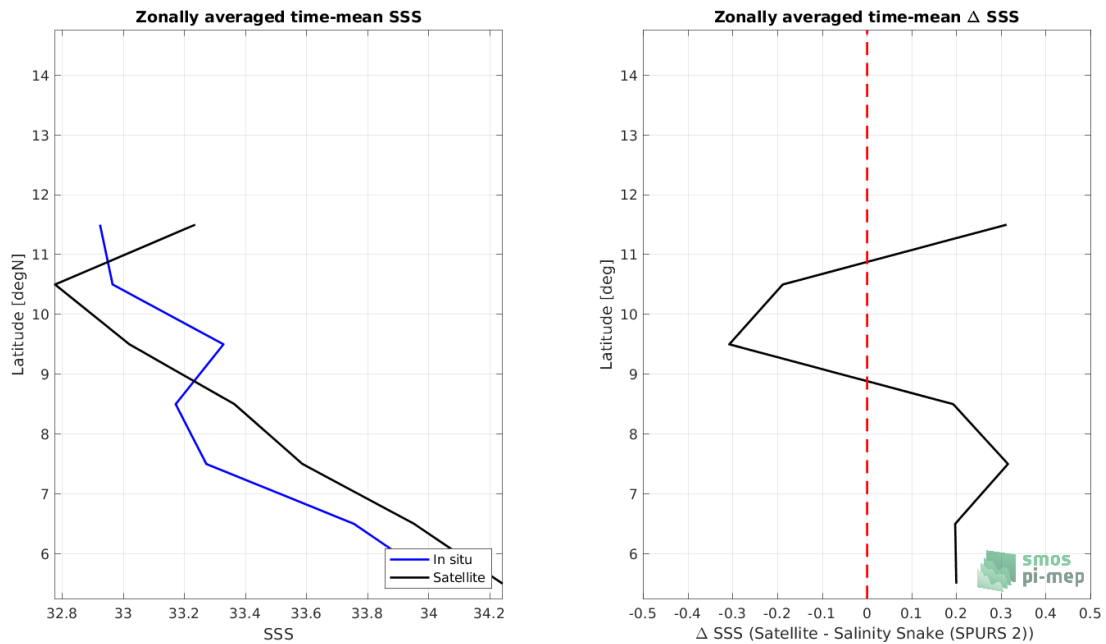
Figure 8: Left panel: Zonal mean SSS from SMAP SSS L4 OI v2 - 7 Days (ESR) satellite product (black) and from Salinity Snake (SPURS 2) (blue). Right panel: Zonal mean of \Delta SSS (Satellite - Salinity Snake (SPURS 2)) for all the collected Pi-MEP match-up pairs estimated over the full satellite product period.
