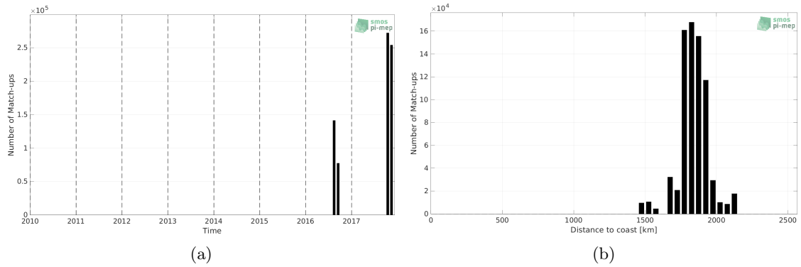
Figure 1: Number of match-ups between Salinity Snake (SPURS 2) and SMAP SSS L4 OI v2 - 7 Days (ESR) SSS as a function of time (a) and as function of the distance to coast (b) over the SPURS 2 Pi-MEP region and for the full satellite product period.
