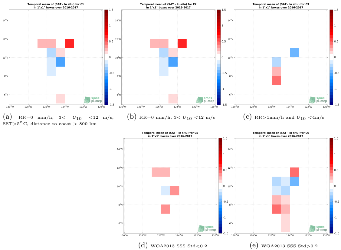
Figure 12: Temporal mean gridded over spatial boxes of size 1^\circ \times 1^\circ of \Delta SSS (SMAP SSS L4 OI v2 - 7 Days (ESR) - Salinity Snake (SPURS 2)) for 5 different subdatasets corresponding to:RR=0 mm/h, 3 < U_{10} < 12 m/s, SST>5°C, distance to coast > 800 km (a), RR=0 mm/h, 3 < U_{10} < 12 m/s (b), RR>1mm/h and U_{10} < 4 m/s (c), WOA2013 SSS Std<0.2 (d), WOA2013 SSS Std>0.2 (e).
