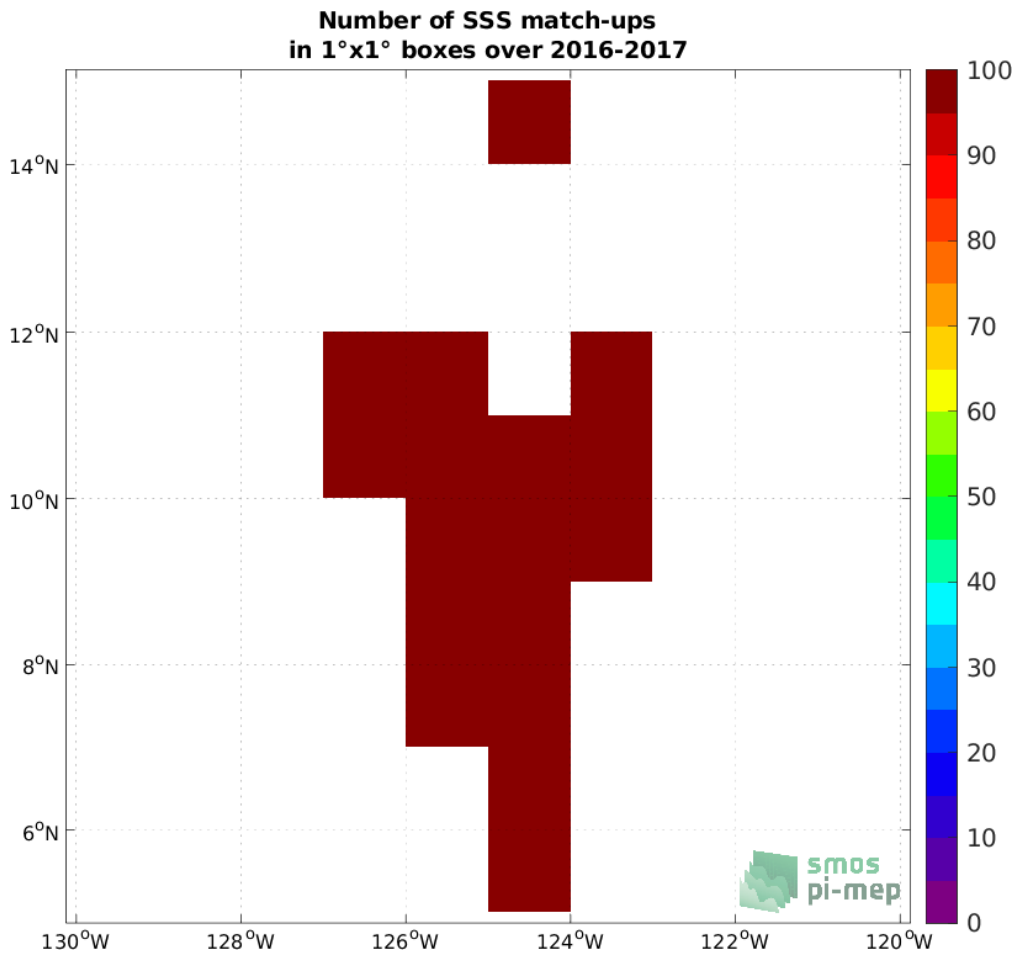
Figure 4: Number of SSS match-ups between Salinity Snake (SPURS 2) SSS and the SMAP SSS L4 OI v2 - 7 Days (ESR) SSS product for the SPURS 2 Pi-MEP region over 1°x1° boxes and for the full satellite product period.
