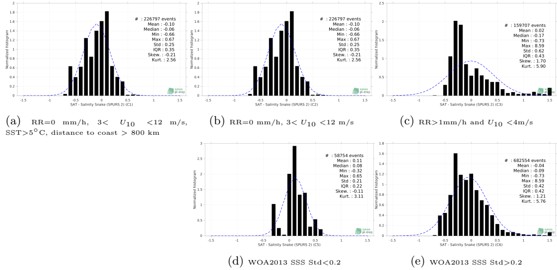
Figure 13: Normalized histogram of \Delta SSS (SMAP SSS L4 OI v2 - 7 Days (ESR) - Salinity Snake (SPURS 2)) for 5 different subdatasets corresponding to: RR=0 mm/h, 3 < U_{10} < 12 m/s, SST > 5°C, distance to coast > 800 km (a), RR=0 mm/h, 3 < U_{10} < 12 m/s (b), RR > 1mm/h and U_{10} < 4 m/s (c), WOA2013 SSS Std < 0.2 (d), WOA2013 SSS Std > 0.2 (e).
