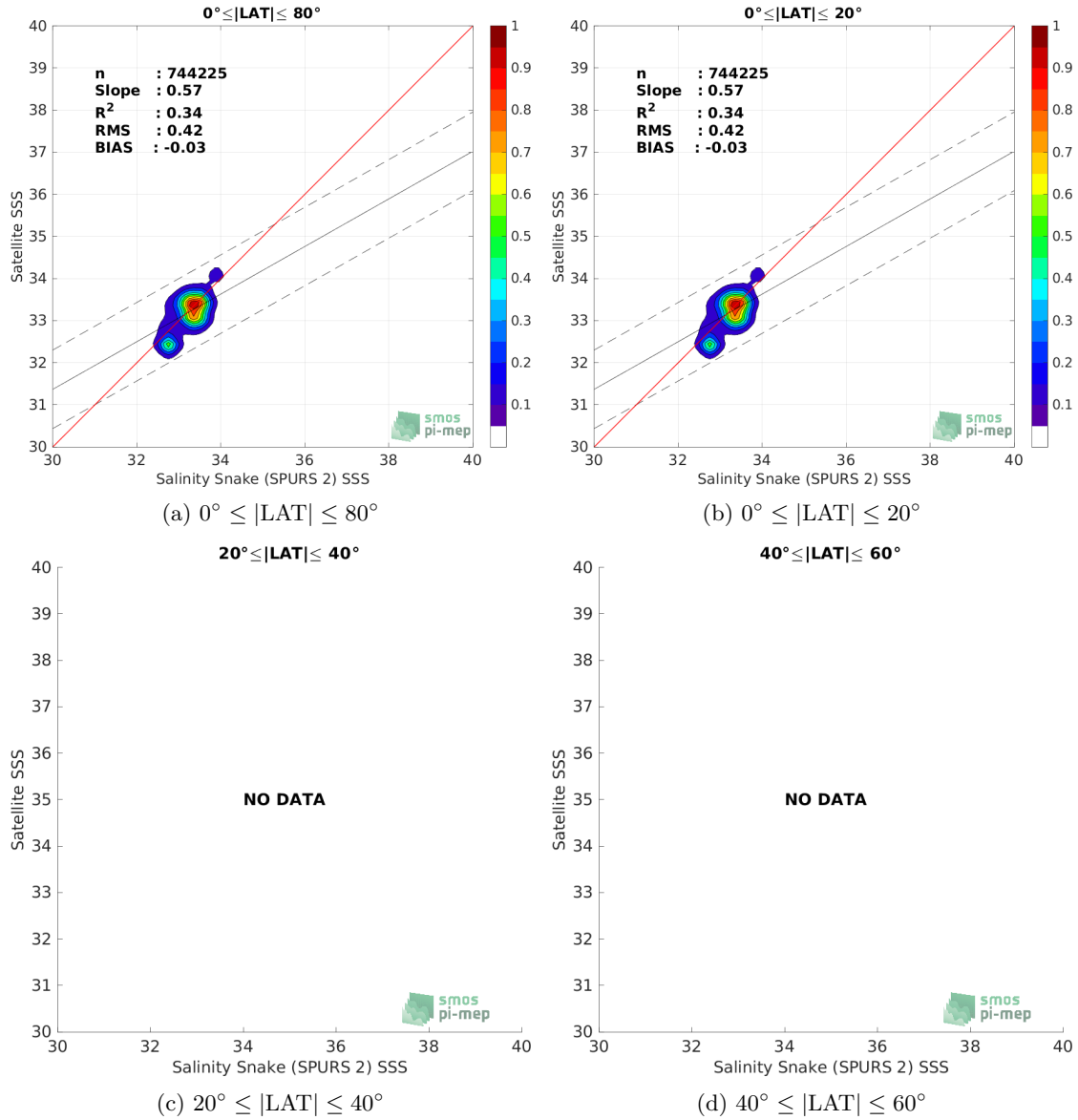
Figure 9: Contour maps of the concentration of SMAP SSS L4 OI v2 - 7 Days (ESR) SSS (y-axis) versus Salinity Snake (SPURS 2) SSS (x-axis) at match-up pairs for different latitude bands. For each plot, the red line shows x=y . The black thin and dashed lines indicate a linear fit through the data cloud and the \pm 95\% confidence levels, respectively. The number match-up pairs n , the slope and R^2 coefficient of the linear fit, the root mean square (RMS) and the mean bias between satellite and in situ data are indicated for each latitude band in each plots.
