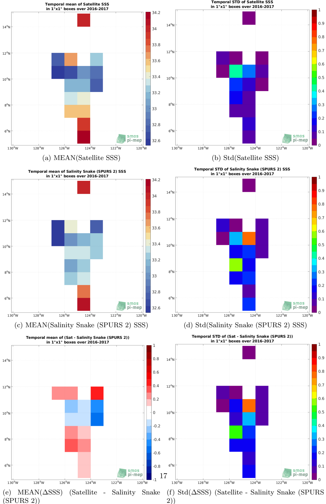
Figure 6: Temporal mean (left) and Std (right) of SSS from SMAP SSS L4 OI v2 - 7 Days (ESR) (top), Salinity Snake (SPURS 2) (middle), and of \Delta SSS (Satellite - Salinity Snake (SPURS 2)). Only match-up pairs are used to generate these maps.
