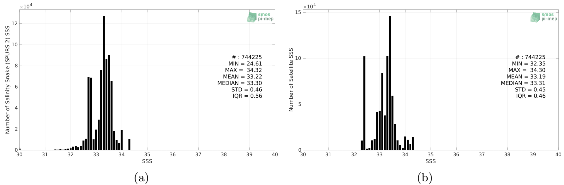
Figure 2: Histograms of SSS from Salinity Snake (SPURS 2) (a) and SMAP SSS L4 OI v2 - 7 Days (ESR) (b) considering all match-up pairs per bins of 0.1 over the SPURS 2 Pi-MEP region and for the full satellite product period.
