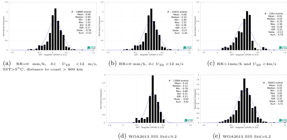
Figure 13: Normalized histogram of \Delta SSS (SMAP SSS L4 OI v2 - 7 Days (ESR) - Seaglider (SPURS 2)) for 5 different subdatasets corresponding to: RR=0 mm/h, 3 < U_{10} < 12 m/s, SST>5°C, distance to coast > 800 km (a), RR=0 mm/h, 3 < U_{10} < 12 m/s (b), RR>1mm/h and U_{10} < 4 m/s (c), WOA2013 SSS Std<0.2 (d), WOA2013 SSS Std>0.2 (e).
