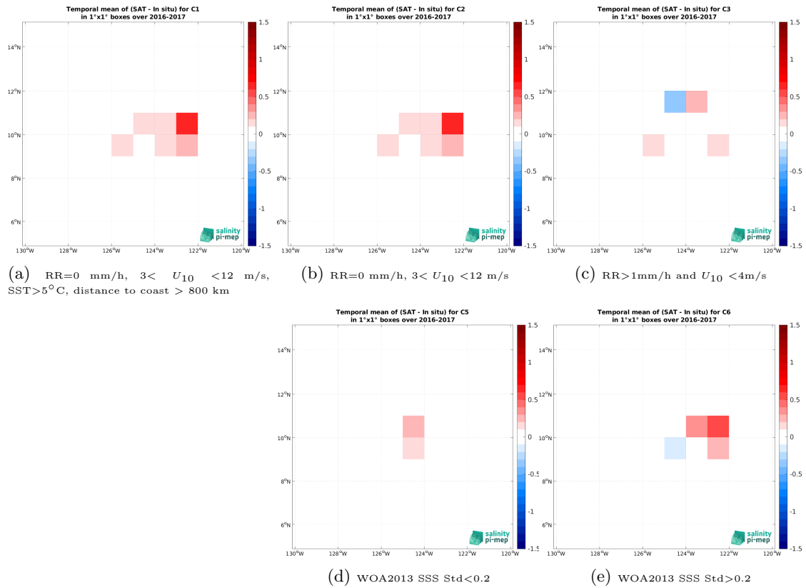
Figure 12: Temporal mean gridded over spatial boxes of size 1^\circ \times 1^\circ of \Delta\text{SSS} (SMAP SSS L4 OI v2 - 7 Days (ESR) - Seaglider (SPURS 2)) for 5 different subdatasets corresponding to:RR=0 mm/h, 3 < U_{10} < 12 m/s, SST >5^\circ\text{C} , distance to coast > 800 km (a), RR=0 mm/h, 3 < U_{10} < 12 m/s (b), RR >1 mm/h and U_{10} < 4 m/s (c), WOA2013 SSS Std <0.2 (d), WOA2013 SSS Std >0.2 (e).
