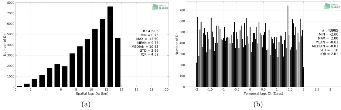
Figure 5: Histograms of the spatial (a) and temporal (b) lags between the location/time of the Seaglider (SPURS 2) measurement and the date of the corresponding SMAP SSS L4 OI v2 - 7 Days (ESR) SSS pixel.
