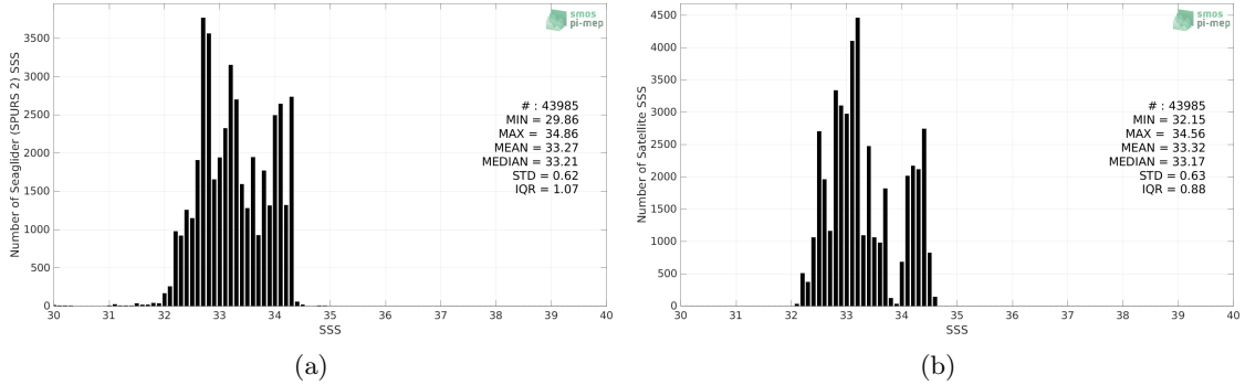
Figure 2: Histograms of SSS from Seaglider (SPURS 2) (a) and SMAP SSS L4 OI v2 - 7 Days (ESR) (b) considering all match-up pairs per bins of 0.1 over the SPURS 2 Pi-MEP region and for the full satellite product period.
