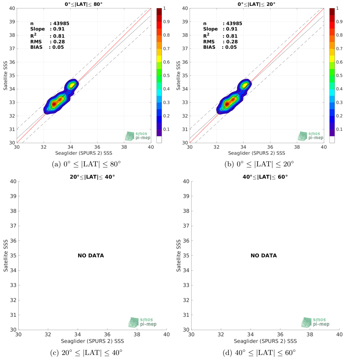
Figure 9: Contour maps of the concentration of SMAP SSS L4 OI v2 - 7 Days (ESR) SSS (y-axis) versus Seaglider (SPURS 2) SSS (x-axis) at match-up pairs for different latitude bands. For each plot, the red line shows x=y . The black thin and dashed lines indicate a linear fit through the data cloud and the \pm 95\% confidence levels, respectively. The number match-up pairs n , the slope and R^2 coefficient of the linear fit, the root mean square (RMS) and the mean bias between satellite and in situ data are indicated for each latitude band in each plots.
