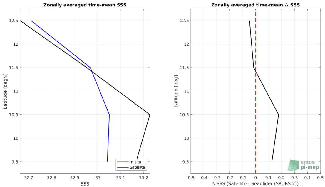
Figure 8: Left panel: Zonal mean SSS from SMAP SSS L4 OI v2 - 7 Days (ESR) satellite product (black) and from Seaglider (SPURS 2) (blue). Right panel: Zonal mean of \Delta SSS (Satellite - Seaglider (SPURS 2)) for all the collected Pi-MEP match-up pairs estimated over the full satellite product period.
