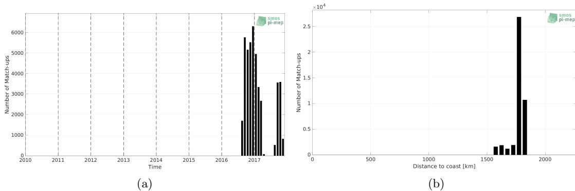
Figure 1: Number of match-ups between Seaglider (SPURS 2) and SMAP SSS L4 OI v2 - 7 Days (ESR) SSS as a function of time (a) and as function of the distance to coast (b) over the SPURS 2 Pi-MEP region and for the full satellite product period.
