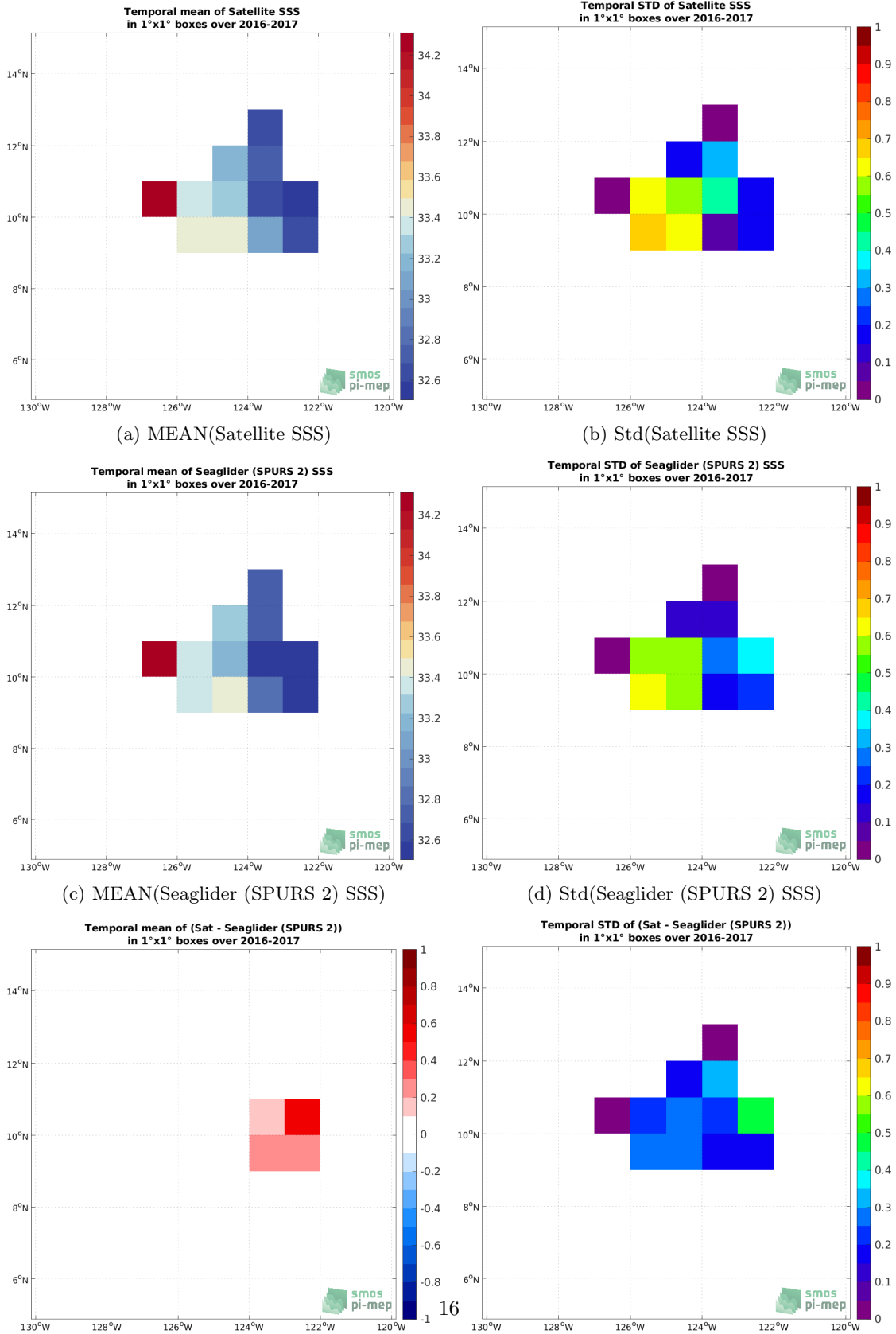
(e) MEAN( \Delta SSS) (Satellite - Seaglider (SPURS 2)) (f) Std( \Delta SSS) (Satellite - Seaglider (SPURS 2)) Figure 6: Temporal mean (left) and Std (right) of SSS from SMAP SSS L4 OI v2 - 7 Days (ESR) (top), Seaglider (SPURS 2) (middle), and of \Delta SSS (Satellite - Seaglider (SPURS 2)). Only match-up pairs are used to generate these maps.
