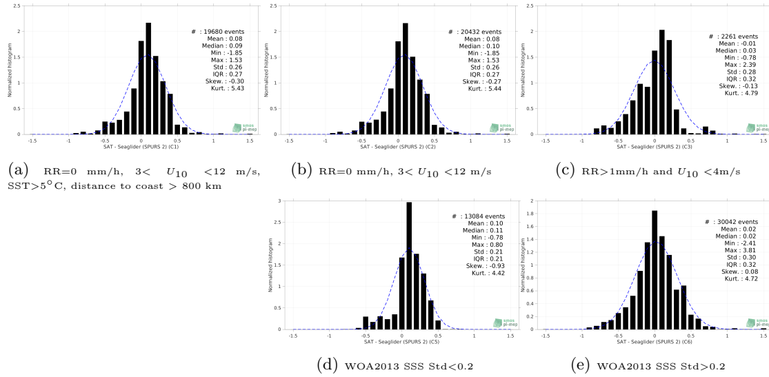
Figure 13: Normalized histogram of \Delta SSS (SMAP SSS L4 OI v2 - 7 Days (ESR) - Seaglider (SPURS 2)) for 5 different subdatasets corresponding to: RR=0 mm/h, 3 < U_{10} < 12 m/s, SST > 5°C, distance to coast > 800 km (a), RR=0 mm/h, 3 < U_{10} < 12 m/s (b), RR > 1mm/h and U_{10} < 4 m/s (c), WOA2013 SSS Std < 0.2 (d), WOA2013 SSS Std > 0.2 (e).
