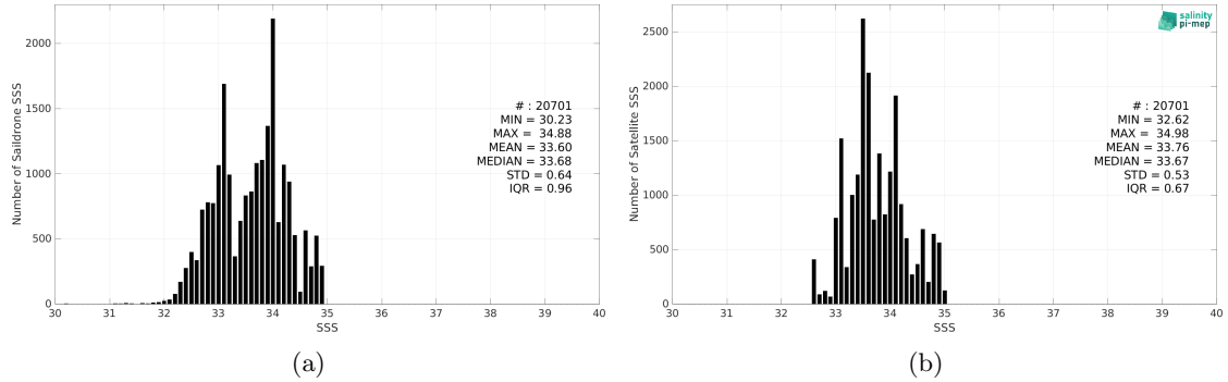
Figure 2: Histograms of SSS from Saildrone (a) and SMAP SSS L4 OI v2 - 7 Days (ESR) (b) considering all match-up pairs per bins of 0.1 over the SPURS 2 Pi-MEP region and for the full satellite product period.
