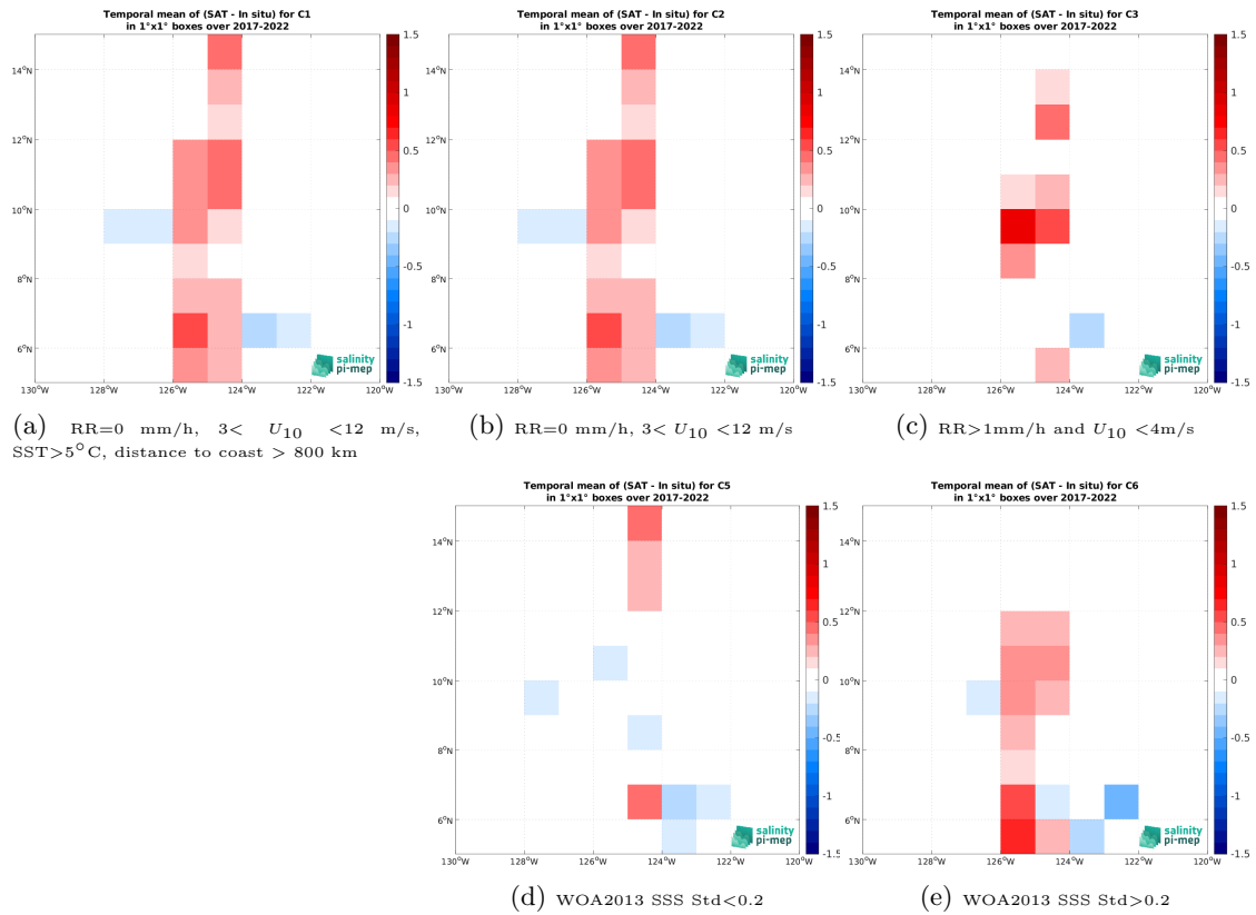
Figure 12: Temporal mean gridded over spatial boxes of size 1^\circ \times 1^\circ of \Delta\text{SSS} (SMAP SSS L4 OI v2 - 7 Days (ESR) - Saildrone) for 5 different subdatasets corresponding to:RR=0 mm/h, 3 < U_{10} < 12 m/s, SST >5^\circ\text{C} , distance to coast > 800 km (a), RR=0 mm/h, 3 < U_{10} < 12 m/s (b), RR >1 mm/h and U_{10} < 4 m/s (c), WOA2013 SSS Std <0.2 (d), WOA2013 SSS Std >0.2 (e).
