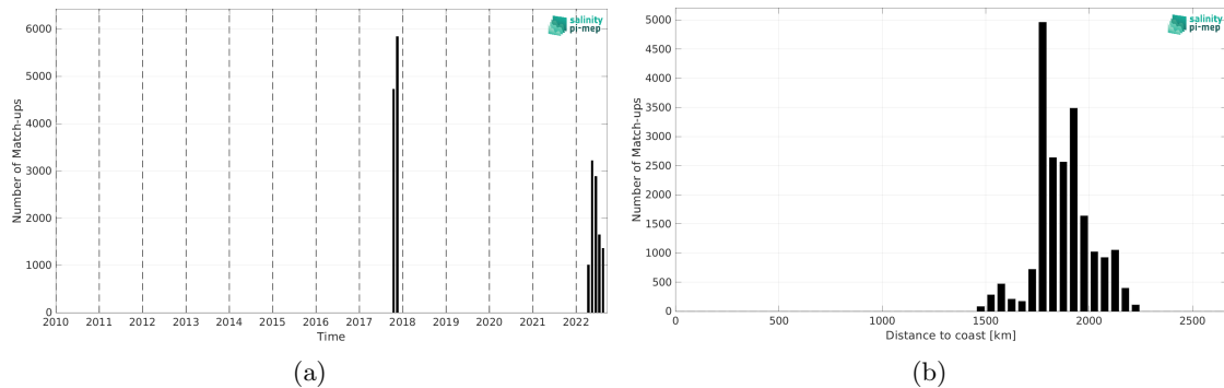
Figure 1: Number of match-ups between Saildrone and SMAP SSS L4 OI v2 - 7 Days (ESR) SSS as a function of time (a) and as function of the distance to coast (b) over the SPURS 2 Pi-MEP region and for the full satellite product period.
