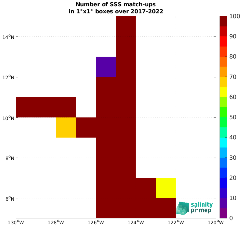
Figure 4: Number of SSS match-ups between Saildrone SSS and the SMAP SSS L4 OI v2 - 7 Days (ESR) SSS product for the SPURS 2 Pi-MEP region over 1^\circ \times 1^\circ boxes and for the full satellite product period.
