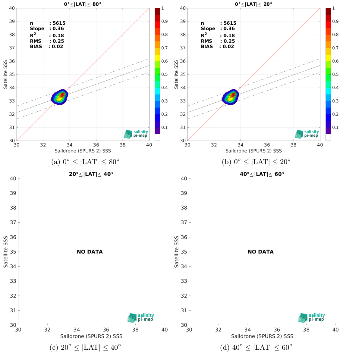
Figure 9: Contour maps of the concentration of SMAP SSS L4 OI v2 - 7 Days (ESR) SSS (y-axis) versus Saildrone (SPURS 2) SSS (x-axis) at match-up pairs for different latitude bands. For each plot, the red line shows x=y . The black thin and dashed lines indicate a linear fit through the data cloud and the \pm 95\% confidence levels, respectively. The number match-up pairs n , the slope and R^2 coefficient of the linear fit, the root mean square (RMS) and the mean bias between satellite and in situ data are indicated for each latitude band in each plots.
