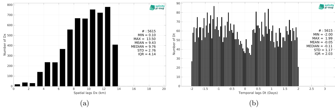
Figure 5: Histograms of the spatial (a) and temporal (b) lags between the location/time of the Saildrone (SPURS 2) measurement and the date of the corresponding SMAP SSS L4 OI v2 - 7 Days (ESR) SSS pixel.
