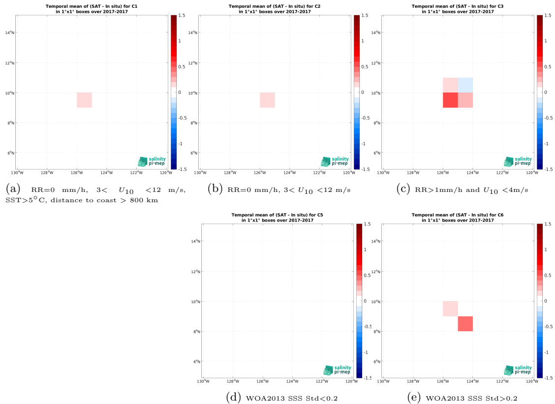
Figure 12: Temporal mean gridded over spatial boxes of size 1^\circ \times 1^\circ of \Delta\text{SSS} (SMAP SSS L4 OI v2 - 7 Days (ESR) - Saildrone (SPURS 2)) for 5 different subdatasets corresponding to:RR=0 mm/h, 3 < U_{10} < 12 m/s, SST >5^\circ\text{C} , distance to coast > 800 km (a), RR=0 mm/h, 3 < U_{10} < 12 m/s (b), RR >1 mm/h and U_{10} < 4 m/s (c), WOA2013 SSS Std <0.2 (d), WOA2013 SSS Std >0.2 (e).
