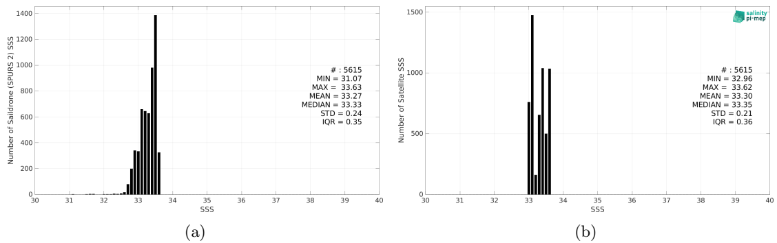
Figure 2: Histograms of SSS from Saildrone (SPURS 2) (a) and SMAP SSS L4 OI v2 - 7 Days (ESR) (b) considering all match-up pairs per bins of 0.1 over the SPURS 2 Pi-MEP region and for the full satellite product period.
