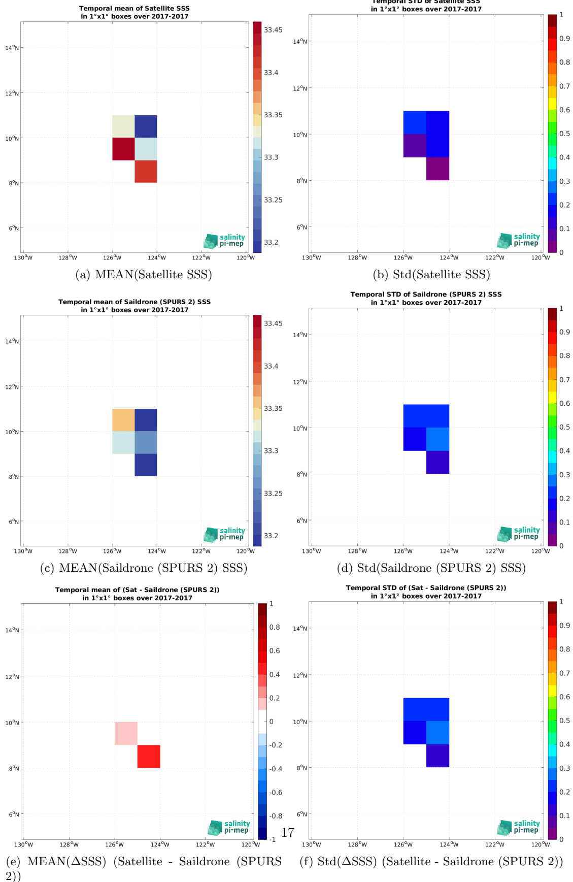
Figure 6: Temporal mean (left) and Std (right) of SSS from SMAP SSS L4 OI v2 - 7 Days (ESR) (top), Saildrone (SPURS 2) (middle), and of \Delta SSS (Satellite - Saildrone (SPURS 2)). Only match-up pairs are used to generate these maps.
