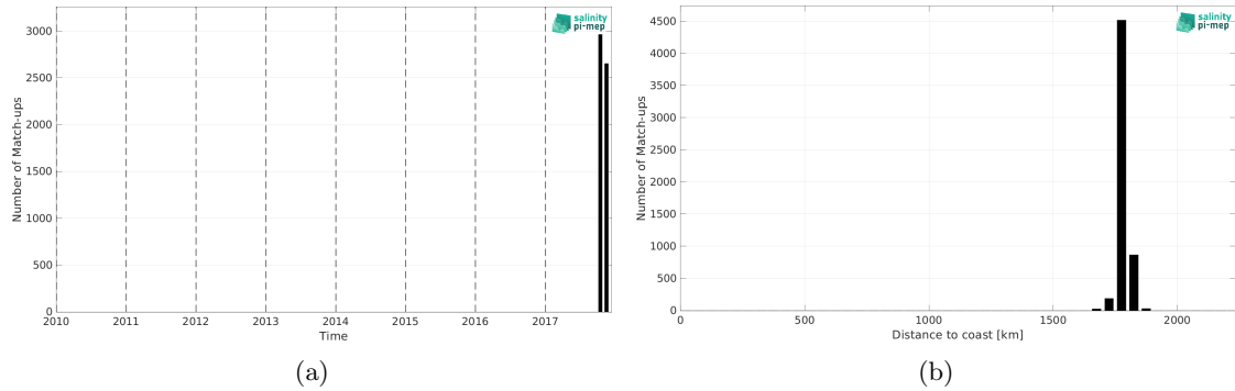
Figure 1: Number of match-ups between Saildrone (SPURS 2) and SMAP SSS L4 OI v2 - 7 Days (ESR) SSS as a function of time (a) and as function of the distance to coast (b) over the SPURS 2 Pi-MEP region and for the full satellite product period.
