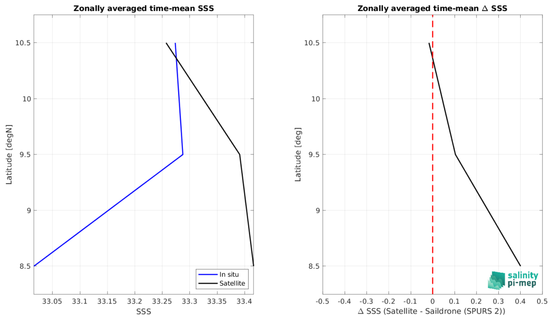
Figure 8: Left panel: Zonal mean SSS from SMAP SSS L4 OI v2 - 7 Days (ESR) satellite product (black) and from Sairdron (SPURS 2) (blue). Right panel: Zonal mean of \Delta SSS (Satellite - Sairdron (SPURS 2)) for all the collected Pi-MEP match-up pairs estimated over the full satellite product period.
