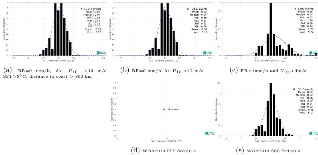
Figure 13: Normalized histogram of \Delta SSS (SMAP SSS L4 OI v2 - 7 Days (ESR) - Saldrone (SPURS 2)) for 5 different subdatasets corresponding to: RR=0 mm/h, 3 < U_{10} < 12 m/s, SST > 5°C, distance to coast > 800 km (a), RR=0 mm/h, 3 < U_{10} < 12 m/s (b), RR > 1mm/h and U_{10} < 4 m/s (c), WOA2013 SSS Std < 0.2 (d), WOA2013 SSS Std > 0.2 (e).
