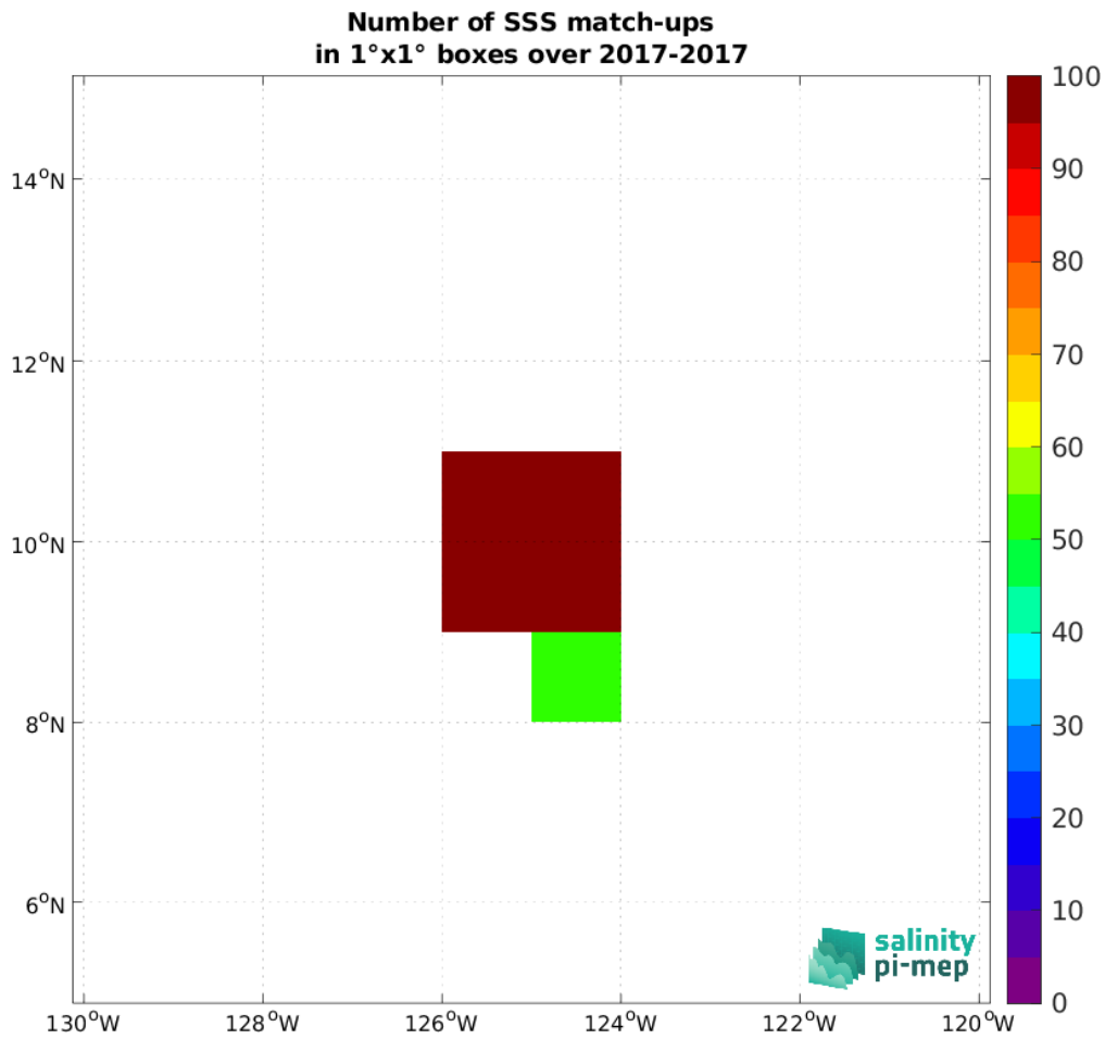
Figure 4: Number of SSS match-ups between Saildrone (SPURS 2) SSS and the SMAP SSS L4 OI v2 - 7 Days (ESR) SSS product for the SPURS 2 Pi-MEP region over 1°x1° boxes and for the full satellite product period.
