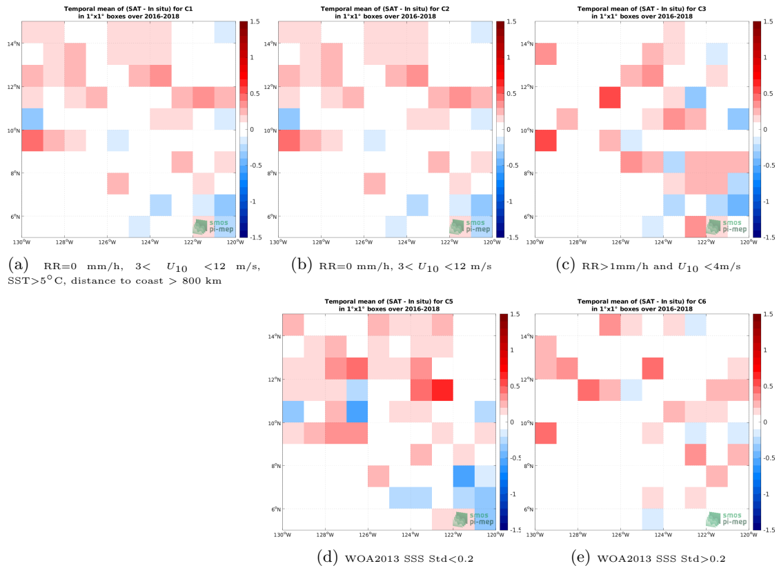
Figure 11: Temporal mean gridded over spatial boxes of size 1^\circ \times 1^\circ of \Delta SSS (SMAP SSS L4 OI v2 - 7 Days (ESR) - Surface drifters) for 5 different subdatasets corresponding to:RR=0 mm/h, 3 < U_{10} < 12 m/s, SST >5^\circ C, distance to coast > 800 km (a), RR=0 mm/h, 3 < U_{10} < 12 m/s (b), RR >1 mm/h and U_{10} < 4 m/s (c), WOA2013 SSS Std <0.2 (d), WOA2013 SSS Std >0.2 (e).
