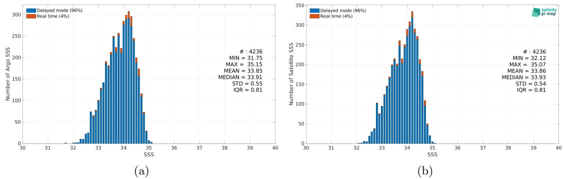
Figure 2: Histograms of SSS from Argo (a) and SMAP SSS L4 OI v2 - 7 Days (ESR) (b) considering all match-up pairs per bins of 0.1 over the SPURS 2 Pi-MEP region and for the full satellite product period.
