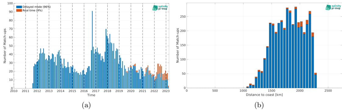
Figure 1: Number of match-ups between Argo and SMAP SSS L4 OI v2 - 7 Days (ESR) SSS as a function of time (a) and as function of the distance to coast (b) over the SPURS 2 Pi-MEP region and for the full satellite product period.
