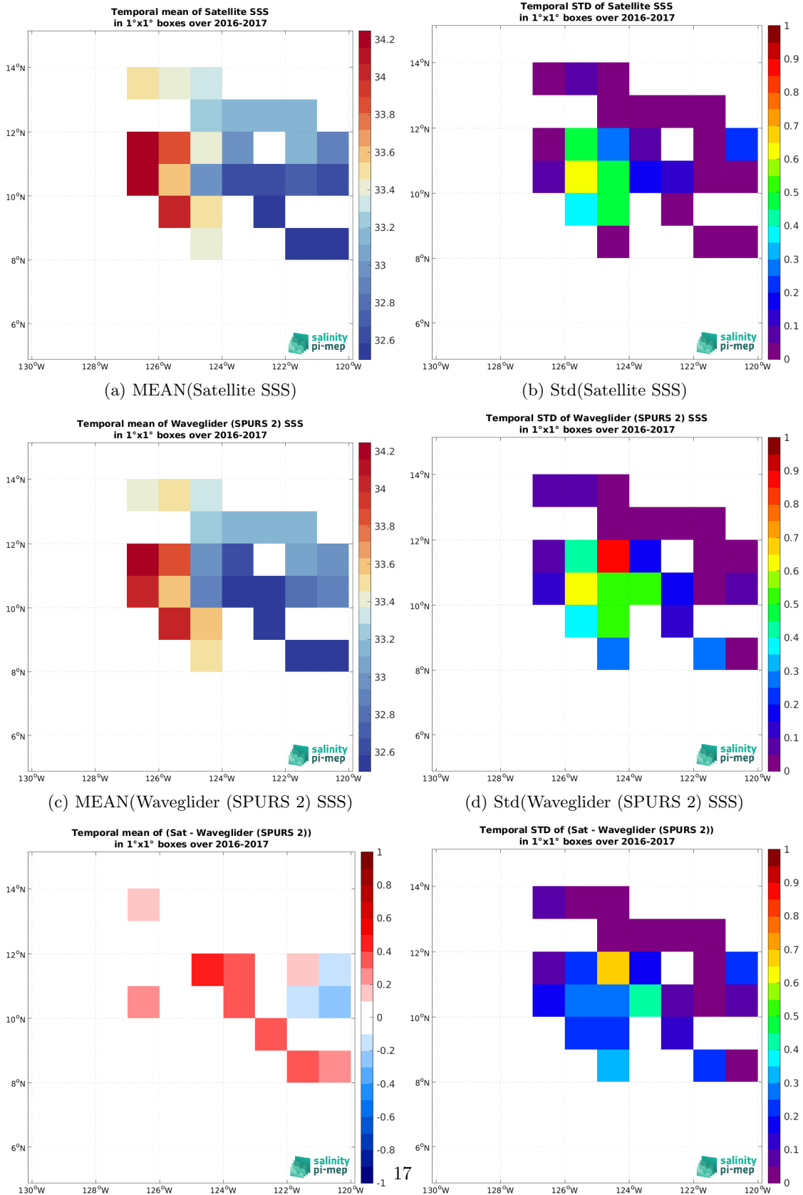
Figure 6: Temporal mean (left) and Std (right) of SSS from SMAP SSS L4 OI v2 - Monthly (IPRC) (top), Waveglider (SPURS 2) (middle), and of \Delta SSS (Satellite - Waveglider (SPURS 2)). Only match-up pairs are used to generate these maps.
