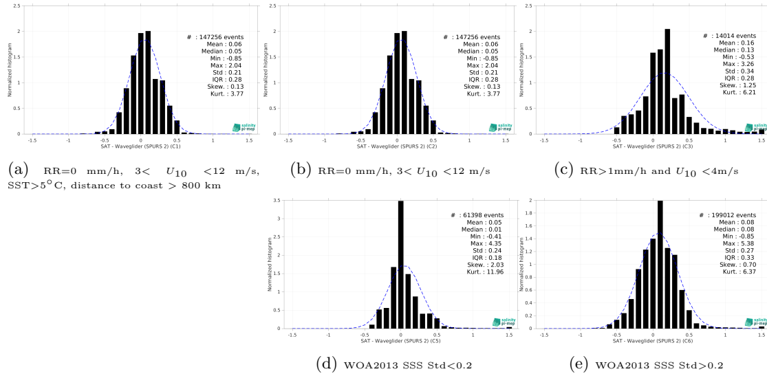
Figure 13: Normalized histogram of \Delta SSS (SMAP SSS L4 OI v2 - Monthly (IPRC) - Waveglider (SPURS 2)) for 5 different subdatasets corresponding to: RR=0 mm/h, 3 < U_{10} < 12 m/s, SST > 5°C, distance to coast > 800 km (a), RR=0 mm/h, 3 < U_{10} < 12 m/s (b), RR > 1mm/h and U_{10} < 4 m/s (c), WOA2013 SSS Std < 0.2 (d), WOA2013 SSS Std > 0.2 (e).
