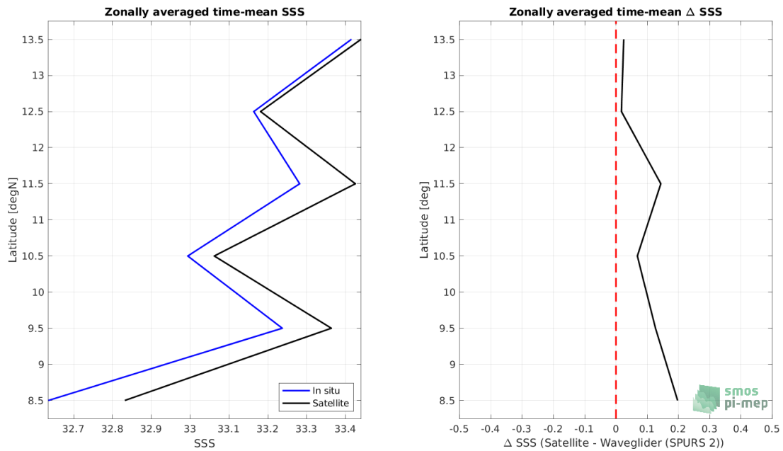
Figure 8: Left panel: Zonal mean SSS from SMAP SSS L4 OI v2 - Monthly (IPRC) satellite product (black) and from Waveglider (SPURS 2) (blue). Right panel: Zonal mean of \Delta SSS (Satellite - Waveglider (SPURS 2)) for all the collected Pi-MEP match-up pairs estimated over the full satellite product period.
