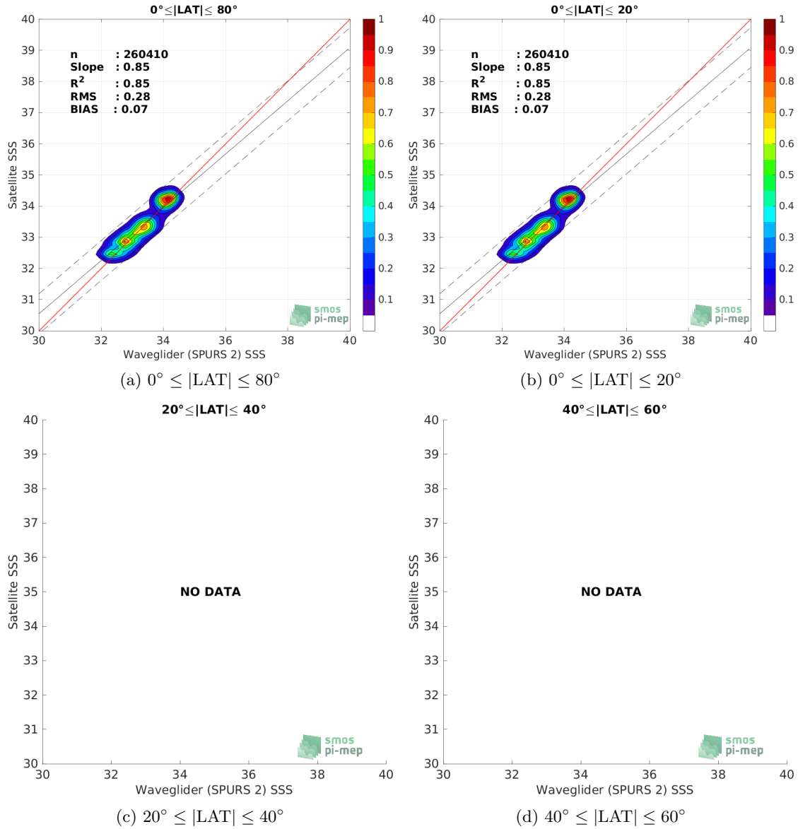
Figure 9: Contour maps of the concentration of SMAP SSS L4 OI v2 - Monthly (IPRC) SSS (y-axis) versus Waveglider (SPURS 2) SSS (x-axis) at match-up pairs for different latitude bands. For each plot, the red line shows x=y . The black thin and dashed lines indicate a linear fit through the data cloud and the \pm 95\% confidence levels, respectively. The number match-up pairs n , the slope and R^2 coefficient of the linear fit, the root mean square (RMS) and the mean bias between satellite and in situ data are indicated for each latitude band in each plots.
