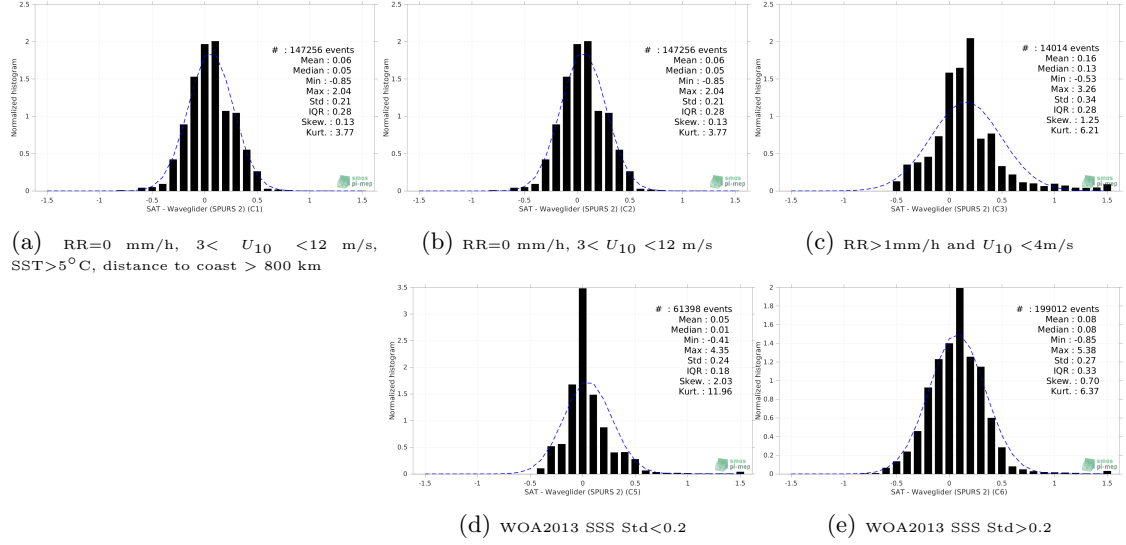
Figure 13: Normalized histogram of \Delta SSS (SMAP SSS L4 OI v2 - Monthly (IPRC) - Waveglider (SPURS 2)) for 5 different subdatasets corresponding to: RR=0 mm/h, 3 < U_{10} < 12 m/s, SST > 5°C, distance to coast > 800 km (a), RR=0 mm/h, 3 < U_{10} < 12 m/s (b), RR > 1mm/h and U_{10} < 4 m/s (c), WOA2013 SSS Std < 0.2 (d), WOA2013 SSS Std > 0.2 (e).
