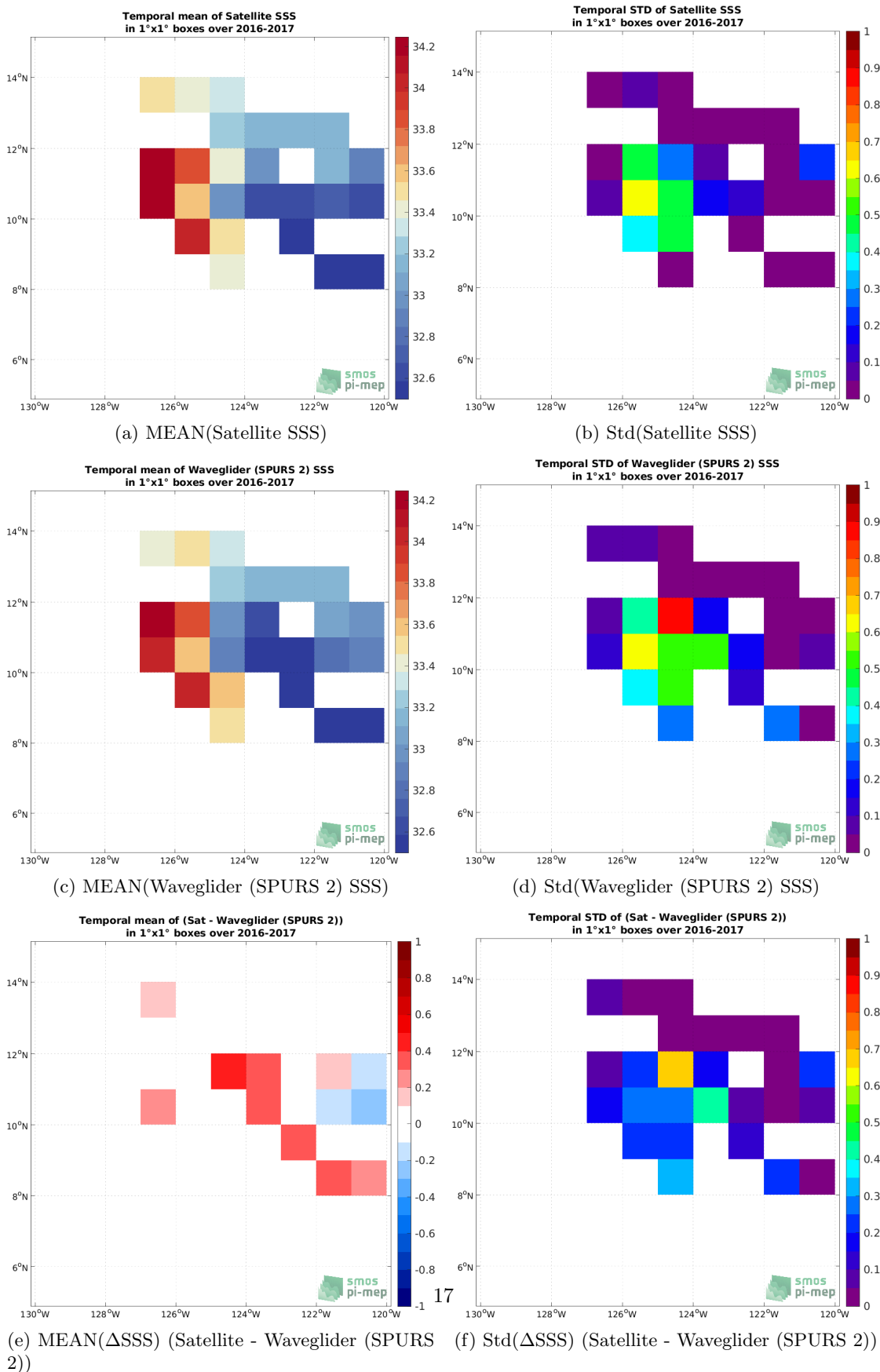
Figure 6: Temporal mean (left) and Std (right) of SSS from SMAP SSS L4 OI v2 - Monthly (IPRC) (top), Waveglider (SPURS 2) (middle), and of \Delta SSS (Satellite - Waveglider (SPURS 2)). Only match-up pairs are used to generate these maps.
