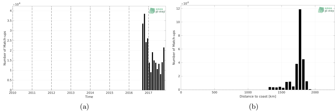
Figure 1: Number of match-ups between Waveglider (SPURS 2) and SMAP SSS L4 OI v2 - Monthly (IPRC) SSS as a function of time (a) and as function of the distance to coast (b) over the SPURS 2 Pi-MEP region and for the full satellite product period.
