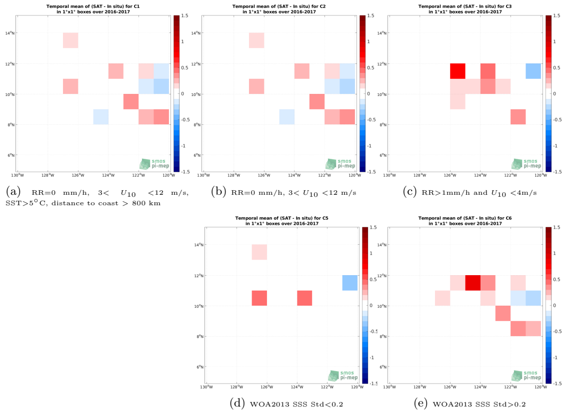
Figure 12: Temporal mean gridded over spatial boxes of size 1^\circ \times 1^\circ of \Delta SSS (SMAP SSS L4 OI v2 - Monthly (IPRC) - Waveglider (SPURS 2)) for 5 different subdatasets corresponding to:RR=0 mm/h, 3 < U_{10} < 12 m/s, SST >5^\circ C, distance to coast > 800 km (a), RR=0 mm/h, 3 < U_{10} < 12 m/s (b), RR >1 mm/h and U_{10} < 4 m/s (c), WOA2013 SSS Std <0.2 (d), WOA2013 SSS Std >0.2 (e).
