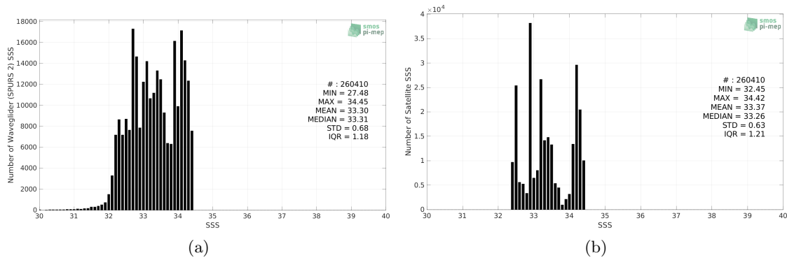
Figure 2: Histograms of SSS from Waveglider (SPURS 2) (a) and SMAP SSS L4 OI v2 - Monthly (IPRC) (b) considering all match-up pairs per bins of 0.1 over the SPURS 2 Pi-MEP region and for the full satellite product period.
