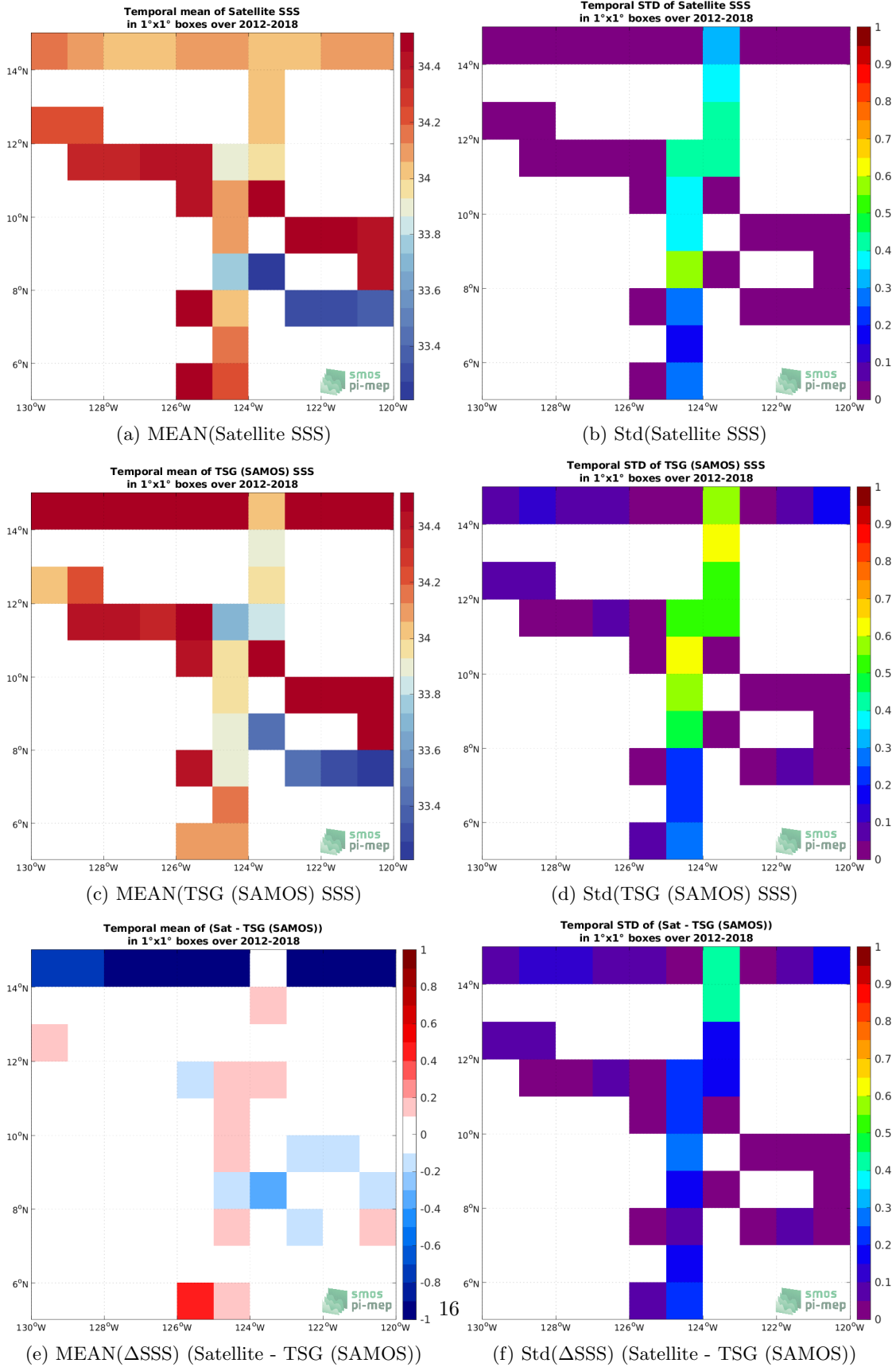
Figure 6: Temporal mean (left) and Std (right) of SSS from SMAP SSS L4 OI v2 - Monthly (IPRC) (top), TSG (SAMOS) (middle), and of \Delta SSS (Satellite - TSG (SAMOS)). Only match-up pairs are used to generate these maps.
