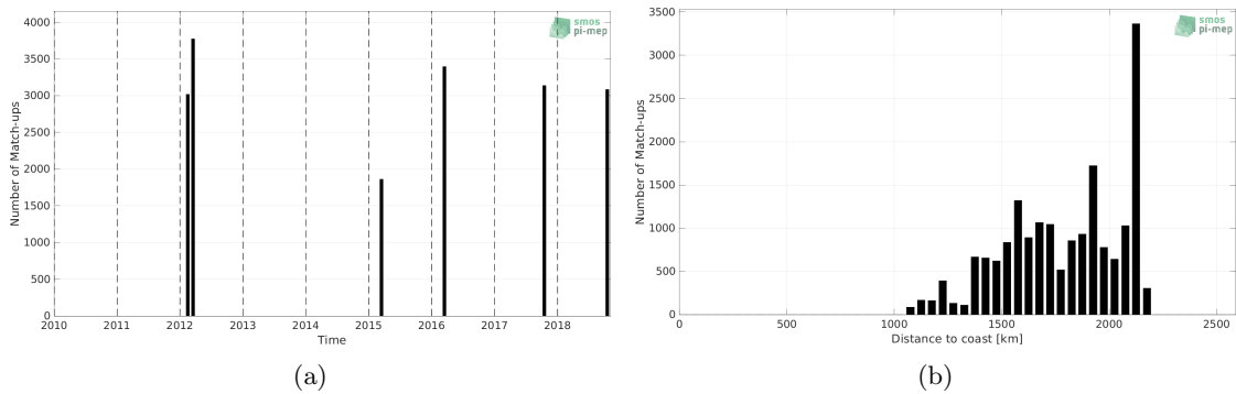
Figure 1: Number of match-ups between TSG (SAMOS) and SMAP SSS L4 OI v2 - Monthly (IPRC) SSS as a function of time (a) and as function of the distance to coast (b) over the SPURS 2 Pi-MEP region and for the full satellite product period.
