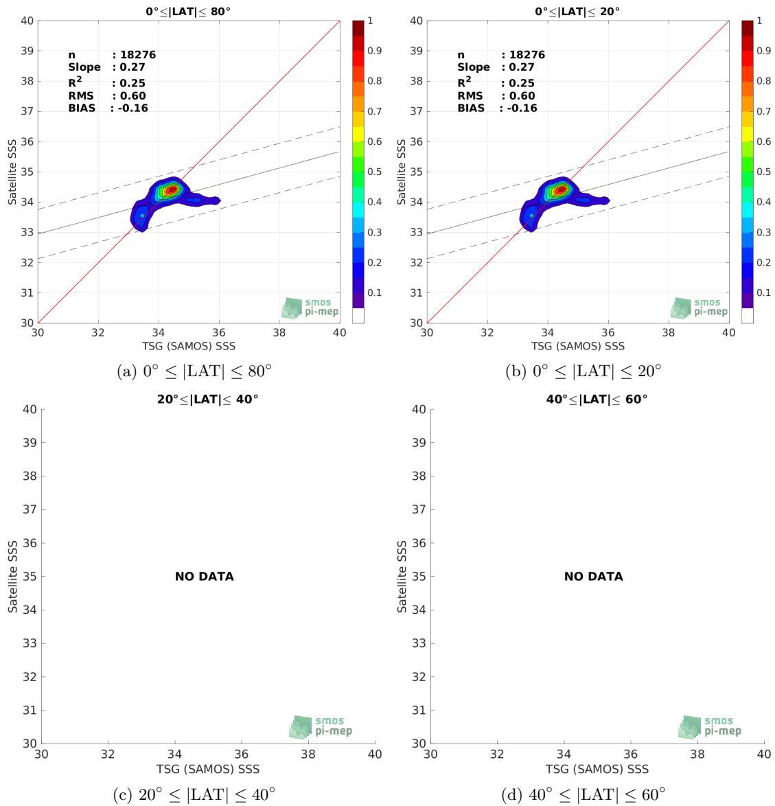
Figure 9: Contour maps of the concentration of SMAP SSS L4 OI v2 - Monthly (IPRC) SSS (y-axis) versus TSG (SAMOS) SSS (x-axis) at match-up pairs for different latitude bands. For each plot, the red line shows x=y . The black thin and dashed lines indicate a linear fit through the data cloud and the \pm 95\% confidence levels, respectively. The number match-up pairs n , the slope and R^2 coefficient of the linear fit, the root mean square (RMS) and the mean bias between satellite and in situ data are indicated for each latitude band in each plots.
