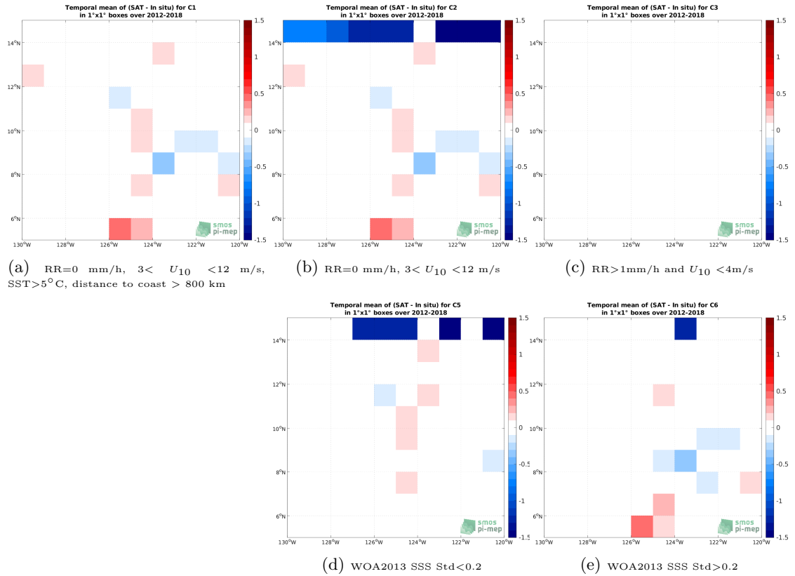
Figure 12: Temporal mean gridded over spatial boxes of size 1^\circ \times 1^\circ of \Delta SSS (SMAP SSS L4 OI v2 - Monthly (IPRC) - TSG (SAMOS)) for 5 different subdatasets corresponding to:RR=0 mm/h, 3 < U_{10} < 12 m/s, SST >5^\circ\text{C} , distance to coast > 800 km (a), RR=0 mm/h, 3 < U_{10} < 12 m/s (b), RR >1 mm/h and U_{10} < 4 m/s (c), WOA2013 SSS Std <0.2 (d), WOA2013 SSS Std >0.2 (e).
