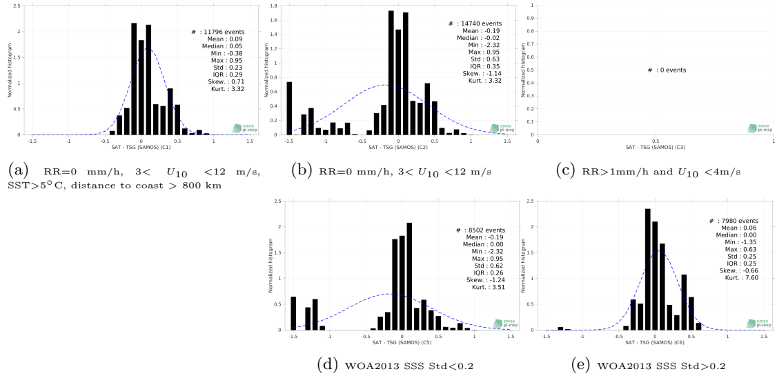
Figure 13: Normalized histogram of \Delta SSS (SMAP SSS L4 OI v2 - Monthly (IPRC) - TSG (SAMOS)) for 5 different subdatasets corresponding to: RR=0 mm/h, 3 < U_{10} < 12 m/s, SST > 5°C, distance to coast > 800 km (a), RR=0 mm/h, 3 < U_{10} < 12 m/s (b), RR > 1mm/h and U_{10} < 4 m/s (c), WOA2013 SSS Std < 0.2 (d), WOA2013 SSS Std > 0.2 (e).
