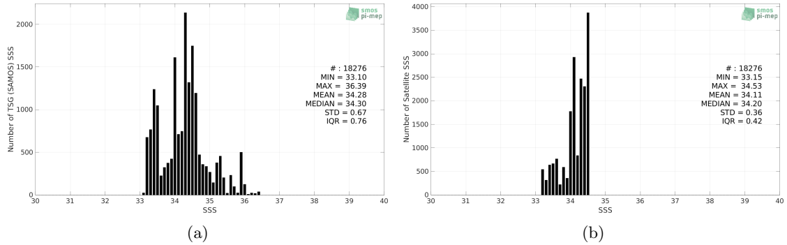
Figure 2: Histograms of SSS from TSG (SAMOS) (a) and SMAP SSS L4 OI v2 - Monthly (IPRC) (b) considering all match-up pairs per bins of 0.1 over the SPURS 2 Pi-MEP region and for the full satellite product period.
