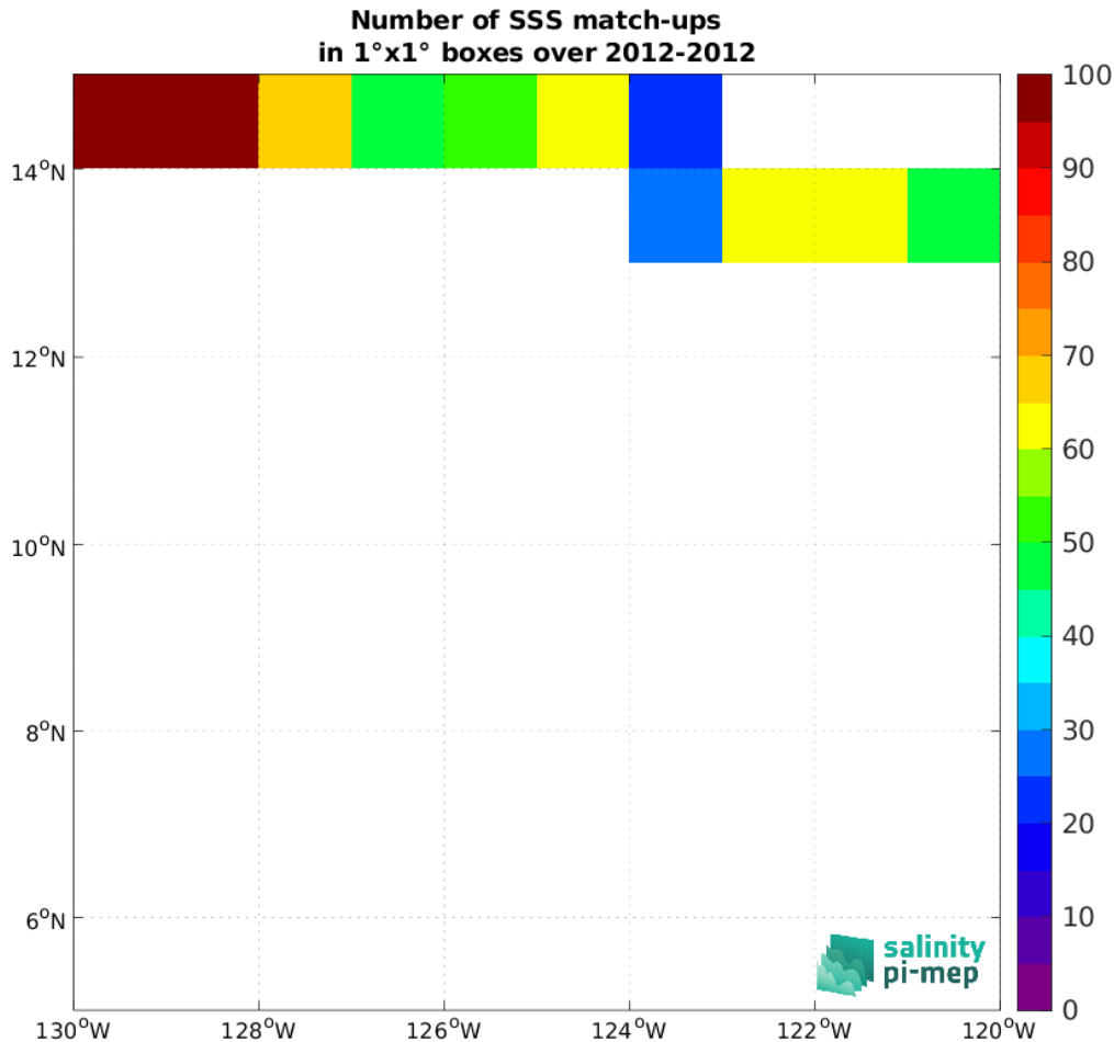
Figure 4: Number of SSS match-ups between TSG (GOSUD-Research-vessel) SSS and the SMAP SSS L4 OI v2 - Monthly (IPRC) SSS product for the SPURS 2 Pi-MEP region over 1^\circ \times 1^\circ boxes and for the full satellite product period.
