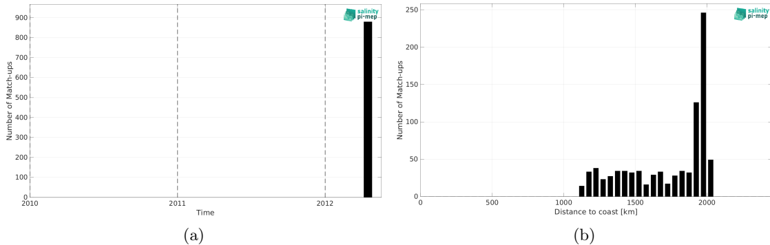
Figure 1: Number of match-ups between TSG (GOSUD-Research-vessel) and SMAP SSS L4 OI v2 - Monthly (IPRC) SSS as a function of time (a) and as function of the distance to coast (b) over the SPURS 2 Pi-MEP region and for the full satellite product period.
