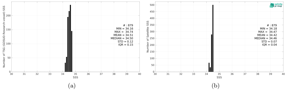
Figure 2: Histograms of SSS from TSG (GOSUD-Research-vessel) (a) and SMAP SSS L4 OI v2 - Monthly (IPRC) (b) considering all match-up pairs per bins of 0.1 over the SPURS 2 Pi-MEP region and for the full satellite product period.
