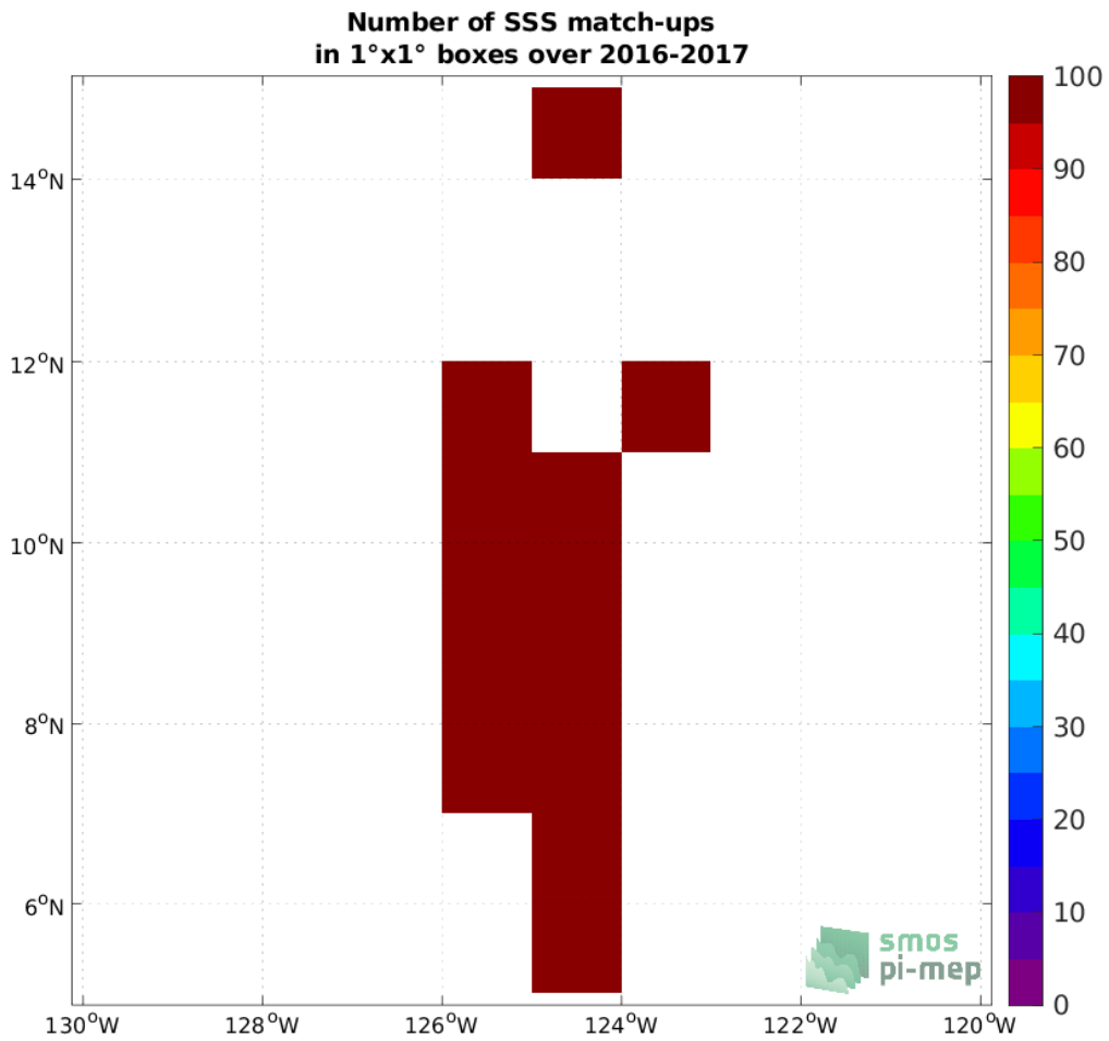
Figure 4: Number of SSS match-ups between Salinity Snake (SPURS 2) SSS and the SMAP SSS L4 OI v2 - Monthly (IPRC) SSS product for the SPURS 2 Pi-MEP region over 1^\circ \times 1^\circ boxes and for the full satellite product period.
