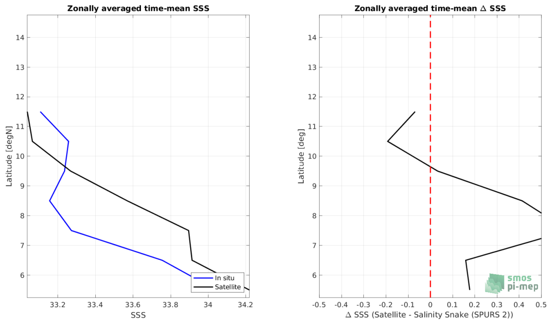
Figure 8: Left panel: Zonal mean SSS from SMAP SSS L4 OI v2 - Monthly (IPRC) satellite product (black) and from Salinity Snake (SPURS 2) (blue). Right panel: Zonal mean of \Delta SSS (Satellite - Salinity Snake (SPURS 2)) for all the collected Pi-MEP match-up pairs estimated over the full satellite product period.
