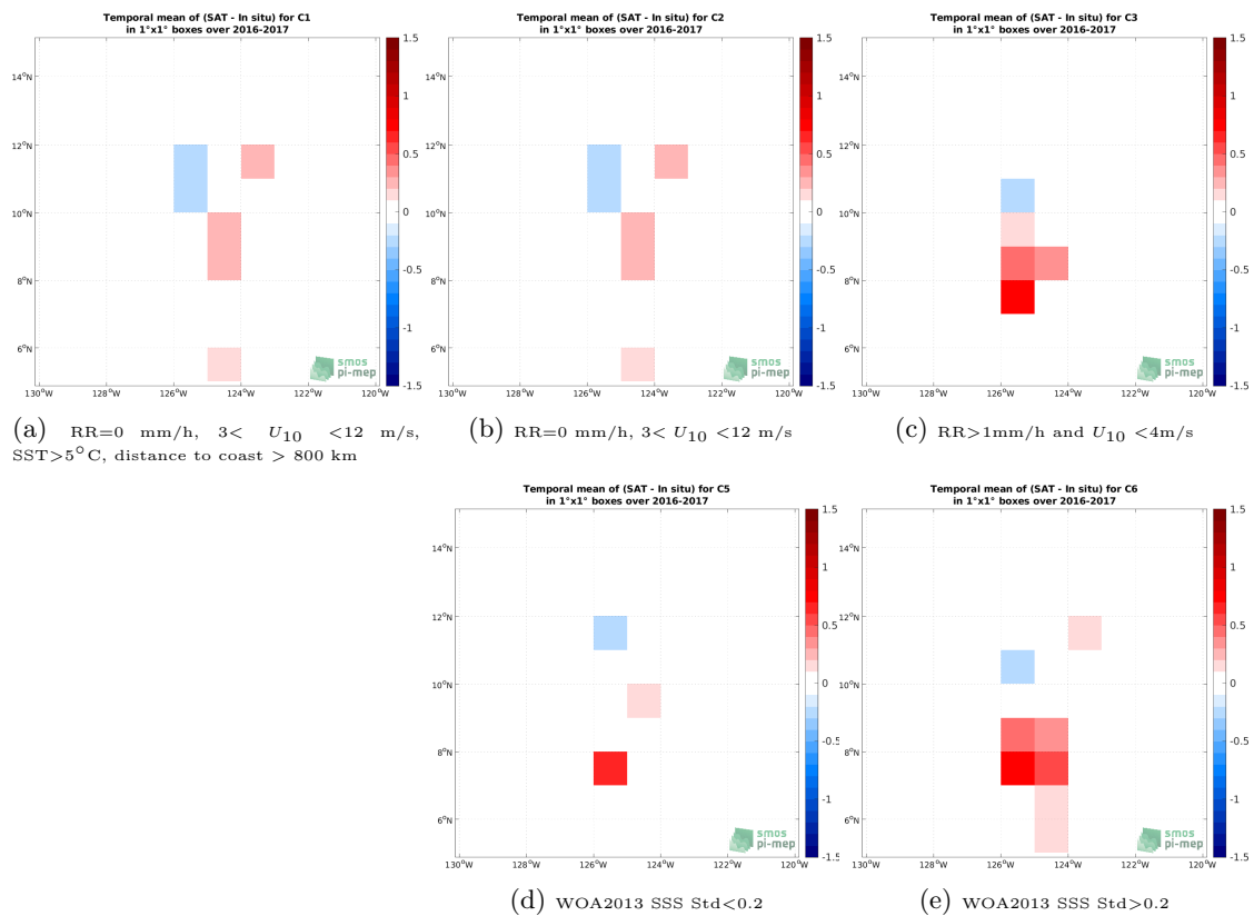
Figure 12: Temporal mean gridded over spatial boxes of size 1^\circ \times 1^\circ of \Delta SSS (SMAP SSS L4 OI v2 - Monthly (IPRC) - Salinity Snake (SPURS 2)) for 5 different subdatasets corresponding to:RR=0 mm/h, 3 < U_{10} < 12 m/s, SST>5°C, distance to coast > 800 km (a), RR=0 mm/h, 3 < U_{10} < 12 m/s (b), RR>1mm/h and U_{10} < 4 m/s (c), WOA2013 SSS Std<0.2 (d), WOA2013 SSS Std>0.2 (e).
