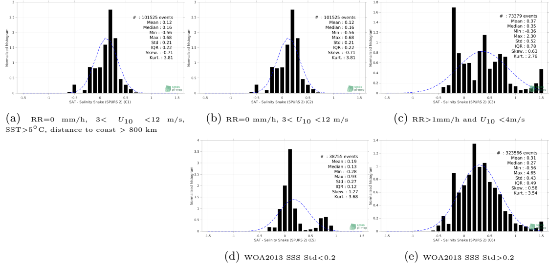
Figure 13: Normalized histogram of \Delta SSS (SMAP SSS L4 OI v2 - Monthly (IPRC) - Salinity Snake (SPURS 2)) for 5 different subdatasets corresponding to: RR=0 mm/h, 3 < U_{10} < 12 m/s, SST > 5°C, distance to coast > 800 km (a), RR=0 mm/h, 3 < U_{10} < 12 m/s (b), RR > 1mm/h and U_{10} < 4 m/s (c), WOA2013 SSS Std < 0.2 (d), WOA2013 SSS Std > 0.2 (e).
