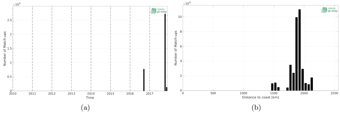
Figure 1: Number of match-ups between Salinity Snake (SPURS 2) and SMAP SSS L4 OI v2 - Monthly (IPRC) SSS as a function of time (a) and as function of the distance to coast (b) over the SPURS 2 Pi-MEP region and for the full satellite product period.
