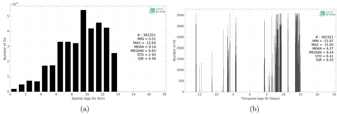
Figure 5: Histograms of the spatial (a) and temporal (b) lags between the location/time of the Salinity Snake (SPURS 2) measurement and the date of the corresponding SMAP SSS L4 OI v2 - Monthly (IPRC) SSS pixel.
