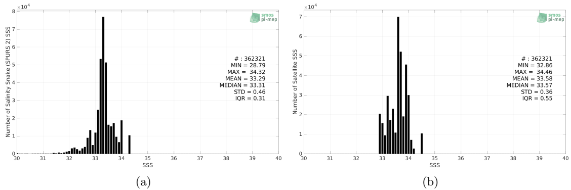
Figure 2: Histograms of SSS from Salinity Snake (SPURS 2) (a) and SMAP SSS L4 OI v2 - Monthly (IPRC) (b) considering all match-up pairs per bins of 0.1 over the SPURS 2 Pi-MEP region and for the full satellite product period.
