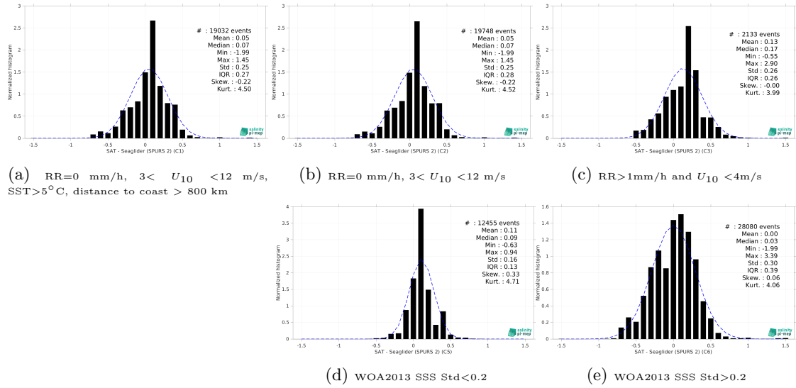
Figure 13: Normalized histogram of \Delta SSS (SMAP SSS L4 OI v2 - Monthly (IPRC) - Seaglider (SPURS 2)) for 5 different subdatasets corresponding to: RR=0 mm/h, 3 < U_{10} < 12 m/s, SST>5°C, distance to coast > 800 km (a), RR=0 mm/h, 3 < U_{10} < 12 m/s (b), RR>1mm/h and U_{10} < 4 m/s (c), WOA2013 SSS Std<0.2 (d), WOA2013 SSS Std>0.2 (e).
