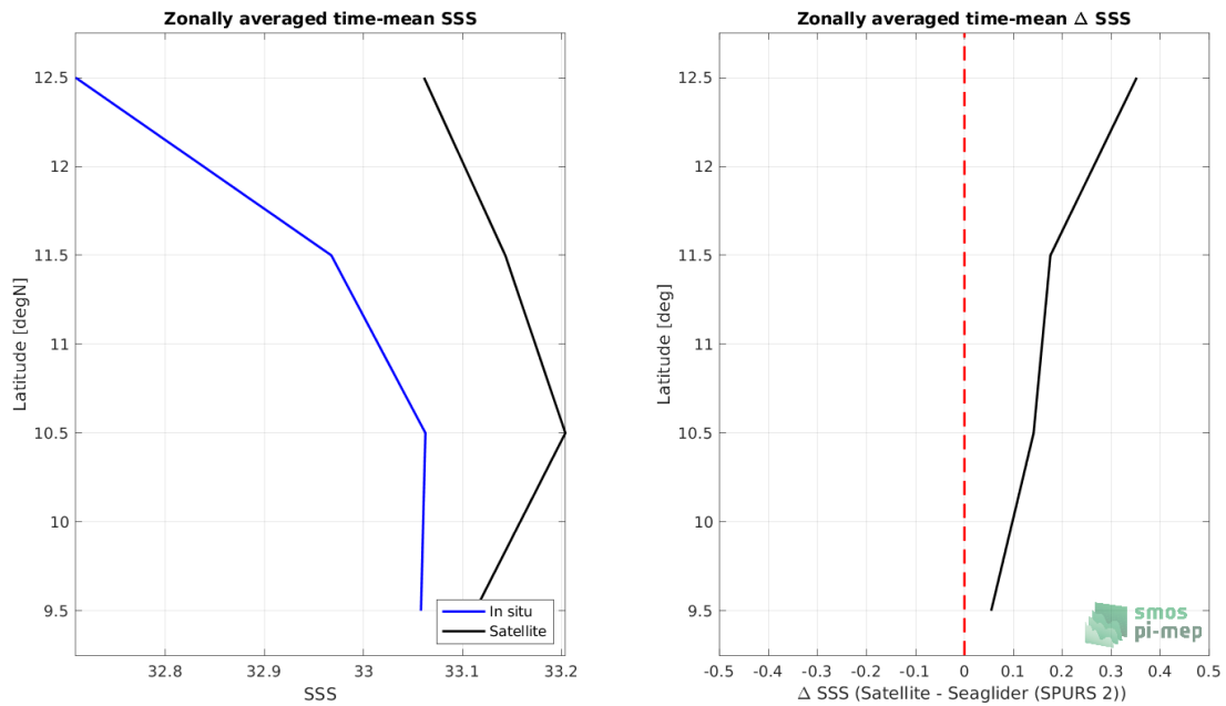
Figure 8: Left panel: Zonal mean SSS from SMAP SSS L4 OI v2 - Monthly (IPRC) satellite product (black) and from Seaglider (SPURS 2) (blue). Right panel: Zonal mean of \Delta SSS (Satellite - Seaglider (SPURS 2)) for all the collected Pi-MEP match-up pairs estimated over the full satellite product period.
