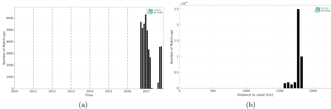
Figure 1: Number of match-ups between Seaglider (SPURS 2) and SMAP SSS L4 OI v2 - Monthly (IPRC) SSS as a function of time (a) and as function of the distance to coast (b) over the SPURS 2 Pi-MEP region and for the full satellite product period.
