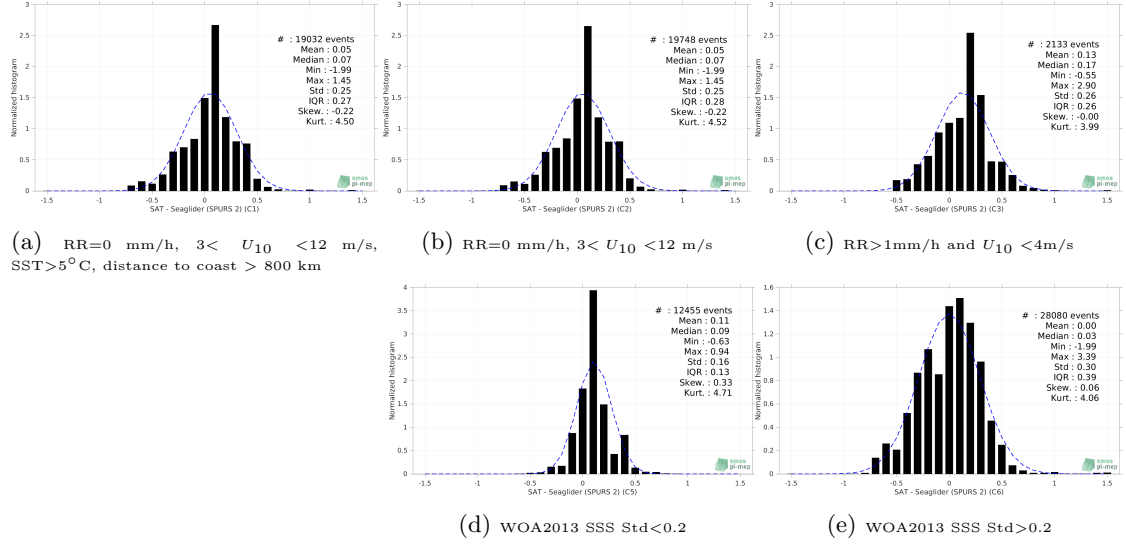
Figure 13: Normalized histogram of \Delta SSS (SMAP SSS L4 OI v2 - Monthly (IPRC) - Seaglider (SPURS 2)) for 5 different subdatasets corresponding to: RR=0 mm/h, 3 < U_{10} < 12 m/s, SST>5°C, distance to coast > 800 km (a), RR=0 mm/h, 3 < U_{10} < 12 m/s (b), RR>1mm/h and U_{10} < 4 m/s (c), WOA2013 SSS Std<0.2 (d), WOA2013 SSS Std>0.2 (e).
