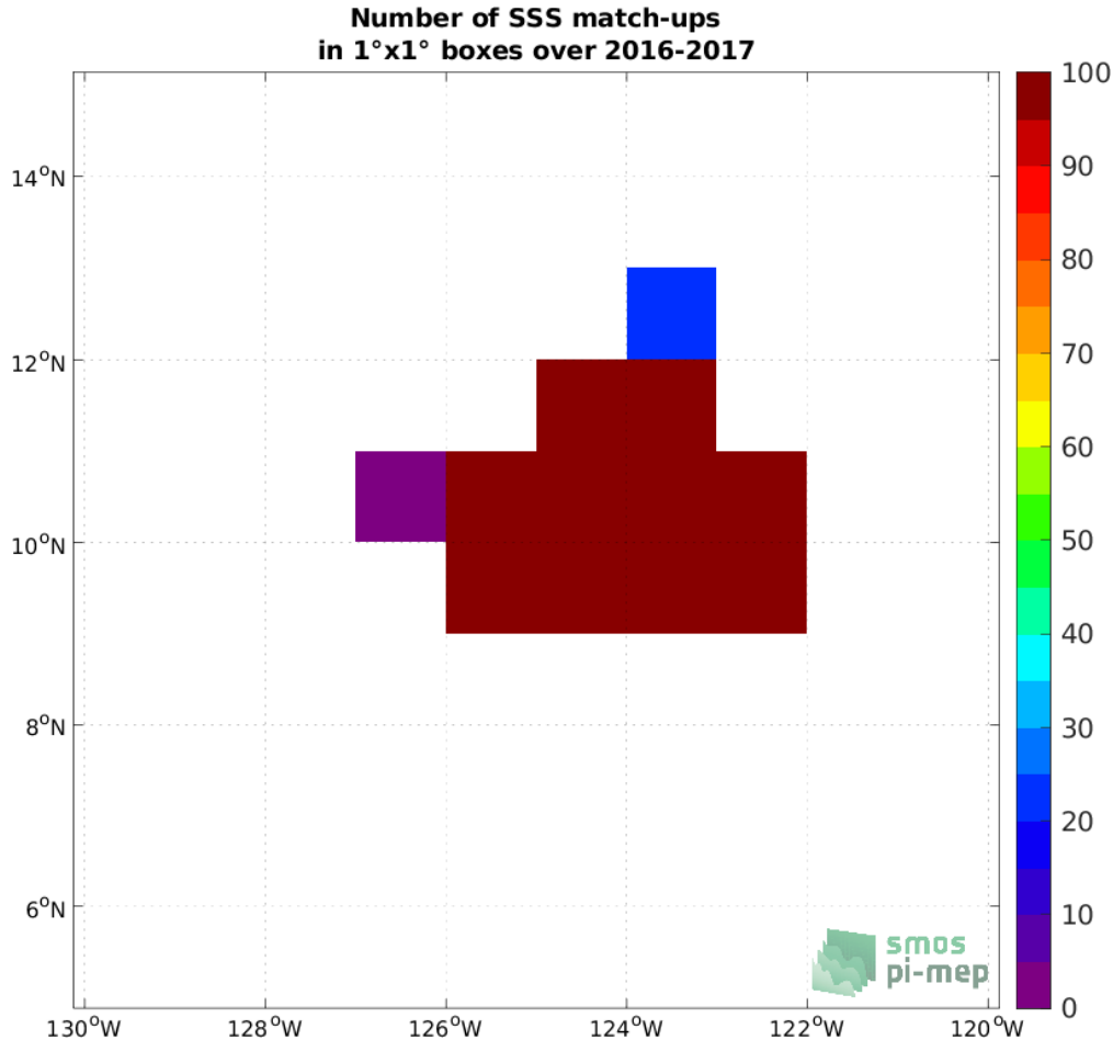
Figure 4: Number of SSS match-ups between Seagliders (SPURS 2) SSS and the SMAP SSS L4 OI v2 - Monthly (IPRC) SSS product for the SPURS 2 Pi-MEP region over 1^\circ \times 1^\circ boxes and for the full satellite product period.
