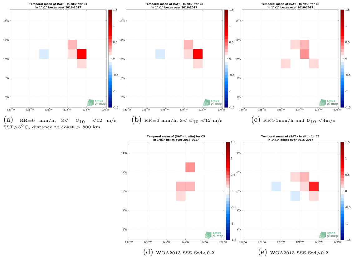
Figure 12: Temporal mean gridded over spatial boxes of size 1^\circ \times 1^\circ of \Delta SSS (SMAP SSS L4 OI v2 - Monthly (IPRC) - Seaglider (SPURS 2)) for 5 different subdatasets corresponding to:RR=0 mm/h, 3 < U_{10} < 12 m/s, SST >5^\circ\text{C} , distance to coast > 800 km (a), RR=0 mm/h, 3 < U_{10} < 12 m/s (b), RR >1 mm/h and U_{10} < 4 m/s (c), WOA2013 SSS Std <0.2 (d), WOA2013 SSS Std >0.2 (e).
