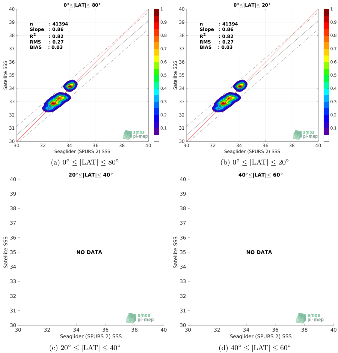
Figure 9: Contour maps of the concentration of SMAP SSS L4 OI v2 - Monthly (IPRC) SSS (y-axis) versus Seaglider (SPURS 2) SSS (x-axis) at match-up pairs for different latitude bands. For each plot, the red line shows x=y . The black thin and dashed lines indicate a linear fit through the data cloud and the \pm 95\% confidence levels, respectively. The number match-up pairs n , the slope and R^2 coefficient of the linear fit, the root mean square (RMS) and the mean bias between satellite and in situ data are indicated for each latitude band in each plots.
