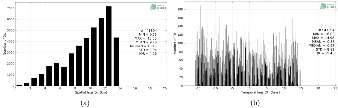
Figure 5: Histograms of the spatial (a) and temporal (b) lags between the location/time of the Seaglider (SPURS 2) measurement and the date of the corresponding SMAP SSS L4 OI v2 - Monthly (IPRC) SSS pixel.
