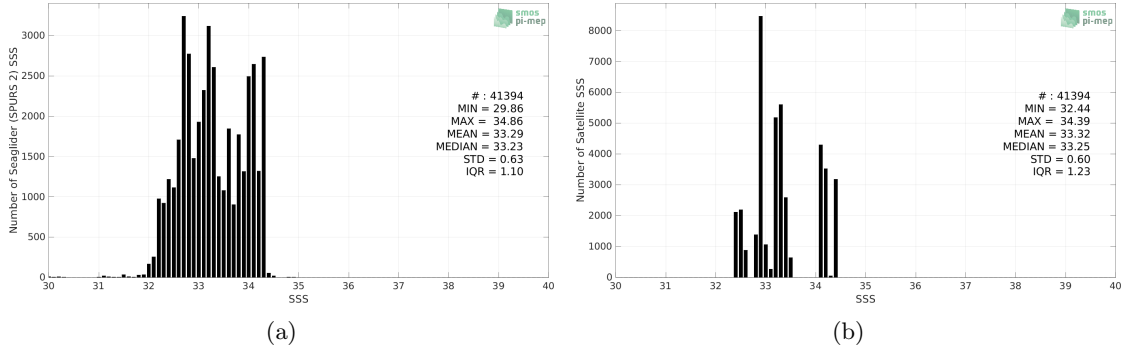
Figure 2: Histograms of SSS from Seaglider (SPURS 2) (a) and SMAP SSS L4 OI v2 - Monthly (IPRC) (b) considering all match-up pairs per bins of 0.1 over the SPURS 2 Pi-MEP region and for the full satellite product period.
