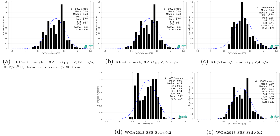
Figure 13: Normalized histogram of \Delta SSS (SMAP SSS L4 OI v2 - Monthly (IPRC) - Saildrone) for 5 different subdatasets corresponding to: RR=0 mm/h, 3 < U_{10} < 12 m/s, SST>5°C, distance to coast > 800 km (a), RR=0 mm/h, 3 < U_{10} < 12 m/s (b), RR>1mm/h and U_{10} < 4 m/s (c), WOA2013 SSS Std<0.2 (d), WOA2013 SSS Std>0.2 (e).
