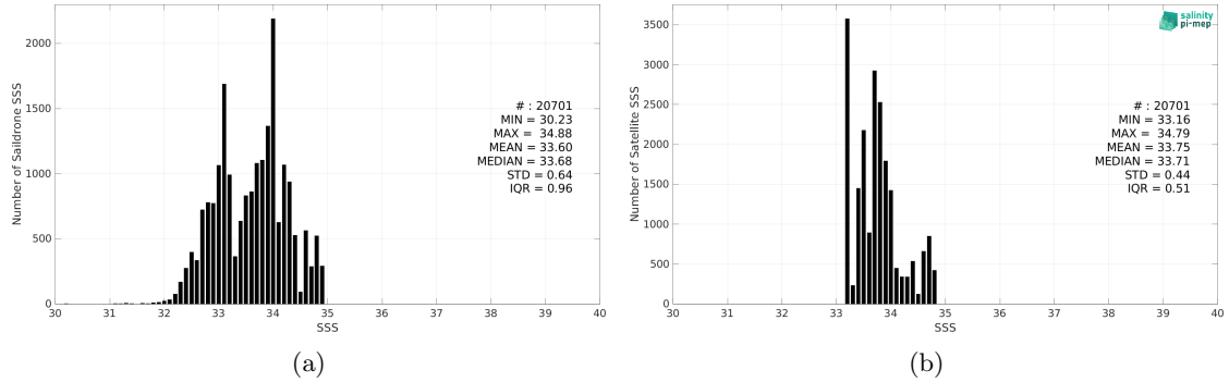
Figure 2: Histograms of SSS from Saildrone (a) and SMAP SSS L4 OI v2 - Monthly (IPRC) (b) considering all match-up pairs per bins of 0.1 over the SPURS 2 Pi-MEP region and for the full satellite product period.
