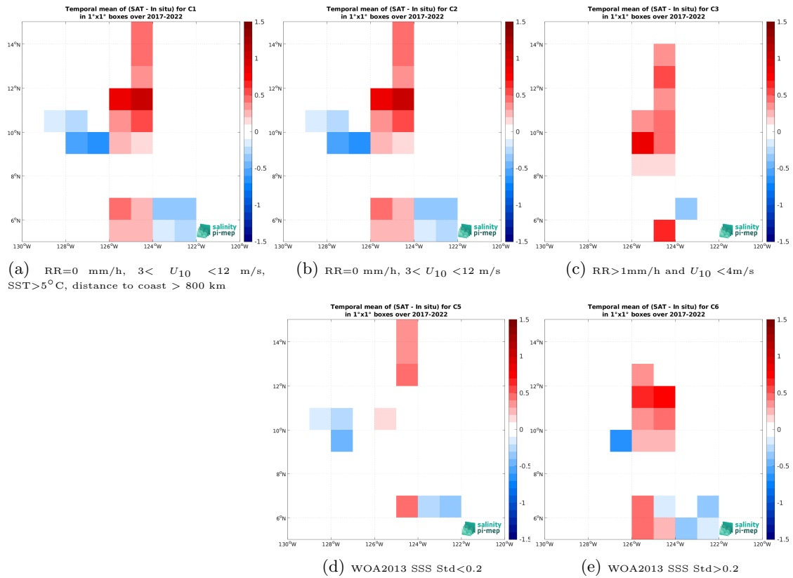
Figure 12: Temporal mean gridded over spatial boxes of size 1^\circ \times 1^\circ of \Delta SSS (SMAP SSS L4 OI v2 - Monthly (IPRC) - Sailydrone) for 5 different subdatasets corresponding to:RR=0 mm/h, 3 < U_{10} < 12 m/s, SST >5^\circ\text{C} , distance to coast > 800 km (a), RR=0 mm/h, 3 < U_{10} < 12 m/s (b), RR >1 mm/h and U_{10} < 4 m/s (c), WOA2013 SSS Std <0.2 (d), WOA2013 SSS Std >0.2 (e).
