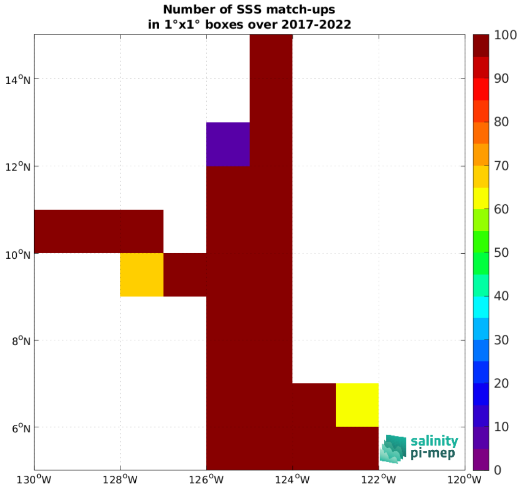
Figure 4: Number of SSS match-ups between Saildrone SSS and the SMAP SSS L4 OI v2 - Monthly (IPRC) SSS product for the SPURS 2 Pi-MEP region over 1^\circ \times 1^\circ boxes and for the full satellite product period.
