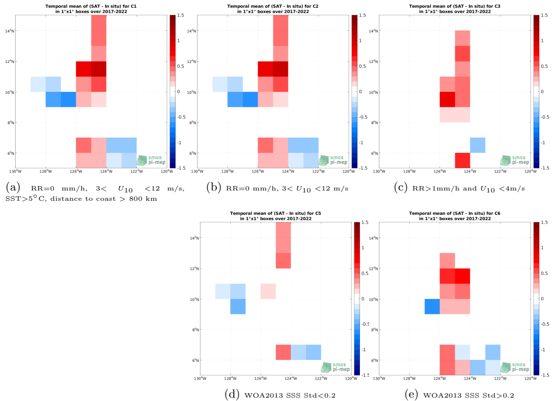
Figure 12: Temporal mean gridded over spatial boxes of size 1^\circ \times 1^\circ of \Delta SSS (SMAP SSS L4 OI v2 - Monthly (IPRC) - Saildrone) for 5 different subdatasets corresponding to:RR=0 mm/h, 3 < U_{10} < 12 m/s, SST >5^\circ\text{C} , distance to coast > 800 km (a), RR=0 mm/h, 3 < U_{10} < 12 m/s (b), RR >1 mm/h and U_{10} < 4 m/s (c), WOA2013 SSS Std <0.2 (d), WOA2013 SSS Std >0.2 (e).
