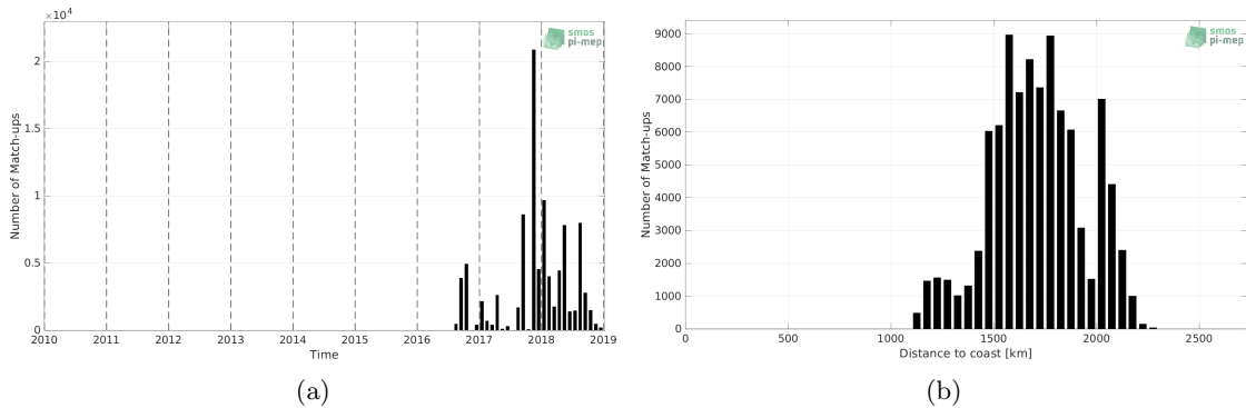
Figure 1: Number of match-ups between Surface drifters and SMAP SSS L4 OI v2 - Monthly (IPRC) SSS as a function of time (a) and as function of the distance to coast (b) over the SPURS 2 Pi-MEP region and for the full satellite product period.
