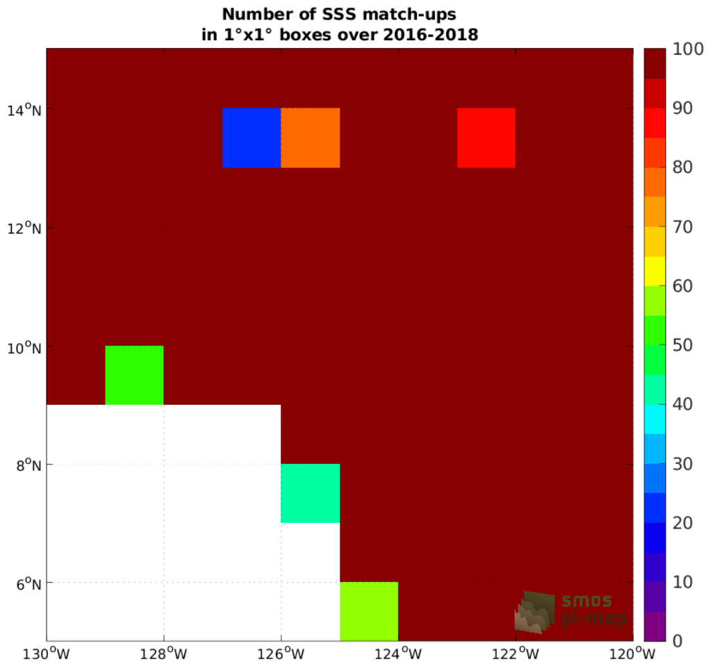
Figure 3: Number of SSS match-ups between Surface drifters SSS and the SMAP SSS L4 OI v2 - Monthly (IPRC) SSS product for the SPURS 2 Pi-MEP region over 1°x1° boxes and for the full satellite product period.
