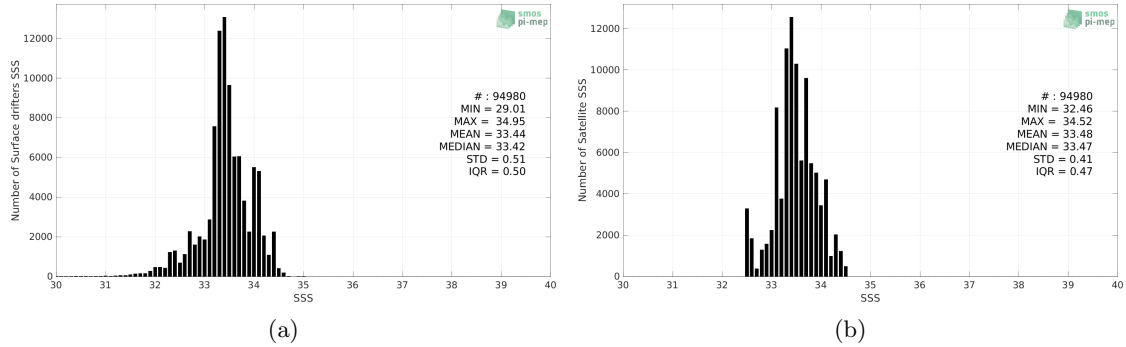
Figure 2: Histograms of SSS from Surface drifters (a) and SMAP SSS L4 OI v2 - Monthly (IPRC) (b) considering all match-up pairs per bins of 0.1 over the SPURS 2 Pi-MEP region and for the full satellite product period.
