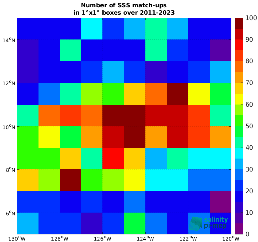
Figure 4: Number of SSS match-ups between Argo SSS and the SMAP SSS L4 OI v2 - Monthly (IPRC) SSS product for the SPURS 2 Pi-MEP region over 1^\circ \times 1^\circ boxes and for the full satellite product period.
