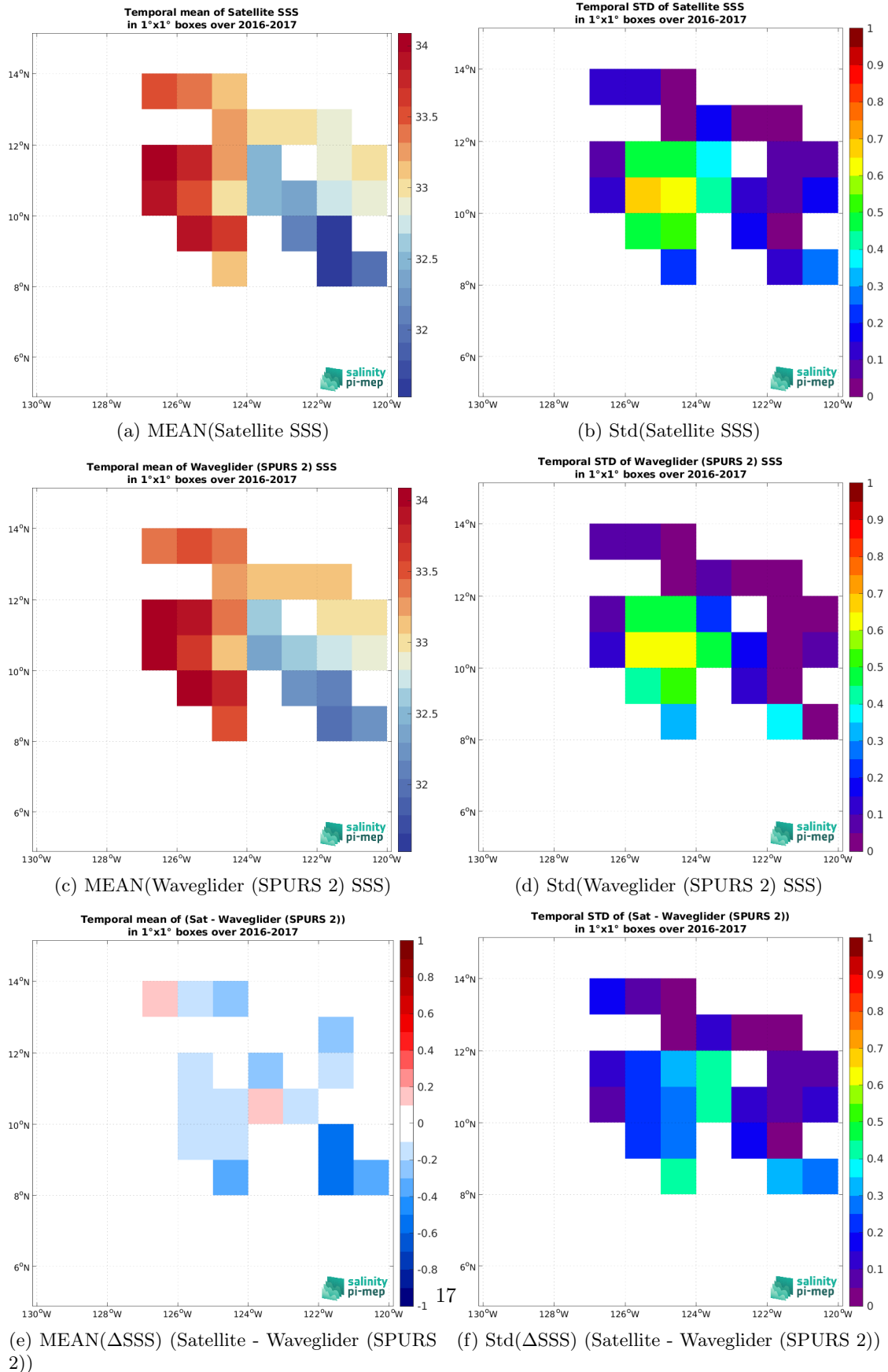
Figure 7: Temporal mean (left) and Std (right) of SSS from SMAP SSS L3 v6 - 8-Day running (RSS) (top), Waveglider (SPURS 2) (middle), and of \Delta SSS (Satellite - Waveglider (SPURS 2)). Only match-up pairs are used to generate these maps.
