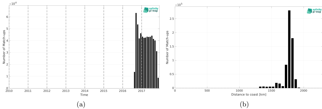
Figure 2: Number of match-ups between Waveglider (SPURS 2) and SMAP SSS L3 v6 - 8-Day running (RSS) SSS as a function of time (a) and as function of the distance to coast (b) over the SPURS 2 Pi-MEP region and for the full satellite product period.
