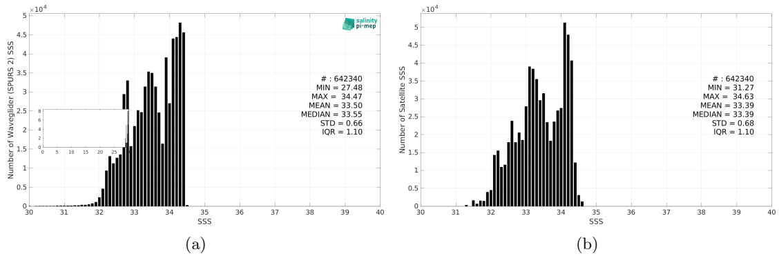
Figure 3: Histograms of SSS from Waveglider (SPURS 2) (a) and SMAP SSS L3 v6 - 8-Day running (RSS) (b) considering all match-up pairs per bins of 0.1 over the SPURS 2 Pi-MEP region and for the full satellite product period.
