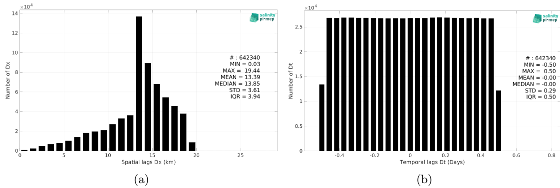
Figure 6: Histograms of the spatial (a) and temporal (b) lags between the location/time of the Waveglider (SPURS 2) measurement and the date of the corresponding SMAP SSS L3 v6 - 8-Day running (RSS) SSS pixel.
