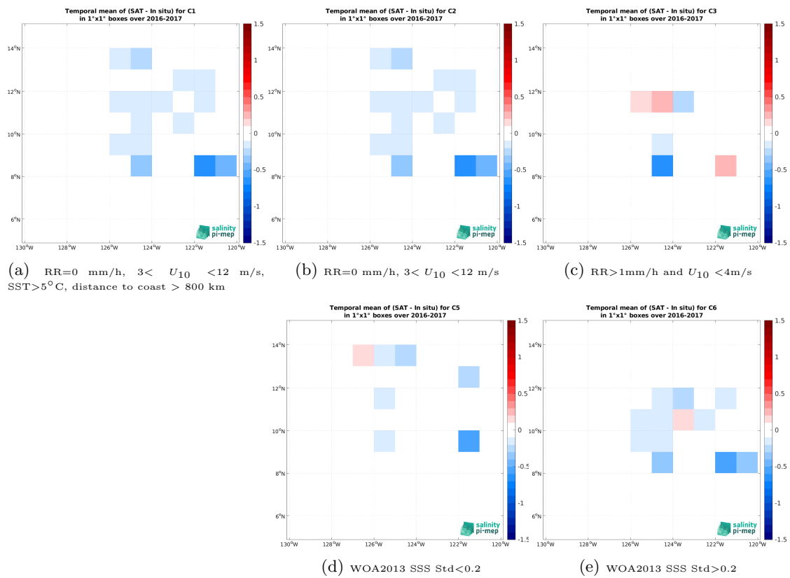
Figure 14: Temporal mean gridded over spatial boxes of size 1^\circ \times 1^\circ of \Delta SSS (SMAP SSS L3 v6 - 8-Day running (RSS) - Waveglider (SPURS 2)) for 5 different subdatasets corresponding to:RR=0 mm/h, 3 < U_{10} < 12 m/s, SST >5^\circ C, distance to coast > 800 km (a), RR=0 mm/h, 3 < U_{10} < 12 m/s (b), RR >1 mm/h and U_{10} < 4 m/s (c), WOA2013 SSS Std <0.2 (d), WOA2013 SSS Std >0.2 (e).
