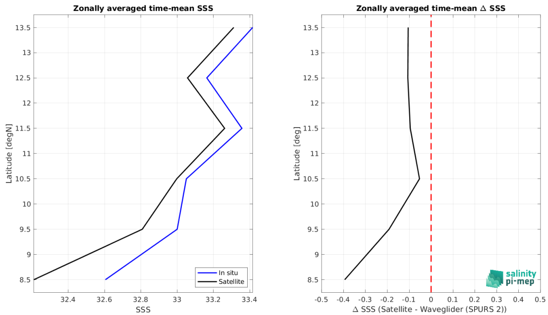
Figure 9: Left panel: Zonal mean SSS from SMAP SSS L3 v6 - 8-Day running (RSS) satellite product (black) and from Waveglider (SPURS 2) (blue). Right panel: Zonal mean of \Delta SSS (Satellite - Waveglider (SPURS 2)) for all the collected Pi-MEP match-up pairs estimated over the full satellite product period.
