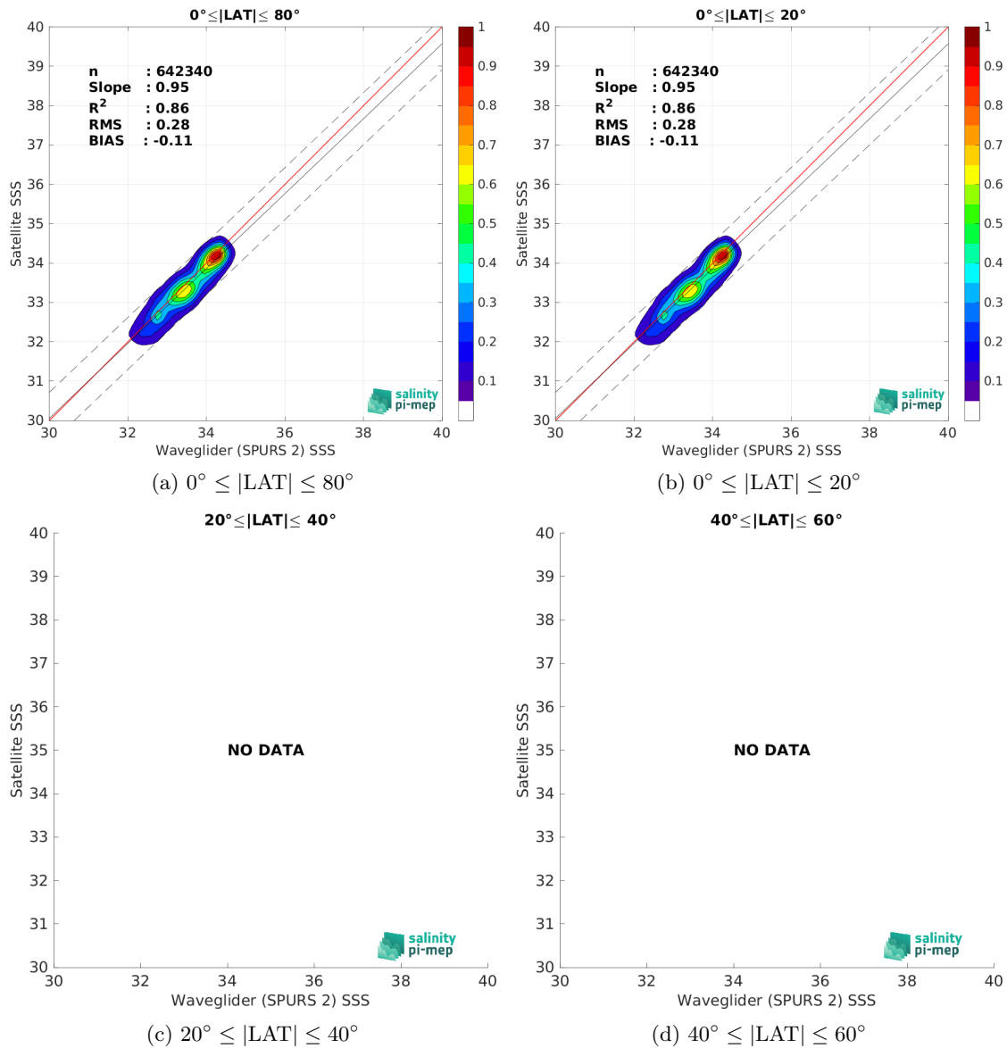
Figure 10: Contour maps of the concentration of SMAP SSS L3 v6 - 8-Day running (RSS) SSS (y-axis) versus Waveglider (SPURS 2) SSS (x-axis) at match-up pairs for different latitude bands. For each plot, the red line shows x=y . The black thin and dashed lines indicate a linear fit through the data cloud and the \pm 95\% confidence levels, respectively. The number match-up pairs n , the slope and R^2 coefficient of the linear fit, the root mean square (RMS) and the mean bias between satellite and in situ data are indicated for each latitude band in each plots.
