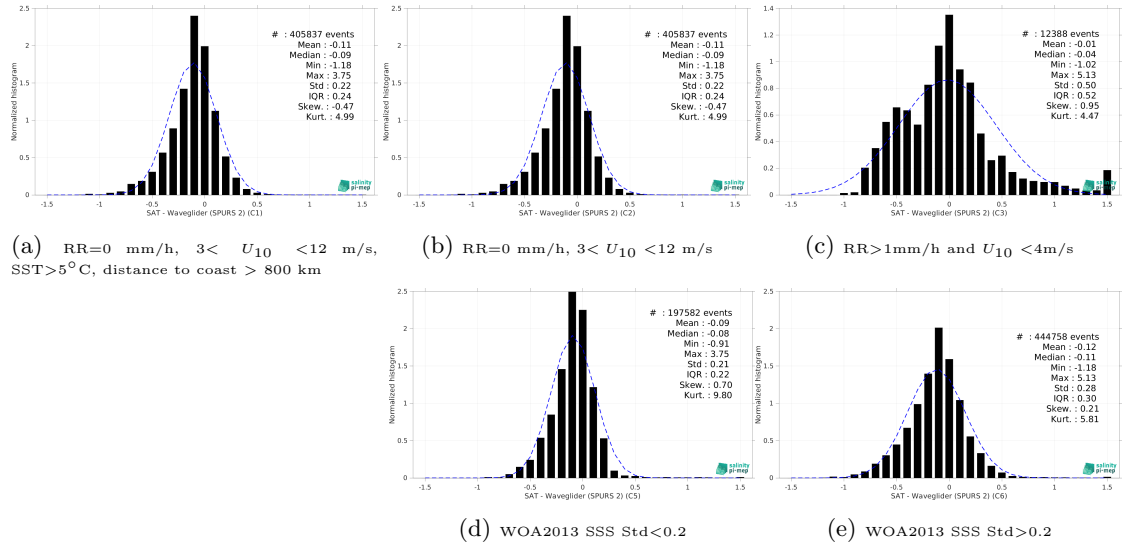
Figure 15: Normalized histogram of \Delta\text{SSS} (SMAP SSS L3 v6 - 8-Day running (RSS) - Waveglider (SPURS 2)) for 5 different subdatasets corresponding to: RR=0 mm/h, 3 < U_{10} < 12 m/s, SST>5°C, distance to coast > 800 km (a), RR=0 mm/h, 3 < U_{10} < 12 m/s (b), RR>1mm/h and U_{10} < 4 m/s (c), WOA2013 SSS Std<0.2 (d), WOA2013 SSS Std>0.2 (e).
