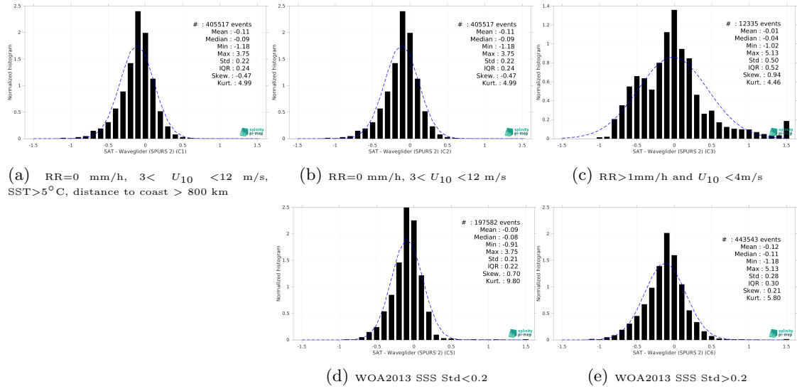
Figure 15: Normalized histogram of \Delta SSS (SMAP SSS L3 v6 - 8-Day running (RSS) - Waveglider (SPURS 2)) for 5 different subdatasets corresponding to: RR=0 mm/h, 3 < U_{10} < 12 m/s, SST>5°C, distance to coast > 800 km (a), RR=0 mm/h, 3 < U_{10} < 12 m/s (b), RR>1mm/h and U_{10} < 4 m/s (c), WOA2013 SSS Std<0.2 (d), WOA2013 SSS Std>0.2 (e).
