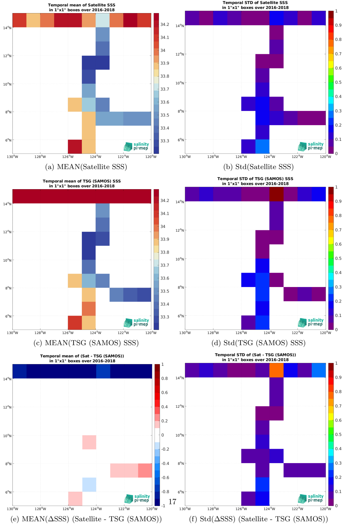
Figure 7: Temporal mean (left) and Std (right) of SSS from SMAP SSS L3 v6 - 8-Day running (RSS) (top), TSG (SAMOS) (middle), and of \Delta SSS (Satellite - TSG (SAMOS)). Only match-up pairs are used to generate these maps.
