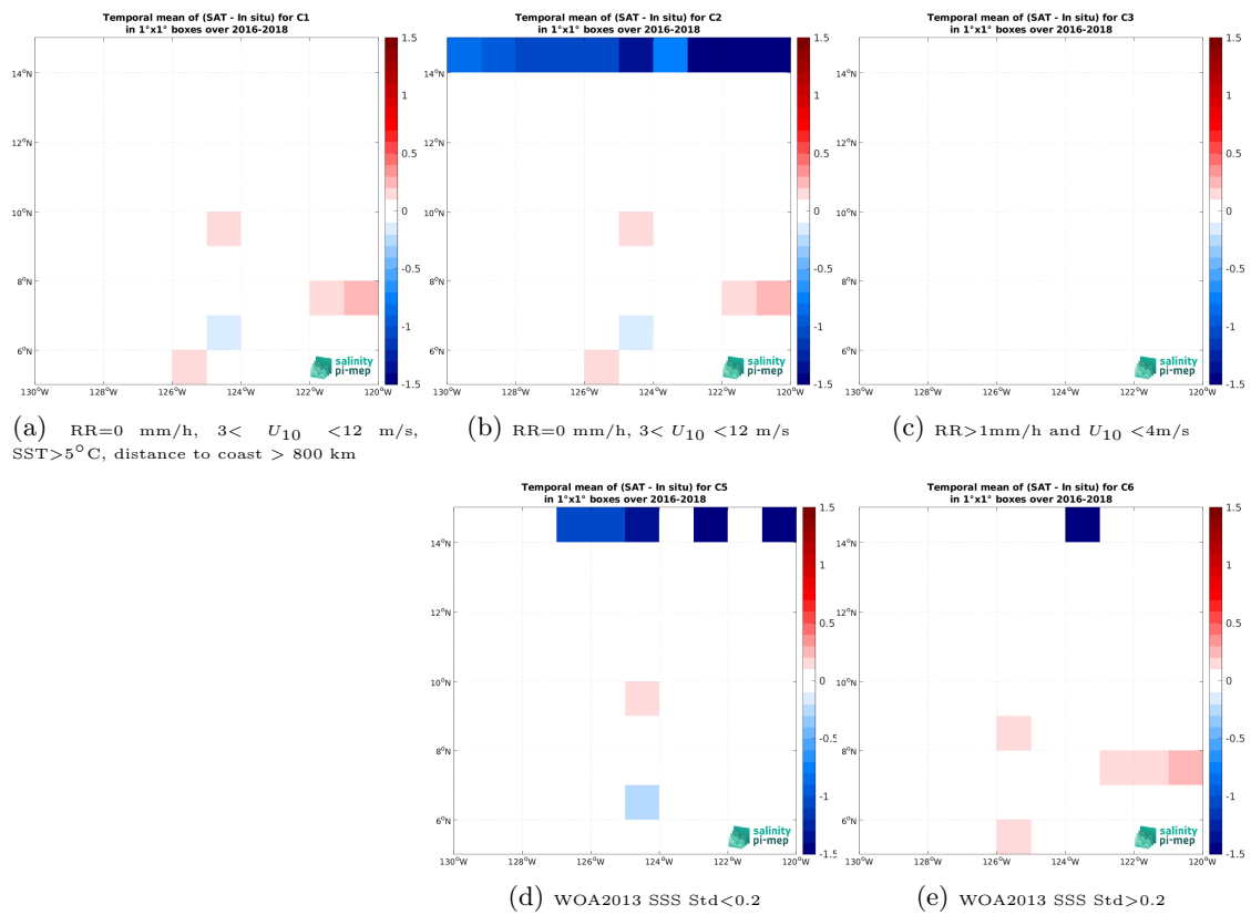
Figure 14: Temporal mean gridded over spatial boxes of size 1^\circ \times 1^\circ of \Delta\text{SSS} (SMAP SSS L3 v6 - 8-Day running (RSS) - TSG (SAMOS)) for 5 different subdatasets corresponding to:RR=0 mm/h, 3 < U_{10} < 12 m/s, SST>5°C, distance to coast > 800 km (a), RR=0 mm/h, 3 < U_{10} < 12 m/s (b), RR>1mm/h and U_{10} < 4 m/s (c), WOA2013 SSS Std<0.2 (d), WOA2013 SSS Std>0.2 (e).
