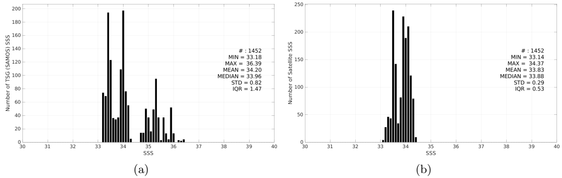
Figure 3: Histograms of SSS from TSG (SAMOS) (a) and SMAP SSS L3 v6 - 8-Day running (RSS) (b) considering all match-up pairs per bins of 0.1 over the SPURS 2 Pi-MEP region and for the full satellite product period.
