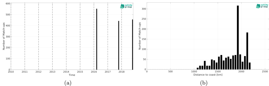
Figure 2: Number of match-ups between TSG (SAMOS) and SMAP SSS L3 v6 - 8-Day running (RSS) SSS as a function of time (a) and as function of the distance to coast (b) over the SPURS 2 Pi-MEP region and for the full satellite product period.
