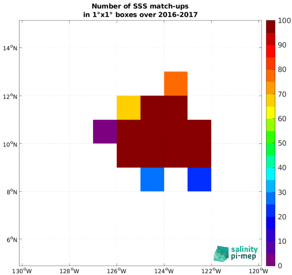
Figure 5: Number of SSS match-ups between Seagliders (SPURS 2) SSS and the SMAP SSS L3 v6 - 8-Day running (RSS) SSS product for the SPURS 2 Pi-MEP region over 1°x1° boxes and for the full satellite product period.
