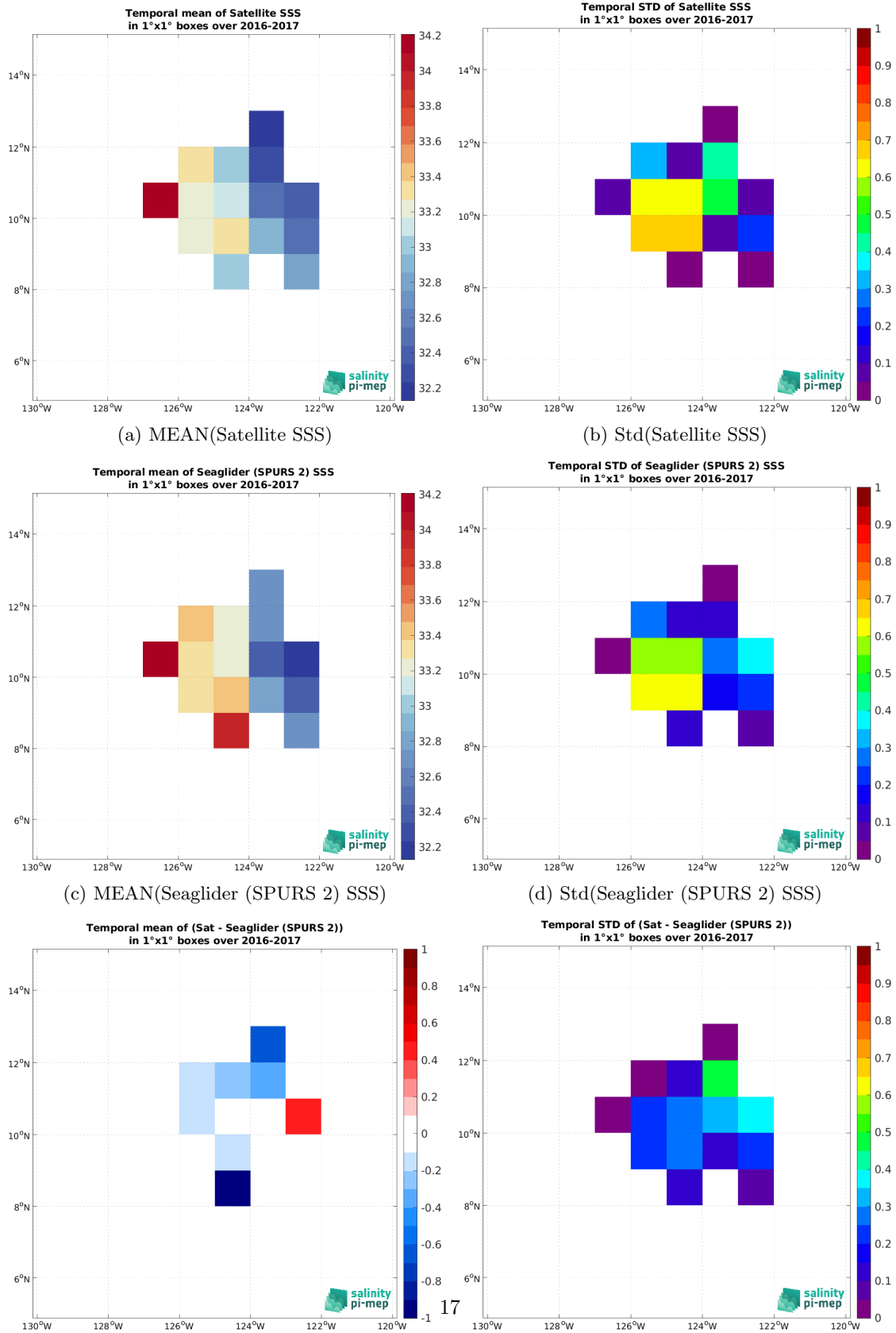
Figure 7: Temporal mean (left) and Std (right) of SSS from SMAP SSS L3 v6 - 8-Day running (RSS) (top), Seaglider (SPURS 2) (middle), and of \Delta SSS (Satellite - Seaglider (SPURS 2)). Only match-up pairs are used to generate these maps.
