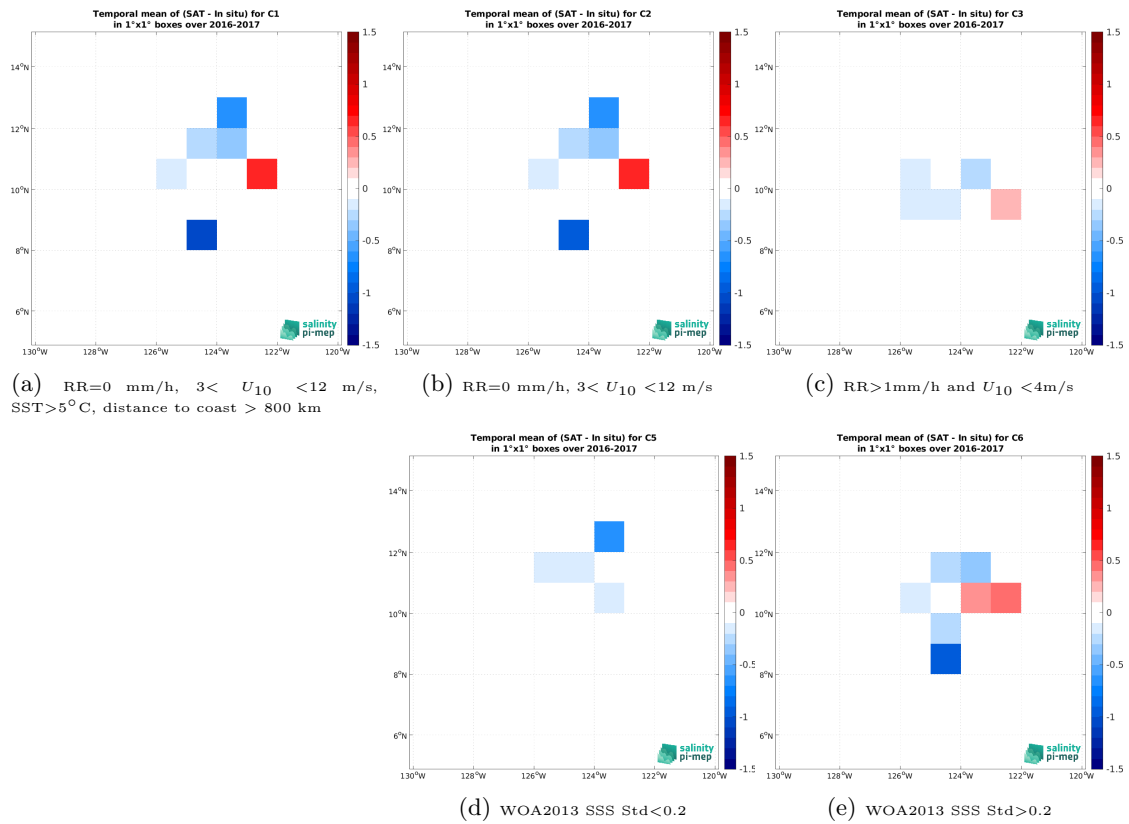
Figure 14: Temporal mean gridded over spatial boxes of size 1^\circ \times 1^\circ of \Delta SSS (SMAP SSS L3 v6 - 8-Day running (RSS) - Seaglider (SPURS 2)) for 5 different subdatasets corresponding to:RR=0 mm/h, 3 < U_{10} < 12 m/s, SST >5^\circ\text{C} , distance to coast > 800 km (a), RR=0 mm/h, 3 < U_{10} < 12 m/s (b), RR >1 mm/h and U_{10} < 4 m/s (c), WOA2013 SSS Std <0.2 (d), WOA2013 SSS Std >0.2 (e).
