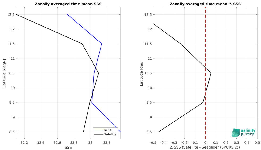
Figure 9: Left panel: Zonal mean SSS from SMAP SSS L3 v6 - 8-Day running (RSS) satellite product (black) and from Seaglider (SPURS 2) (blue). Right panel: Zonal mean of \Delta SSS (Satellite - Seaglider (SPURS 2)) for all the collected Pi-MEP match-up pairs estimated over the full satellite product period.
