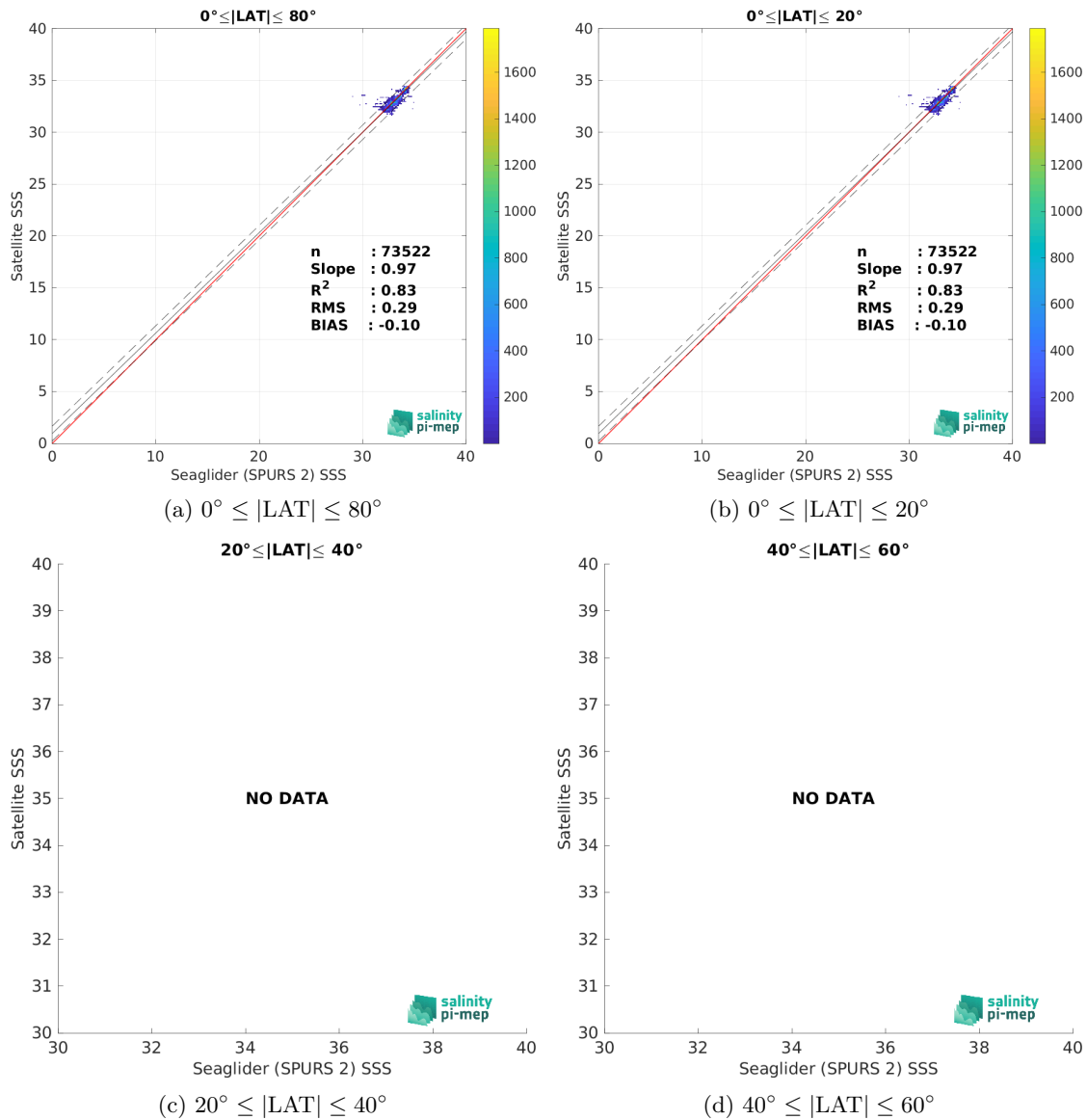
Figure 10: Contour maps of the concentration of SMAP SSS L3 v6 - 8-Day running (RSS) SSS (y-axis) versus Seaglider (SPURS 2) SSS (x-axis) at match-up pairs for different latitude bands. For each plot, the red line shows x=y . The black thin and dashed lines indicate a linear fit through the data cloud and the \pm 95\% confidence levels, respectively. The number match-up pairs n , the slope and R^2 coefficient of the linear fit, the root mean square (RMS) and the mean bias between satellite and in situ data are indicated for each latitude band in each plots.
