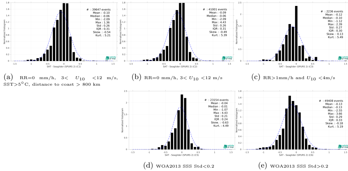
Figure 15: Normalized histogram of \Delta SSS (SMAP SSS L3 v6 - 8-Day running (RSS) - Seaglider (SPURS 2)) for 5 different subdatasets corresponding to: RR=0 mm/h, 3 < U_{10} < 12 m/s, SST > 5°C, distance to coast > 800 km (a), RR=0 mm/h, 3 < U_{10} < 12 m/s (b), RR > 1mm/h and U_{10} < 4 m/s (c), WOA2013 SSS Std < 0.2 (d), WOA2013 SSS Std > 0.2 (e).
