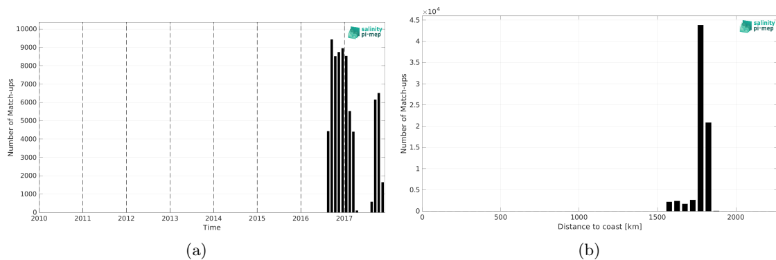
Figure 2: Number of match-ups between Seaglider (SPURS 2) and SMAP SSS L3 v6 - 8-Day running (RSS) SSS as a function of time (a) and as function of the distance to coast (b) over the SPURS 2 Pi-MEP region and for the full satellite product period.
