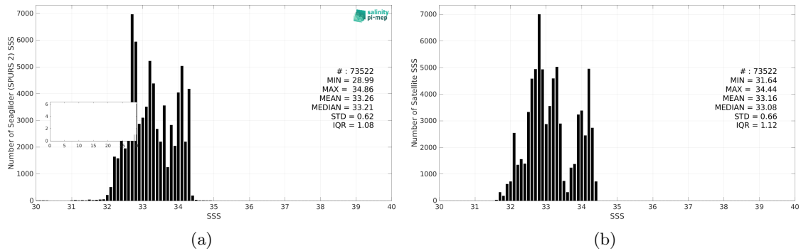
Figure 3: Histograms of SSS from Seaglider (SPURS 2) (a) and SMAP SSS L3 v6 - 8-Day running (RSS) (b) considering all match-up pairs per bins of 0.1 over the SPURS 2 Pi-MEP region and for the full satellite product period.
