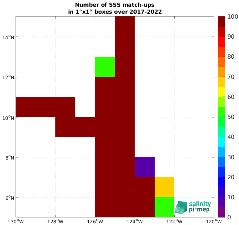
Figure 5: Number of SSS match-ups between Saildrone SSS and the SMAP SSS L3 v6 - 8-Day running (RSS) SSS product for the SPURS 2 Pi-MEP region over 1^\circ \times 1^\circ boxes and for the full satellite product period.
