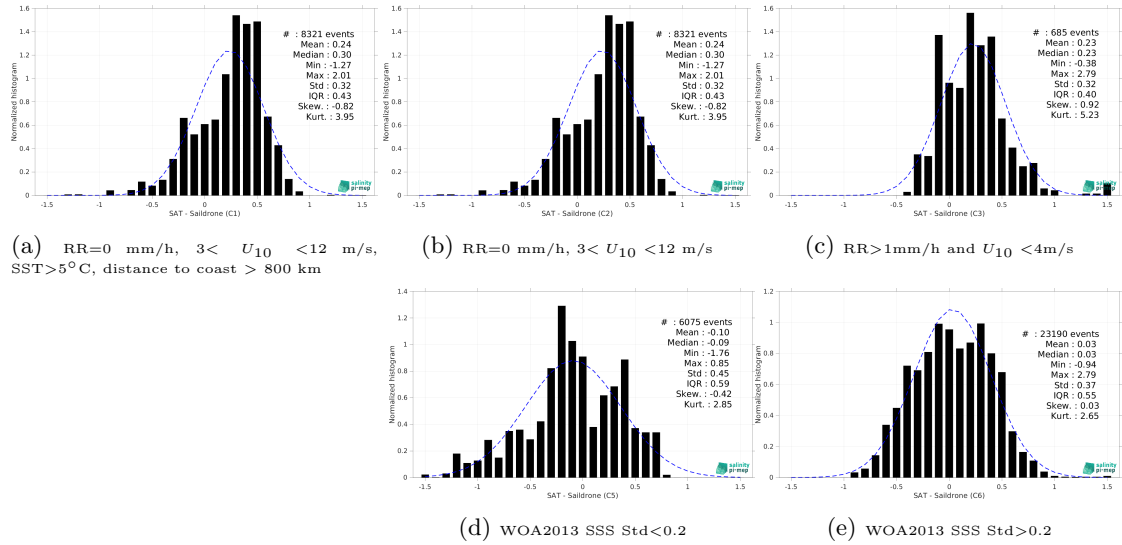
Figure 15: Normalized histogram of \Delta SSS (SMAP SSS L3 v6 - 8-Day running (RSS) - Sairdrone) for 5 different subdatasets corresponding to: RR=0 mm/h, 3 < U_{10} < 12 m/s, SST>5°C, distance to coast > 800 km (a), RR=0 mm/h, 3 < U_{10} < 12 m/s (b), RR>1mm/h and U_{10} < 4 m/s (c), WOA2013 SSS Std<0.2 (d), WOA2013 SSS Std>0.2 (e).
