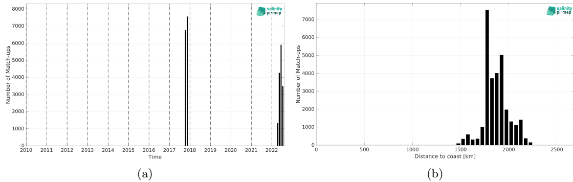
Figure 2: Number of match-ups between Saildrone and SMAP SSS L3 v6 - 8-Day running (RSS) SSS as a function of time (a) and as function of the distance to coast (b) over the SPURS 2 Pi-MEP region and for the full satellite product period.
