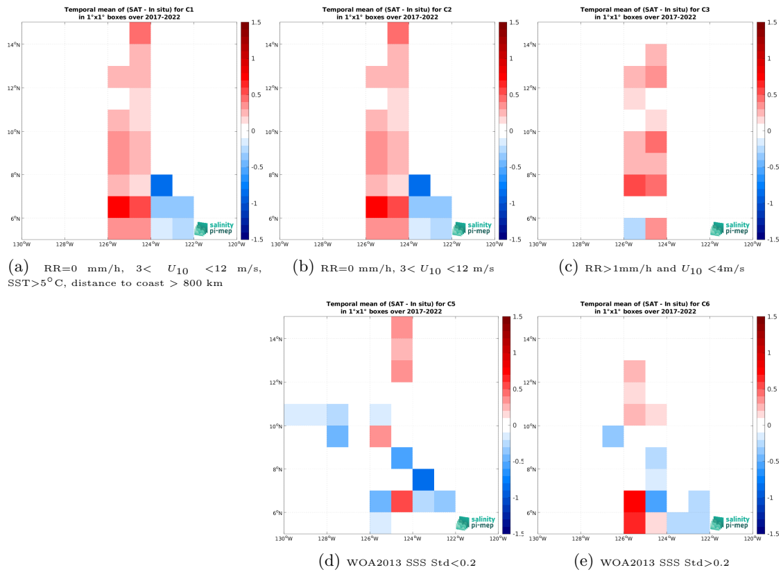
Figure 14: Temporal mean gridded over spatial boxes of size 1^\circ \times 1^\circ of \Delta\text{SSS} (SMAP SSS L3 v6 - 8-Day running (RSS) - Saildrone) for 5 different subdatasets corresponding to:RR=0 mm/h, 3 < U_{10} < 12 m/s, SST>5°C, distance to coast > 800 km (a), RR=0 mm/h, 3 < U_{10} < 12 m/s (b), RR>1mm/h and U_{10} < 4 m/s (c), WOA2013 SSS Std<0.2 (d), WOA2013 SSS Std>0.2 (e).
