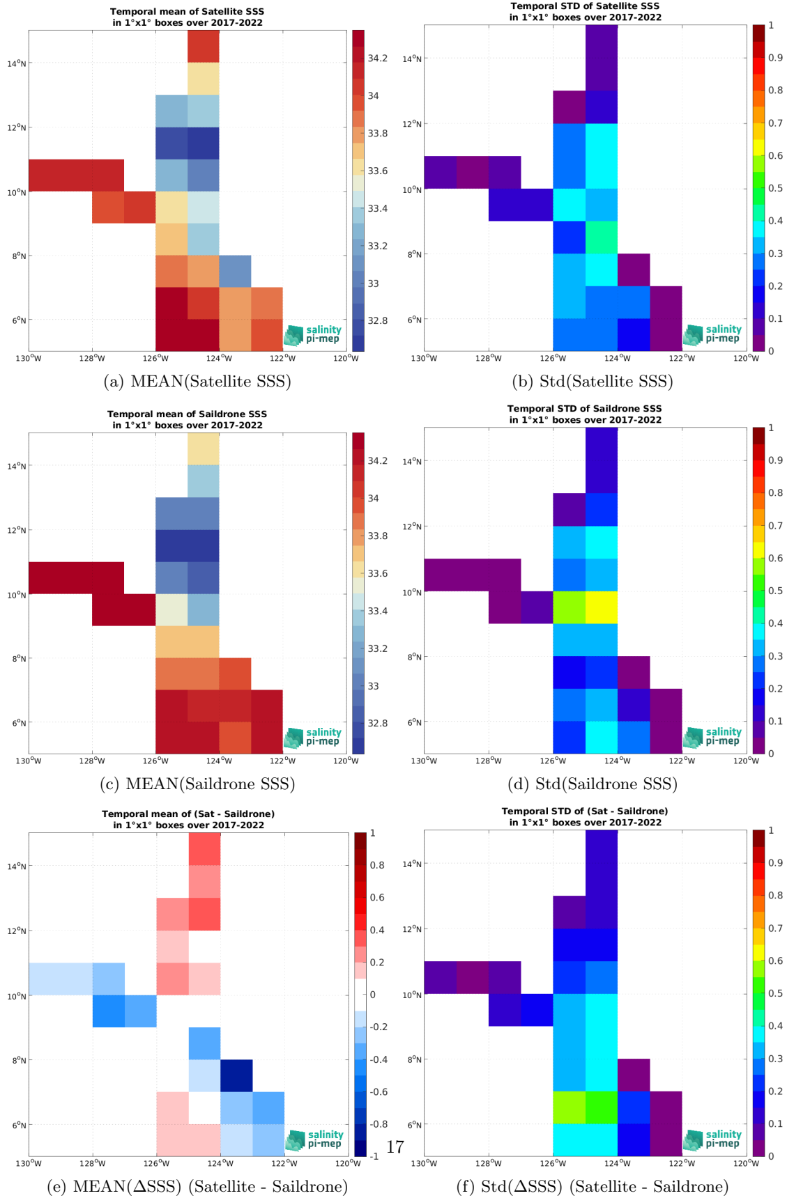
Figure 7: Temporal mean (left) and Std (right) of SSS from SMAP SSS L3 v6 - 8-Day running (RSS) (top), Saildrone (middle), and of \Delta SSS (Satellite - Saildrone). Only match-up pairs are used to generate these maps.
