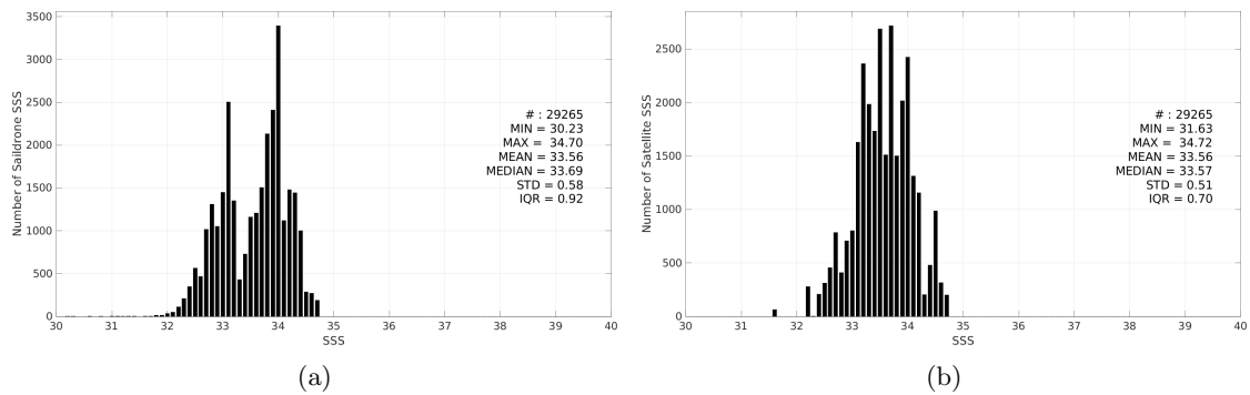
Figure 3: Histograms of SSS from Saildrone (a) and SMAP SSS L3 v6 - 8-Day running (RSS) (b) considering all match-up pairs per bins of 0.1 over the SPURS 2 Pi-MEP region and for the full satellite product period.
