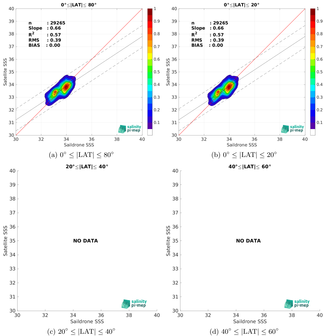
Figure 10: Contour maps of the concentration of SMAP SSS L3 v6 - 8-Day running (RSS) SSS (y-axis) versus Saildrone SSS (x-axis) at match-up pairs for different latitude bands. For each plot, the red line shows x=y . The black thin and dashed lines indicate a linear fit through the data cloud and the \pm 95\% confidence levels, respectively. The number match-up pairs n , the slope and R^2 coefficient of the linear fit, the root mean square (RMS) and the mean bias between satellite and in situ data are indicated for each latitude band in each plots.
