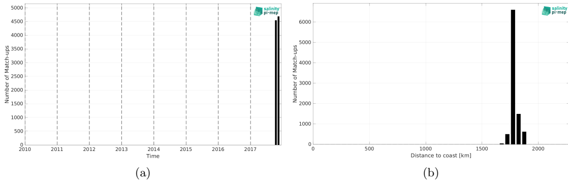
Figure 2: Number of match-ups between Saildrone (SPURS 2) and SMAP SSS L3 v6 - 8-Day running (RSS) SSS as a function of time (a) and as function of the distance to coast (b) over the SPURS 2 Pi-MEP region and for the full satellite product period.
