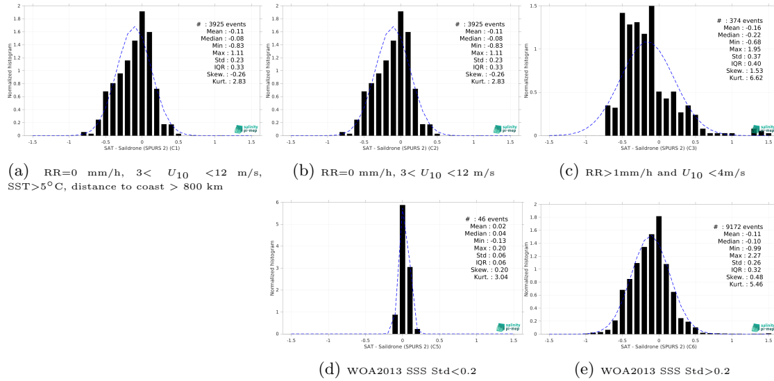
Figure 15: Normalized histogram of \Delta SSS (SMAP SSS L3 v6 - 8-Day running (RSS) - Saldrone (SPURS 2)) for 5 different subdatasets corresponding to: RR=0 mm/h, 3 < U_{10} < 12 m/s, SST > 5°C, distance to coast > 800 km (a), RR=0 mm/h, 3 < U_{10} < 12 m/s (b), RR > 1mm/h and U_{10} < 4 m/s (c), WOA2013 SSS Std < 0.2 (d), WOA2013 SSS Std > 0.2 (e).
