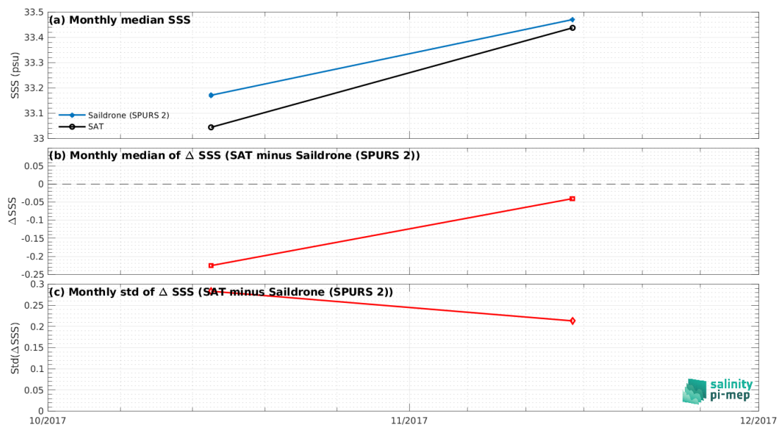
Figure 8: Time series of the monthly median SSS (top), median of \Delta SSS (Satellite - Sairdronne (SPURS 2)) and Std of \Delta SSS (Satellite - Sairdronne (SPURS 2)) over the SPURS 2 Pi-MEP region considering all match-ups collected by the Pi-MEP.
