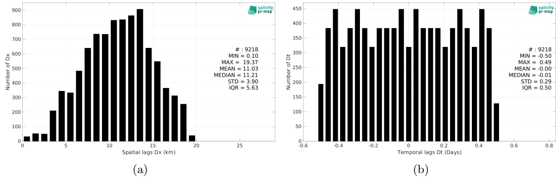
Figure 6: Histograms of the spatial (a) and temporal (b) lags between the location/time of the Saildrone (SPURS 2) measurement and the date of the corresponding SMAP SSS L3 v6 - 8-Day running (RSS) SSS pixel.
