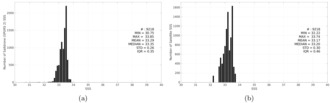
Figure 3: Histograms of SSS from Saildrone (SPURS 2) (a) and SMAP SSS L3 v6 - 8-Day running (RSS) (b) considering all match-up pairs per bins of 0.1 over the SPURS 2 Pi-MEP region and for the full satellite product period.
