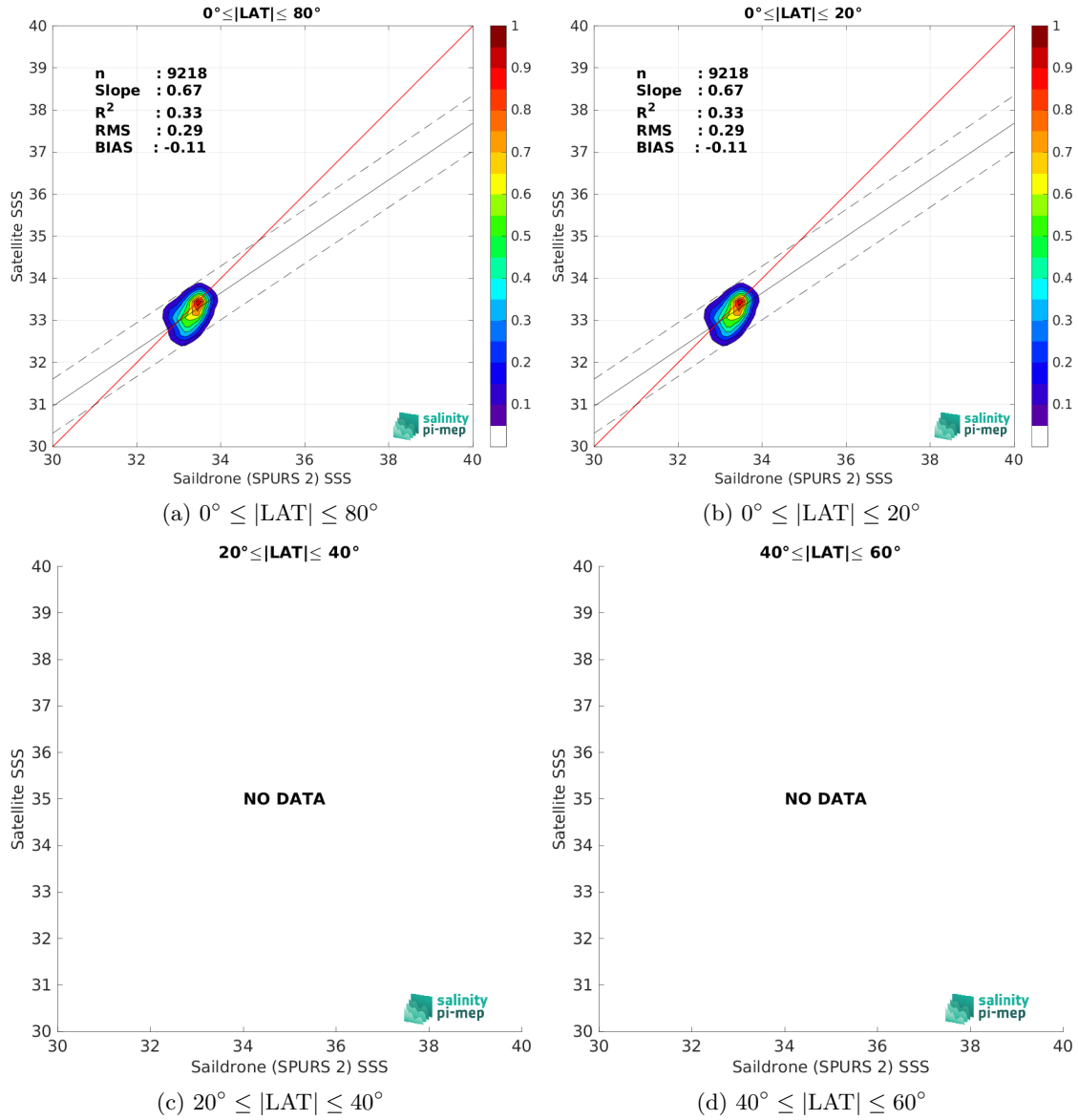
Figure 10: Contour maps of the concentration of SMAP SSS L3 v6 - 8-Day running (RSS) SSS (y-axis) versus Saildrone (SPURS 2) SSS (x-axis) at match-up pairs for different latitude bands. For each plot, the red line shows x=y . The black thin and dashed lines indicate a linear fit through the data cloud and the \pm 95\% confidence levels, respectively. The number match-up pairs n , the slope and R^2 coefficient of the linear fit, the root mean square (RMS) and the mean bias between satellite and in situ data are indicated for each latitude band in each plots.
