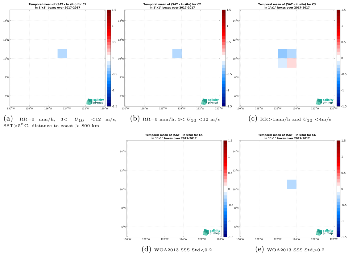
Figure 14: Temporal mean gridded over spatial boxes of size 1^\circ \times 1^\circ of \Delta SSS (SMAP SSS L3 v6 - 8-Day running (RSS) - Sairdron (SPURS 2)) for 5 different subdatasets corresponding to:RR=0 mm/h, 3 < U_{10} < 12 m/s, SST>5°C, distance to coast > 800 km (a), RR=0 mm/h, 3 < U_{10} < 12 m/s (b), RR>1mm/h and U_{10} < 4 m/s (c), WOA2013 SSS Std<0.2 (d), WOA2013 SSS Std>0.2 (e).
