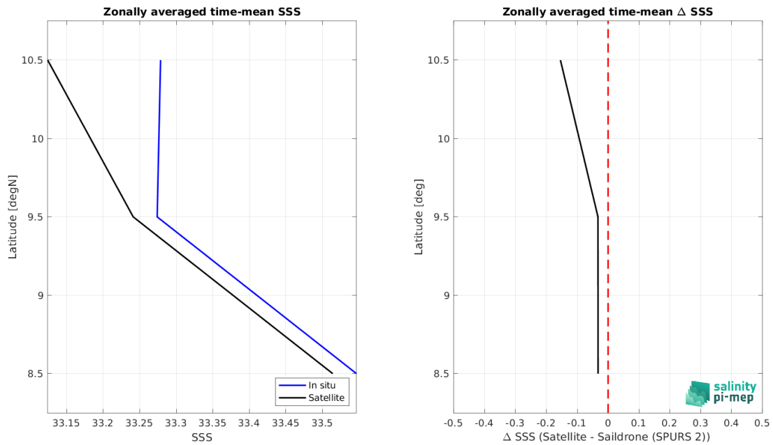
Figure 9: Left panel: Zonal mean SSS from SMAP SSS L3 v6 - 8-Day running (RSS) satellite product (black) and from Sairdron (SPURS 2) (blue). Right panel: Zonal mean of \Delta SSS (Satellite - Sairdron (SPURS 2)) for all the collected Pi-MEP match-up pairs estimated over the full satellite product period.
