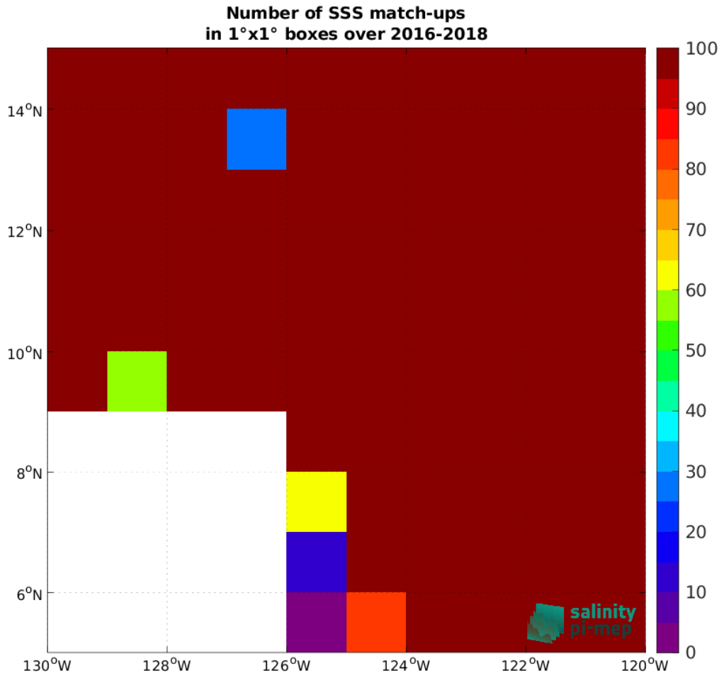
Figure 4: Number of SSS match-ups between Surface drifters SSS and the SMAP SSS L3 v6 - 8-Day running (RSS) SSS product for the SPURS 2 Pi-MEP region over 1^\circ \times 1^\circ boxes and for the full satellite product period.
