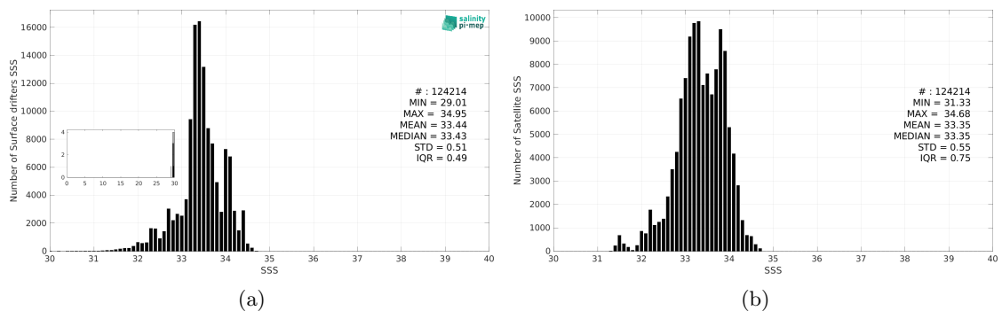
Figure 3: Histograms of SSS from Surface drifters (a) and SMAP SSS L3 v6 - 8-Day running (RSS) (b) considering all match-up pairs per bins of 0.1 over the SPURS 2 Pi-MEP region and for the full satellite product period.
