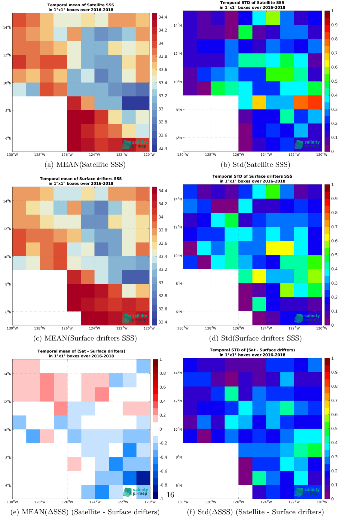
Figure 6: Temporal mean (left) and Std (right) of SSS from SMAP SSS L3 v6 - 8-Day running (RSS) (top), Surface drifters (middle), and of \Delta SSS (Satellite - Surface drifters). Only match-up pairs are used to generate these maps.
