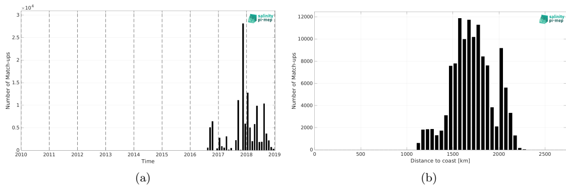
Figure 2: Number of match-ups between Surface drifters and SMAP SSS L3 v6 - 8-Day running (RSS) SSS as a function of time (a) and as function of the distance to coast (b) over the SPURS 2 Pi-MEP region and for the full satellite product period.
