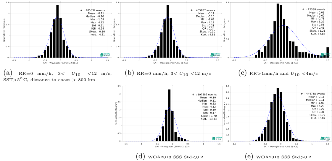
Figure 15: Normalized histogram of \Delta SSS (SMAP SSS L3 v6 - Monthly (RSS) - Waveglider (SPURS 2)) for 5 different subdatasets corresponding to: RR=0 mm/h, 3 < U_{10} < 12 m/s, SST > 5°C, distance to coast > 800 km (a), RR=0 mm/h, 3 < U_{10} < 12 m/s (b), RR > 1mm/h and U_{10} < 4 m/s (c), WOA2013 SSS Std < 0.2 (d), WOA2013 SSS Std > 0.2 (e).
