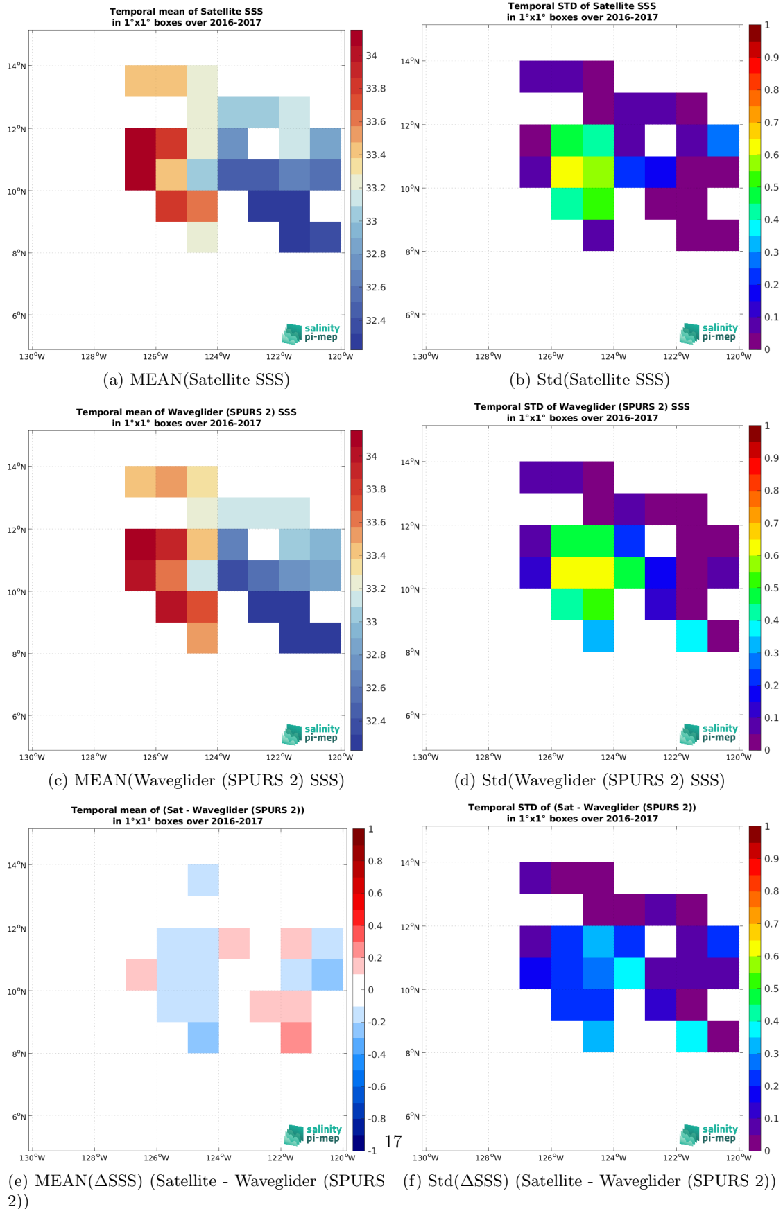
Figure 7: Temporal mean (left) and Std (right) of SSS from SMAP SSS L3 v6 - Monthly (RSS) (top), Waveglider (SPURS 2) (middle), and of \Delta SSS (Satellite - Waveglider (SPURS 2)). Only match-up pairs are used to generate these maps.
