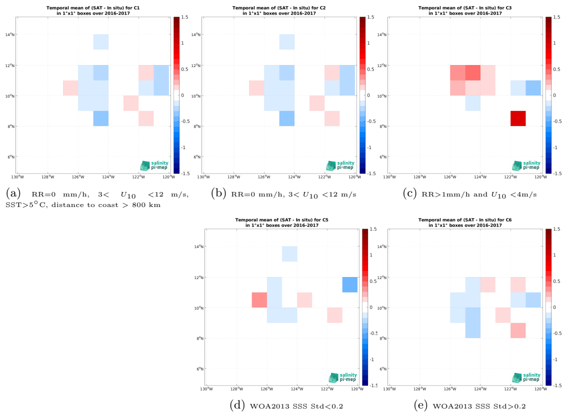
Figure 14: Temporal mean gridded over spatial boxes of size 1^\circ \times 1^\circ of \Delta SSS (SMAP SSS L3 v6 - Monthly (RSS) - Waveglider (SPURS 2)) for 5 different subdatasets corresponding to:RR=0 mm/h, 3 < U_{10} < 12 m/s, SST >5^\circ\text{C} , distance to coast > 800 km (a), RR=0 mm/h, 3 < U_{10} < 12 m/s (b), RR >1 mm/h and U_{10} < 4 m/s (c), WOA2013 SSS Std <0.2 (d), WOA2013 SSS Std >0.2 (e).
