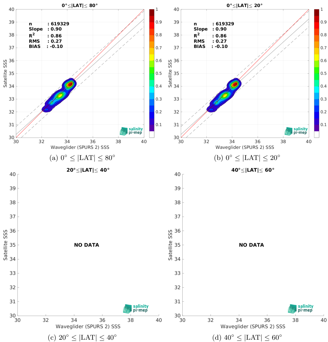
Figure 10: Contour maps of the concentration of SMAP SSS L3 v6 - Monthly (RSS) SSS (y-axis) versus Waveglider (SPURS 2) SSS (x-axis) at match-up pairs for different latitude bands. For each plot, the red line shows x=y . The black thin and dashed lines indicate a linear fit through the data cloud and the \pm 95\% confidence levels, respectively. The number match-up pairs n , the slope and R^2 coefficient of the linear fit, the root mean square (RMS) and the mean bias between satellite and in situ data are indicated for each latitude band in each plots.
