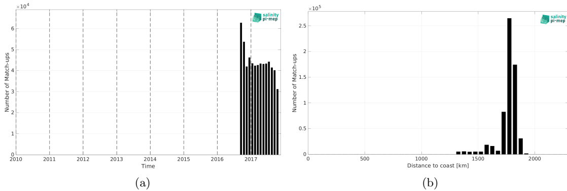
Figure 2: Number of match-ups between Waveglider (SPURS 2) and SMAP SSS L3 v6 - Monthly (RSS) SSS as a function of time (a) and as function of the distance to coast (b) over the SPURS 2 Pi-MEP region and for the full satellite product period.
