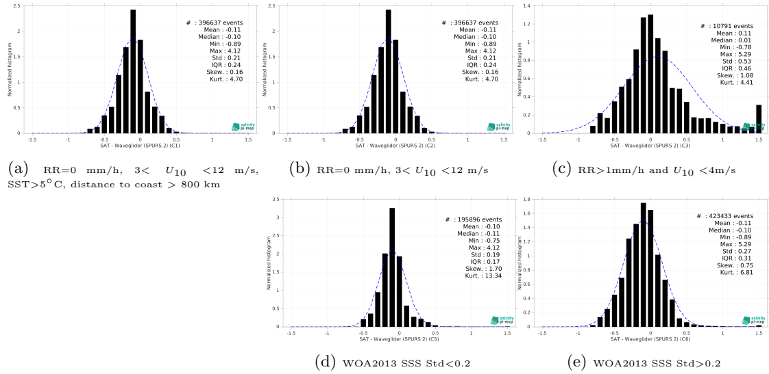
Figure 15: Normalized histogram of \Delta SSS (SMAP SSS L3 v6 - Monthly (RSS) - Waveglider (SPURS 2)) for 5 different subdatasets corresponding to: RR=0 mm/h, 3 < U_{10} < 12 m/s, SST>5°C, distance to coast > 800 km (a), RR=0 mm/h, 3 < U_{10} < 12 m/s (b), RR>1mm/h and U_{10} < 4 m/s (c), WOA2013 SSS Std<0.2 (d), WOA2013 SSS Std>0.2 (e).
