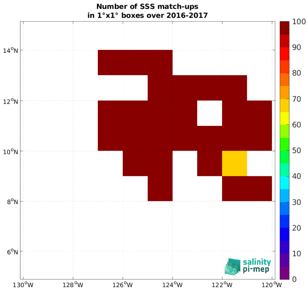
Figure 5: Number of SSS match-ups between Waveglider (SPURS 2) SSS and the SMAP SSS L3 v6 - Monthly (RSS) SSS product for the SPURS 2 Pi-MEP region over 1°x1° boxes and for the full satellite product period.
