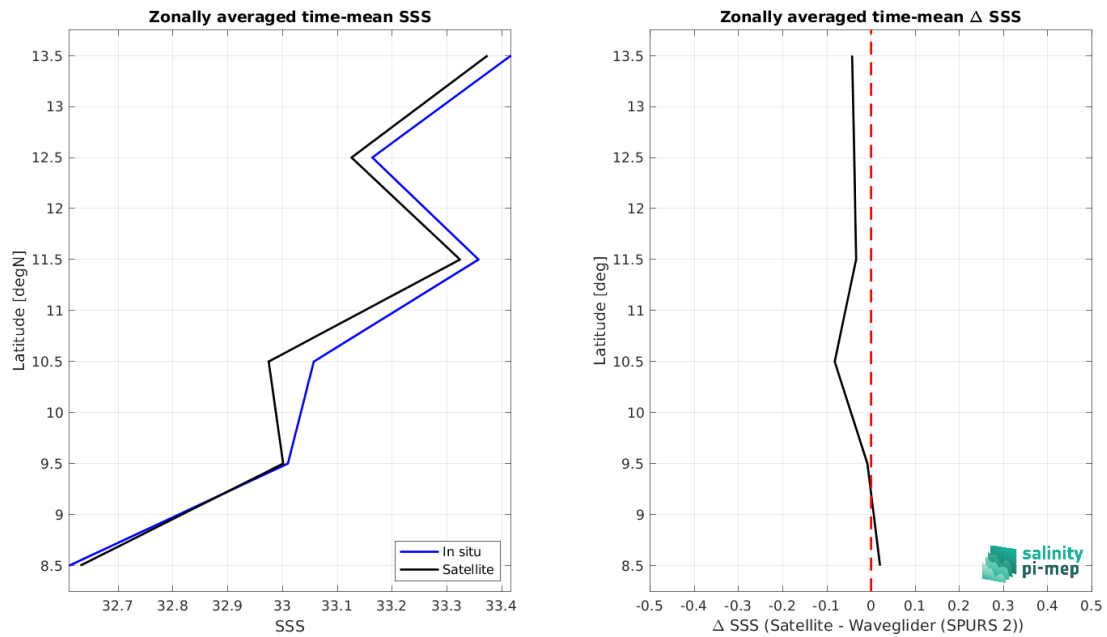
Figure 9: Left panel: Zonal mean SSS from SMAP SSS L3 v6 - Monthly (RSS) satellite product (black) and from Waveglider (SPURS 2) (blue). Right panel: Zonal mean of \Delta SSS (Satellite - Waveglider (SPURS 2)) for all the collected Pi-MEP match-up pairs estimated over the full satellite product period.
