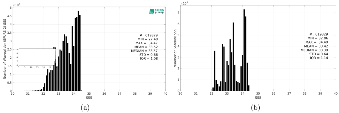
Figure 3: Histograms of SSS from Waveglider (SPURS 2) (a) and SMAP SSS L3 v6 - Monthly (RSS) (b) considering all match-up pairs per bins of 0.1 over the SPURS 2 Pi-MEP region and for the full satellite product period.
