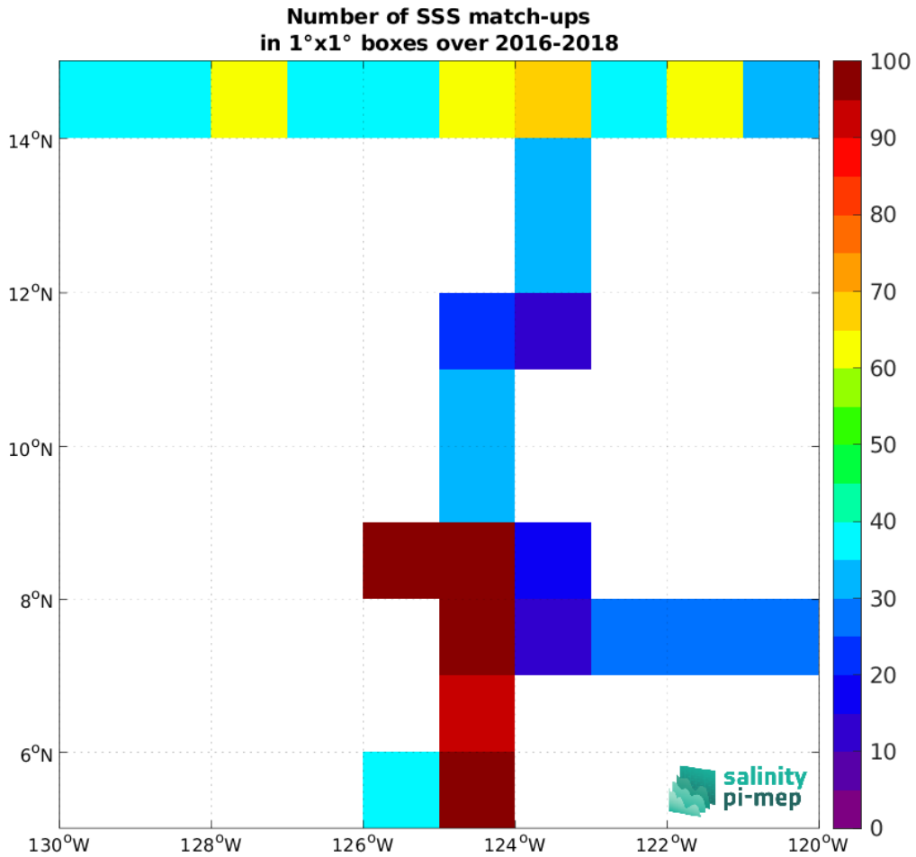
Figure 5: Number of SSS match-ups between TSG (SAMOS) SSS and the SMAP SSS L3 v6 - Monthly (RSS) SSS product for the SPURS 2 Pi-MEP region over 1^\circ \times 1^\circ boxes and for the full satellite product period.
