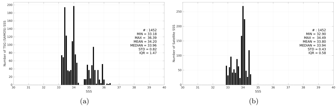
Figure 3: Histograms of SSS from TSG (SAMOS) (a) and SMAP SSS L3 v6 - Monthly (RSS) (b) considering all match-up pairs per bins of 0.1 over the SPURS 2 Pi-MEP region and for the full satellite product period.
