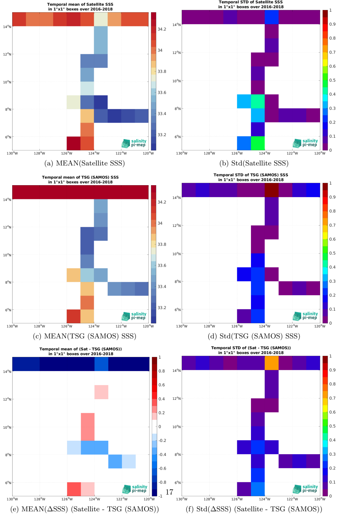
Figure 7: Temporal mean (left) and Std (right) of SSS from SMAP SSS L3 v6 - Monthly (RSS) (top), TSG (SAMOS) (middle), and of \Delta SSS (Satellite - TSG (SAMOS)). Only match-up pairs are used to generate these maps.
