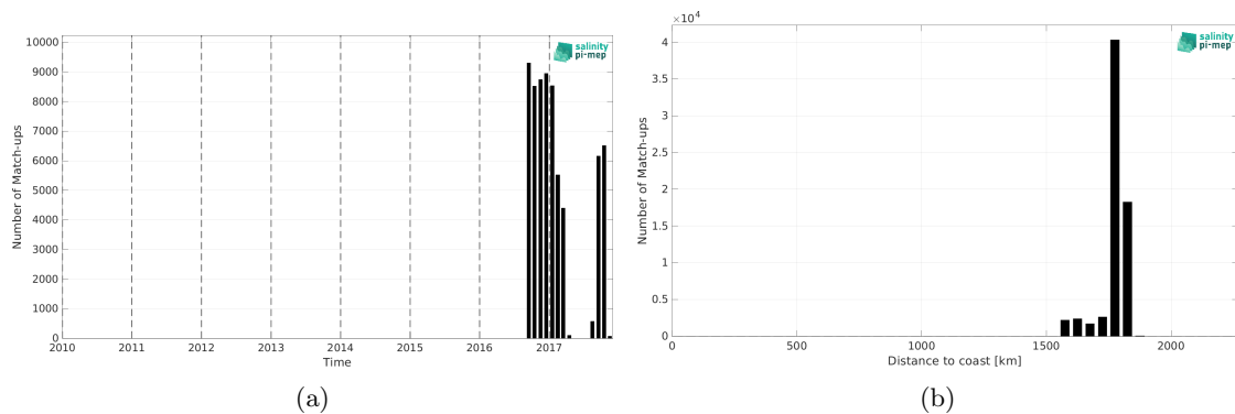
Figure 2: Number of match-ups between Seaglider (SPURS 2) and SMAP SSS L3 v6 - Monthly (RSS) SSS as a function of time (a) and as function of the distance to coast (b) over the SPURS 2 Pi-MEP region and for the full satellite product period.
