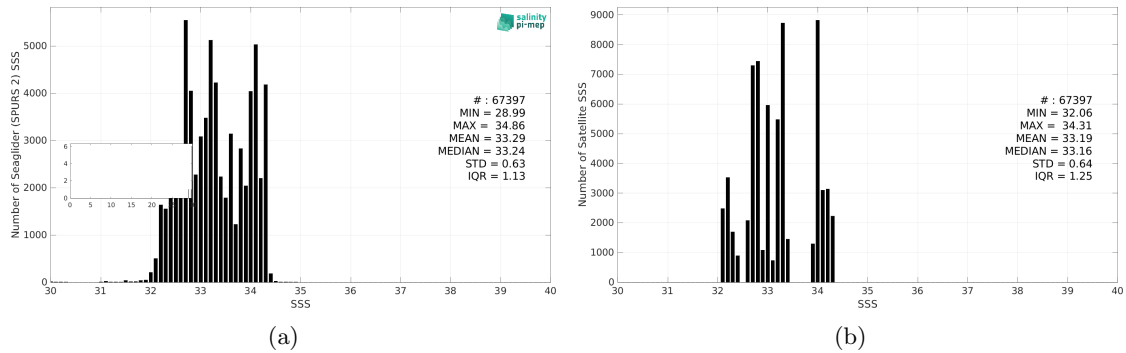
Figure 3: Histograms of SSS from Seaglider (SPURS 2) (a) and SMAP SSS L3 v6 - Monthly (RSS) (b) considering all match-up pairs per bins of 0.1 over the SPURS 2 Pi-MEP region and for the full satellite product period.
