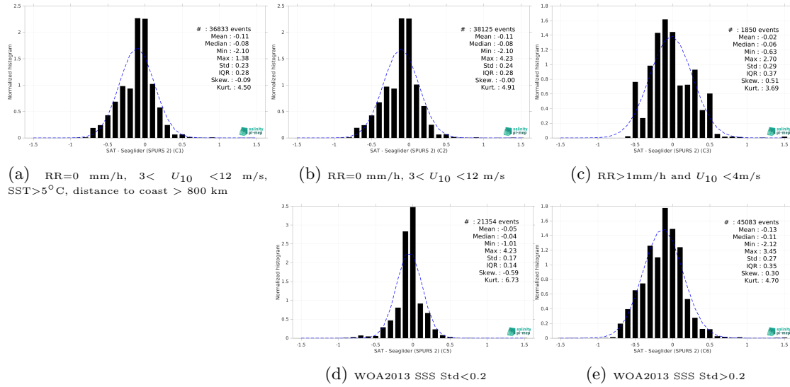
Figure 15: Normalized histogram of \Delta SSS (SMAP SSS L3 v6 - Monthly (RSS) - Seaglider (SPURS 2)) for 5 different subdatasets corresponding to: RR=0 mm/h, 3 < U_{10} < 12 m/s, SST>5°C, distance to coast > 800 km (a), RR=0 mm/h, 3 < U_{10} < 12 m/s (b), RR>1mm/h and U_{10} < 4 m/s (c), WOA2013 SSS Std<0.2 (d), WOA2013 SSS Std>0.2 (e).
