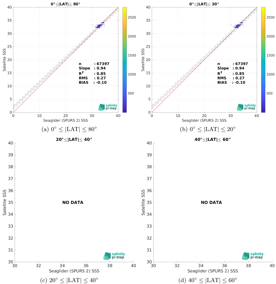
Figure 10: Contour maps of the concentration of SMAP SSS L3 v6 - Monthly (RSS) SSS (y-axis) versus Seaglider (SPURS 2) SSS (x-axis) at match-up pairs for different latitude bands. For each plot, the red line shows x=y . The black thin and dashed lines indicate a linear fit through the data cloud and the \pm 95\% confidence levels, respectively. The number match-up pairs n , the slope and R^2 coefficient of the linear fit, the root mean square (RMS) and the mean bias between satellite and in situ data are indicated for each latitude band in each plots.
