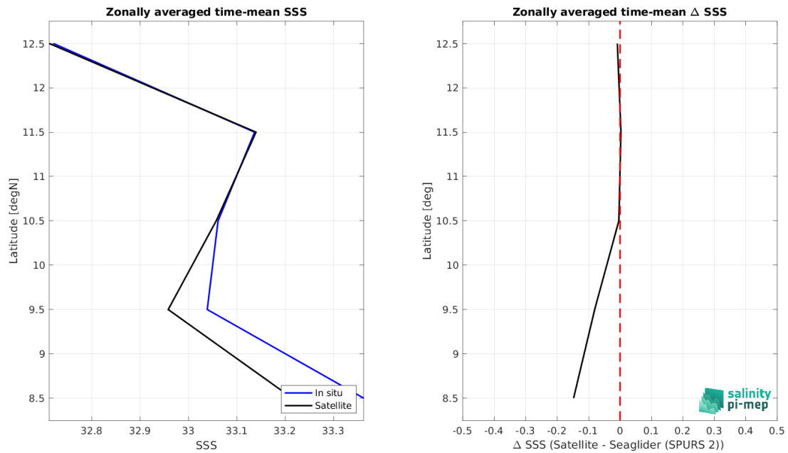
Figure 9: Left panel: Zonal mean SSS from SMAP SSS L3 v6 - Monthly (RSS) satellite product (black) and from Seaglider (SPURS 2) (blue). Right panel: Zonal mean of \Delta SSS (Satellite - Seaglider (SPURS 2)) for all the collected Pi-MEP match-up pairs estimated over the full satellite product period.
