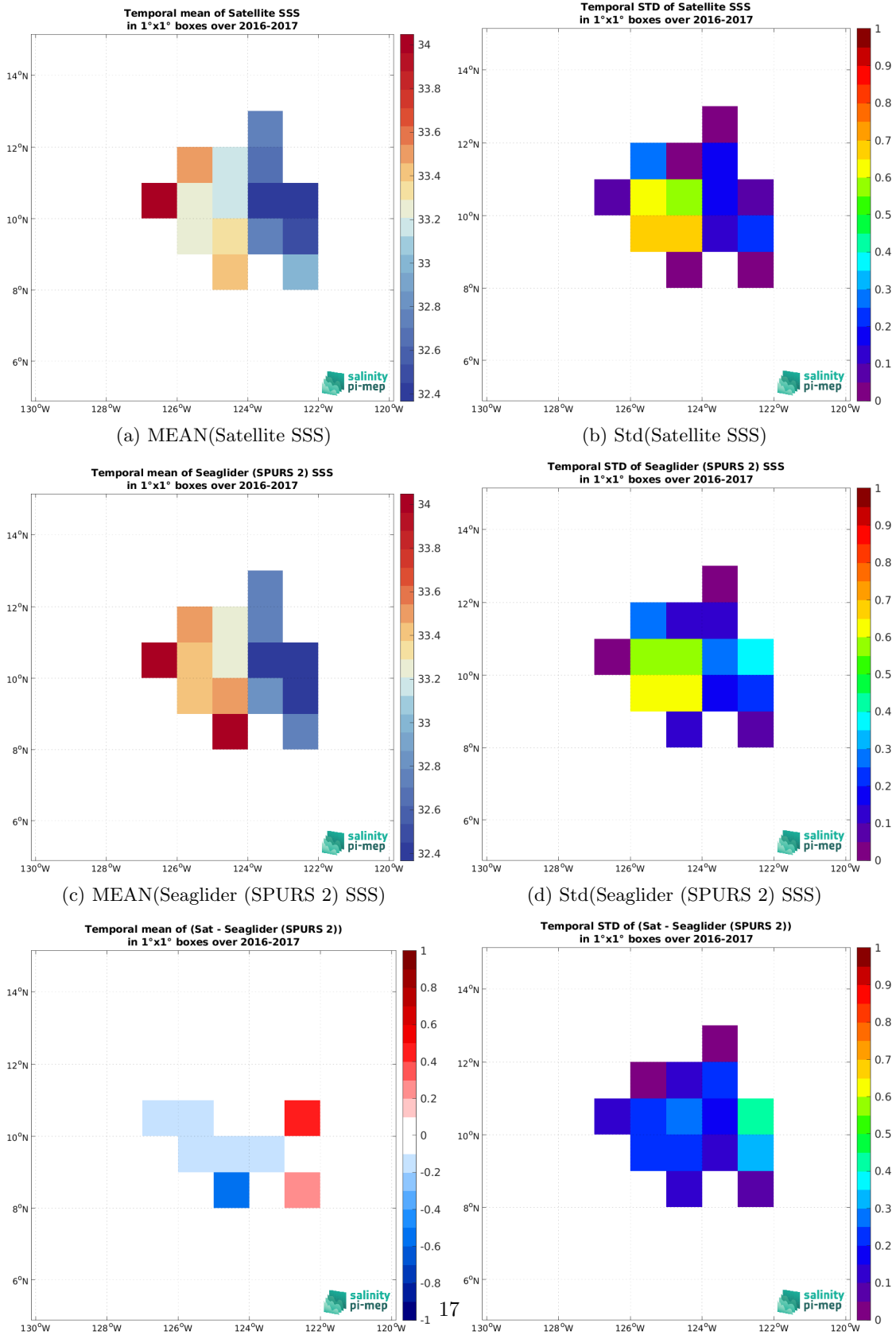
Figure 7: Temporal mean (left) and Std (right) of SSS from SMAP SSS L3 v6 - Monthly (RSS) (top), Seaglider (SPURS 2) (middle), and of \Delta SSS (Satellite - Seaglider (SPURS 2)). Only match-up pairs are used to generate these maps.
