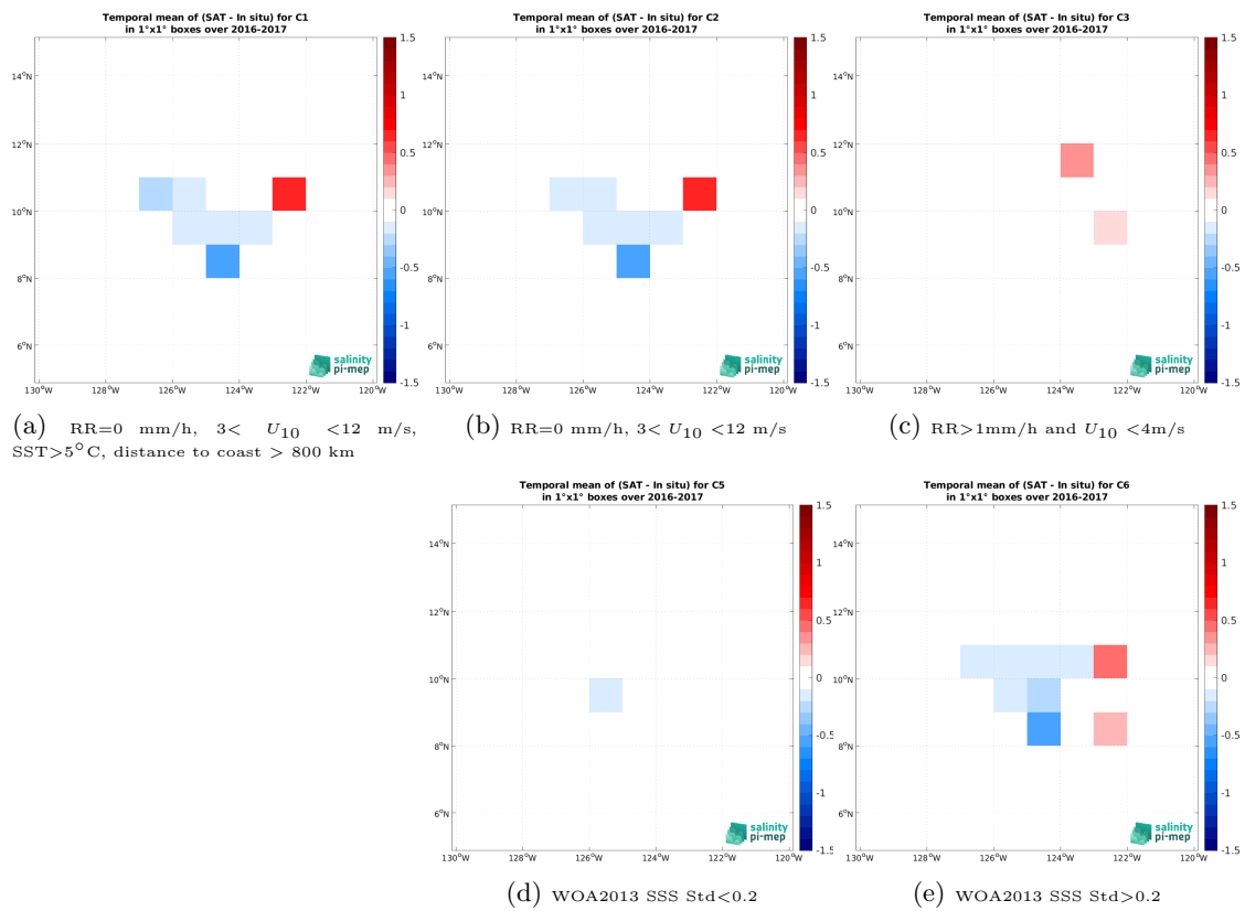
Figure 14: Temporal mean gridded over spatial boxes of size 1^\circ \times 1^\circ of \Delta SSS (SMAP SSS L3 v6 - Monthly (RSS) - Seaglider (SPURS 2)) for 5 different subdatasets corresponding to:RR=0 mm/h, 3 < U_{10} < 12 m/s, SST>5°C, distance to coast > 800 km (a), RR=0 mm/h, 3 < U_{10} < 12 m/s (b), RR>1mm/h and U_{10} < 4 m/s (c), WOA2013 SSS Std<0.2 (d), WOA2013 SSS Std>0.2 (e).
