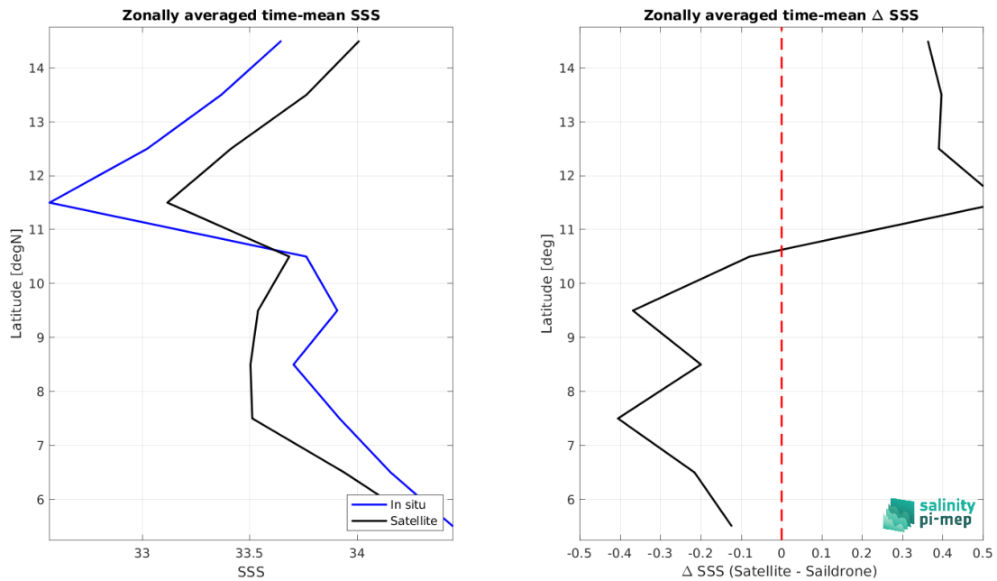
Figure 9: Left panel: Zonal mean SSS from SMAP SSS L3 v6 - Monthly (RSS) satellite product (black) and from Sairdrone (blue). Right panel: Zonal mean of \Delta SSS (Satellite - Sairdrone) for all the collected Pi-MEP match-up pairs estimated over the full satellite product period.
