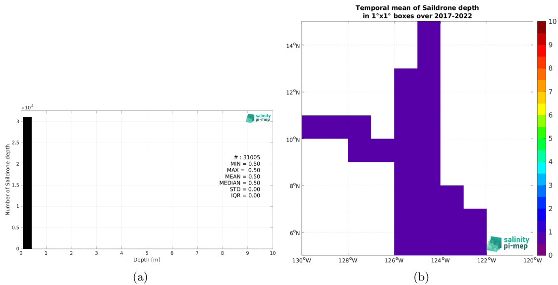
Figure 4: Histograms of the depth of the upper level SSS measurements from Saïdrone in the Match-up DataBase for the SPURS 2 Pi-MEP region (a) and temporal mean spatial distribution of pressure of the in situ SSS data over 1^\circ \times 1^\circ boxes and for the full satellite product period (b).
