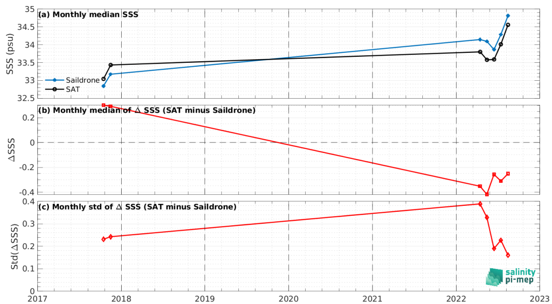
Figure 8: Time series of the monthly median SSS (top), median of \Delta SSS (Satellite - Sairdrone) and Std of \Delta SSS (Satellite - Sairdrone) over the SPURS 2 Pi-MEP region considering all match-ups collected by the Pi-MEP.
