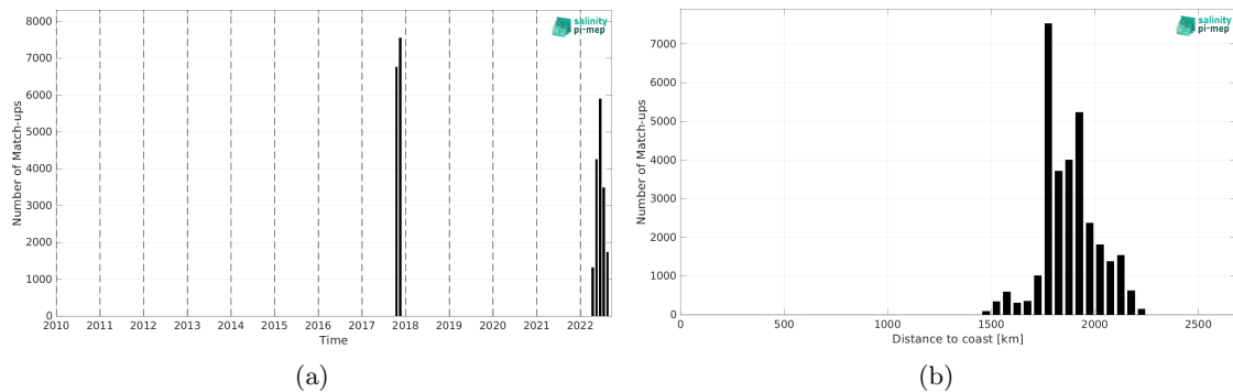
Figure 2: Number of match-ups between Sairdrone and SMAP SSS L3 v6 - Monthly (RSS) SSS as a function of time (a) and as function of the distance to coast (b) over the SPURS 2 Pi-MEP region and for the full satellite product period.
