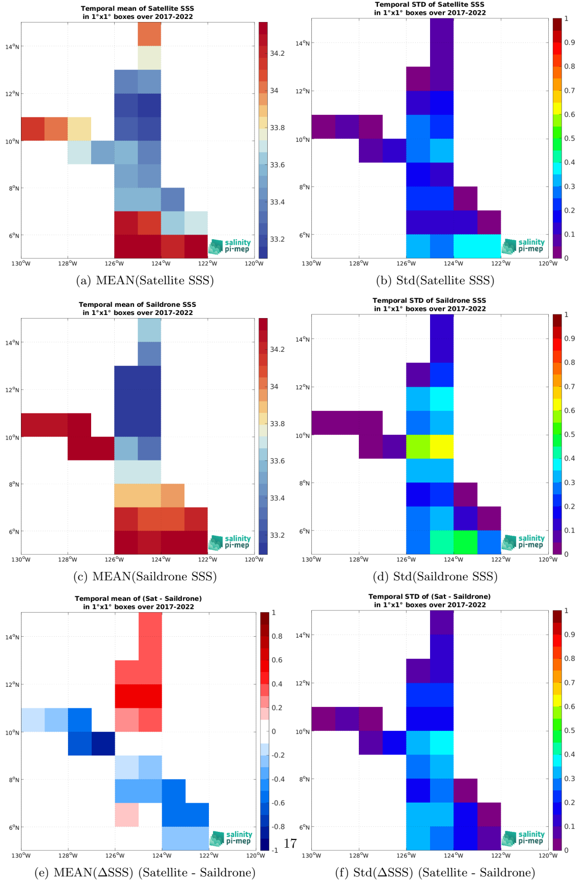
Figure 7: Temporal mean (left) and Std (right) of SSS from SMAP SSS L3 v6 - Monthly (RSS) (top), Saildrone (middle), and of \Delta SSS (Satellite - Saildrone). Only match-up pairs are used to generate these maps.
