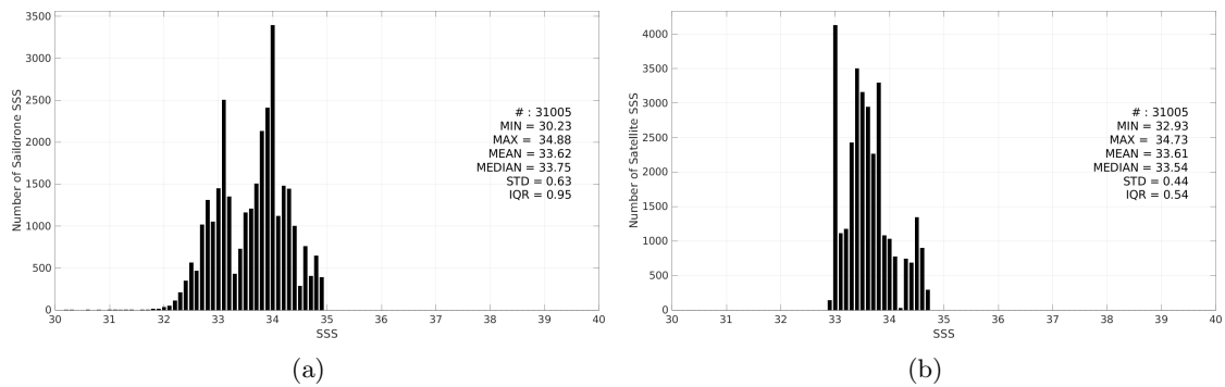
Figure 3: Histograms of SSS from Saïdrone (a) and SMAP SSS L3 v6 - Monthly (RSS) (b) considering all match-up pairs per bins of 0.1 over the SPURS 2 Pi-MEP region and for the full satellite product period.
