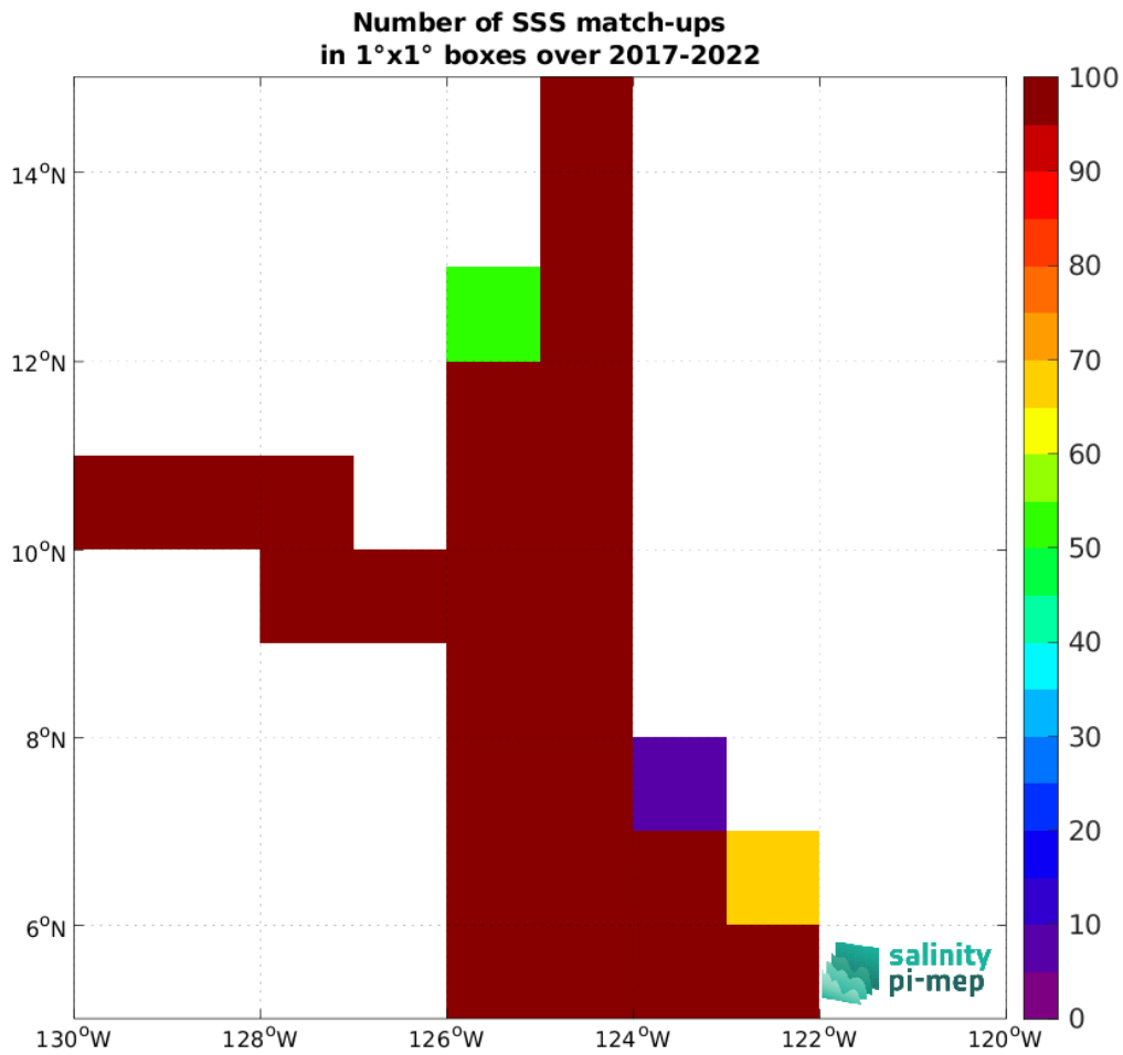
Figure 5: Number of SSS match-ups between Saildrone SSS and the SMAP SSS L3 v6 - Monthly (RSS) SSS product for the SPURS 2 Pi-MEP region over 1°x1° boxes and for the full satellite product period.
