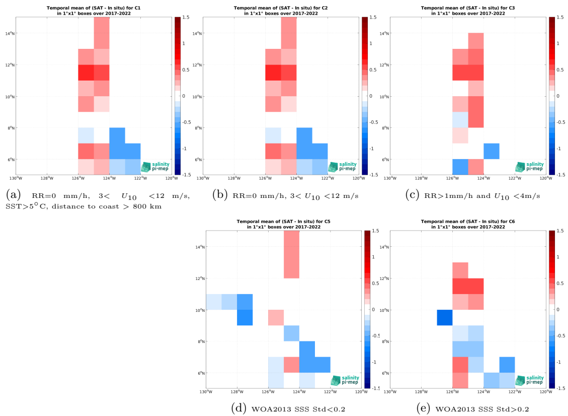
Figure 14: Temporal mean gridded over spatial boxes of size 1^\circ \times 1^\circ of \Delta SSS (SMAP SSS L3 v6 - Monthly (RSS) - Sairdrone) for 5 different subdatasets corresponding to:RR=0 mm/h, 3 < U_{10} < 12 m/s, SST > 5°C, distance to coast > 800 km (a), RR=0 mm/h, 3 < U_{10} < 12 m/s (b), RR > 1mm/h and U_{10} < 4 m/s (c), WOA2013 SSS Std < 0.2 (d), WOA2013 SSS Std > 0.2 (e).
