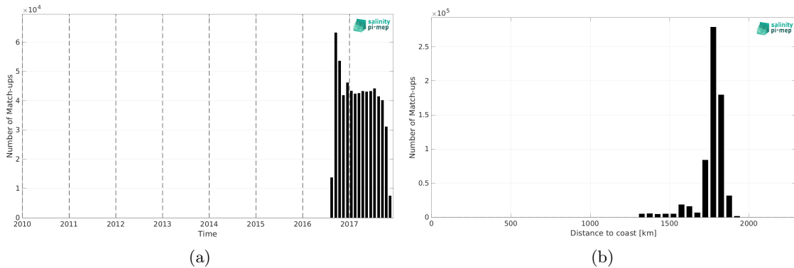
Figure 2: Number of match-ups between Waveglider (SPURS 2) and SMAP SSS L3 v5.3 - 8-Day running (RSS) SSS as a function of time (a) and as function of the distance to coast (b) over the SPURS 2 Pi-MEP region and for the full satellite product period.
