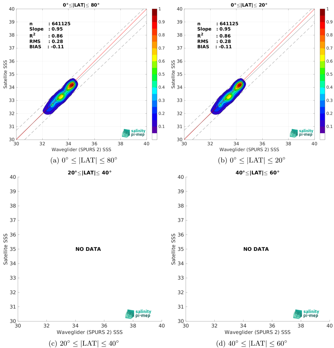
Figure 10: Contour maps of the concentration of SMAP SSS L3 v5.3 - 8-Day running (RSS) SSS (y-axis) versus Waveglider (SPURS 2) SSS (x-axis) at match-up pairs for different latitude bands. For each plot, the red line shows x=y . The black thin and dashed lines indicate a linear fit through the data cloud and the \pm 95\% confidence levels, respectively. The number match-up pairs n , the slope and R^2 coefficient of the linear fit, the root mean square (RMS) and the mean bias between satellite and in situ data are indicated for each latitude band in each plots.
