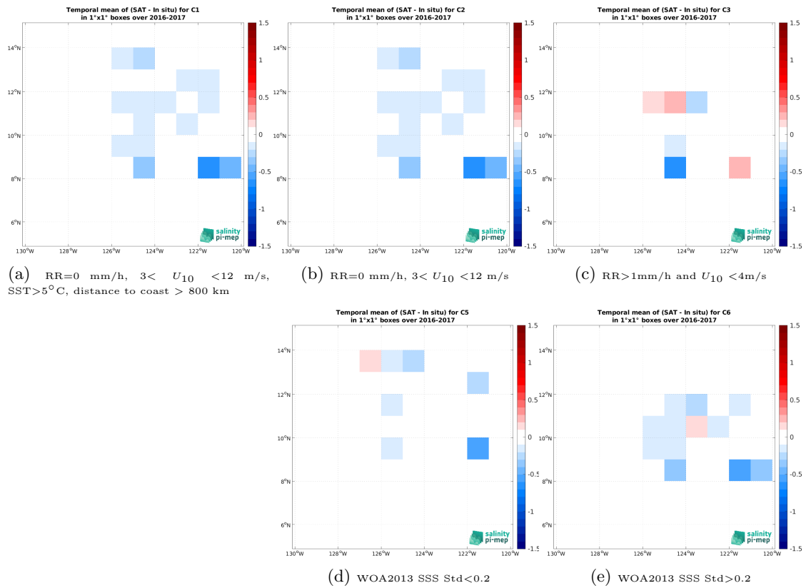
Figure 14: Temporal mean gridded over spatial boxes of size 1^\circ \times 1^\circ of \Delta SSS (SMAP SSS L3 v5.3 - 8-Day running (RSS) - Waveglider (SPURS 2)) for 5 different subdatasets corresponding to:RR=0 mm/h, 3 < U_{10} < 12 m/s, SST >5^\circ C, distance to coast > 800 km (a), RR=0 mm/h, 3 < U_{10} < 12 m/s (b), RR >1 mm/h and U_{10} < 4 m/s (c), WOA2013 SSS Std <0.2 (d), WOA2013 SSS Std >0.2 (e).
