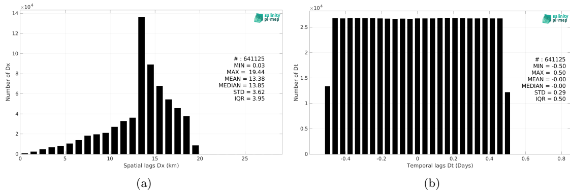
Figure 6: Histograms of the spatial (a) and temporal (b) lags between the location/time of the Waveglider (SPURS 2) measurement and the date of the corresponding SMAP SSS L3 v5.3 - 8-Day running (RSS) SSS pixel.
