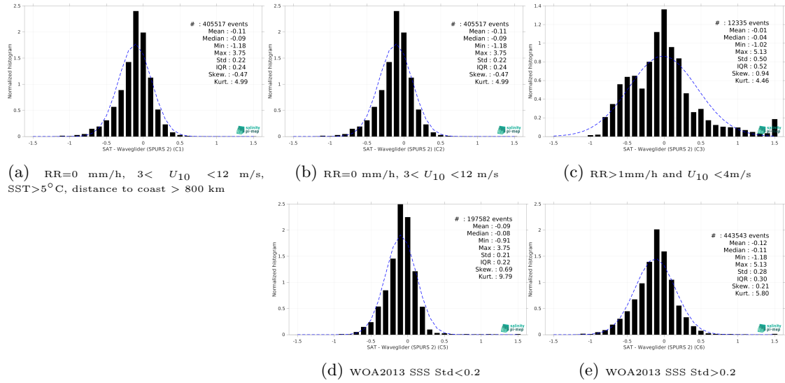
Figure 15: Normalized histogram of \Delta\text{SSS} (SMAP SSS L3 v5.3 - 8-Day running (RSS) - Waveglider (SPURS 2)) for 5 different subdatasets corresponding to: RR=0 mm/h, 3 < U_{10} < 12 m/s, SST>5°C, distance to coast > 800 km (a), RR=0 mm/h, 3 < U_{10} < 12 m/s (b), RR>1mm/h and U_{10} < 4 m/s (c), WOA2013 SSS Std<0.2 (d), WOA2013 SSS Std>0.2 (e).
