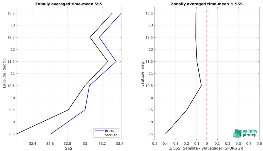
Figure 9: Left panel: Zonal mean SSS from SMAP SSS L3 v5.3 - 8-Day running (RSS) satellite product (black) and from Waveglider (SPURS 2) (blue). Right panel: Zonal mean of \Delta SSS (Satellite - Waveglider (SPURS 2)) for all the collected Pi-MEP match-up pairs estimated over the full satellite product period.
