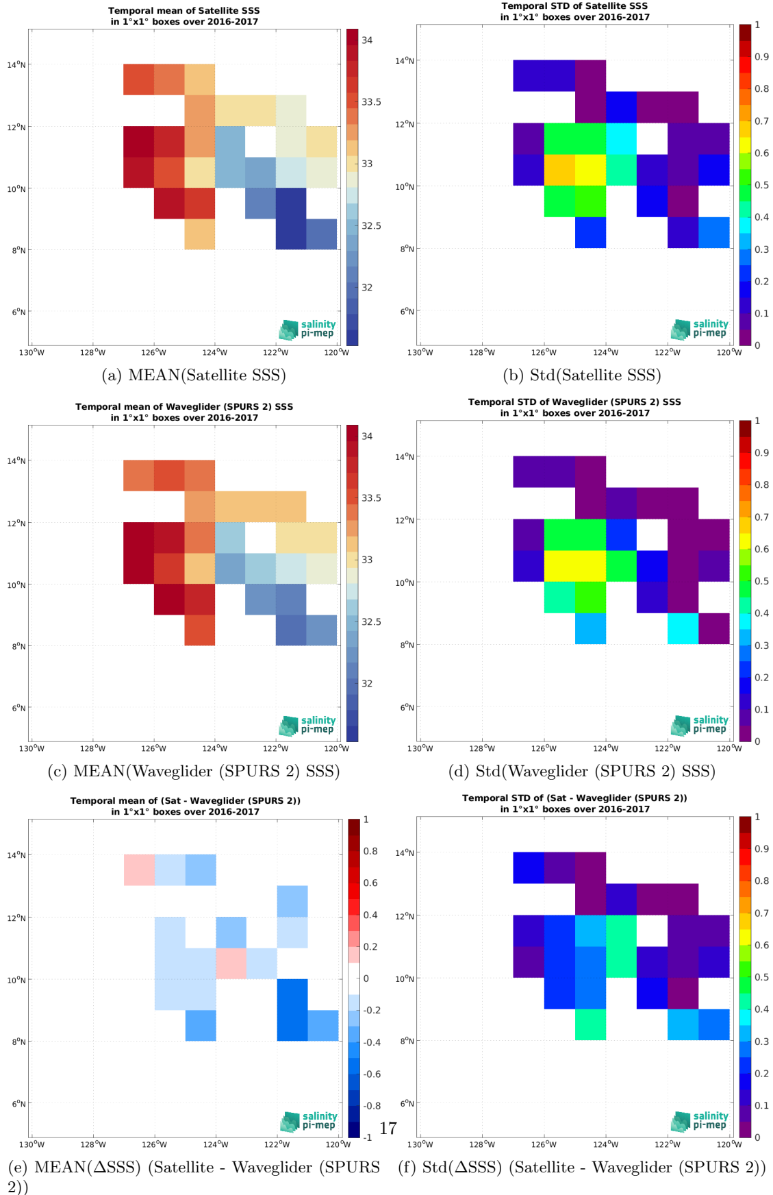
Figure 7: Temporal mean (left) and Std (right) of SSS from SMAP SSS L3 v5.3 - 8-Day running (RSS) (top), Waveglider (SPURS 2) (middle), and of \Delta SSS (Satellite - Waveglider (SPURS 2)). Only match-up pairs are used to generate these maps.
