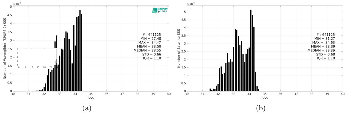
Figure 3: Histograms of SSS from Waveglider (SPURS 2) (a) and SMAP SSS L3 v5.3 - 8-Day running (RSS) (b) considering all match-up pairs per bins of 0.1 over the SPURS 2 Pi-MEP region and for the full satellite product period.
