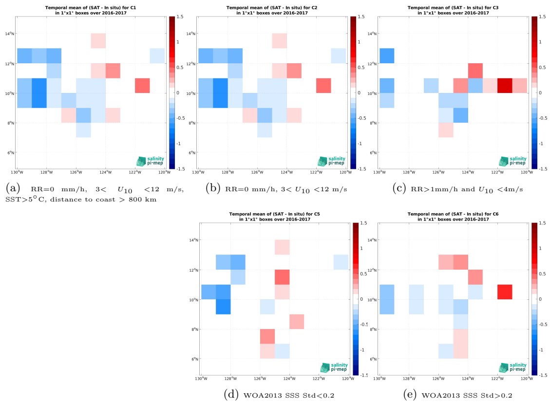
Figure 14: Temporal mean gridded over spatial boxes of size 1^\circ \times 1^\circ of \Delta\text{SSS} (SMAP SSS L3 v5.3 - 8-Day running (RSS) - Salinity Snake (SPURS 2)) for 5 different subdatasets corresponding to:RR=0 mm/h, 3 < U_{10} < 12 m/s, SST>5°C, distance to coast > 800 km (a), RR=0 mm/h, 3 < U_{10} < 12 m/s (b), RR>1mm/h and U_{10} < 4 m/s (c), WOA2013 SSS Std<0.2 (d), WOA2013 SSS Std>0.2 (e).
