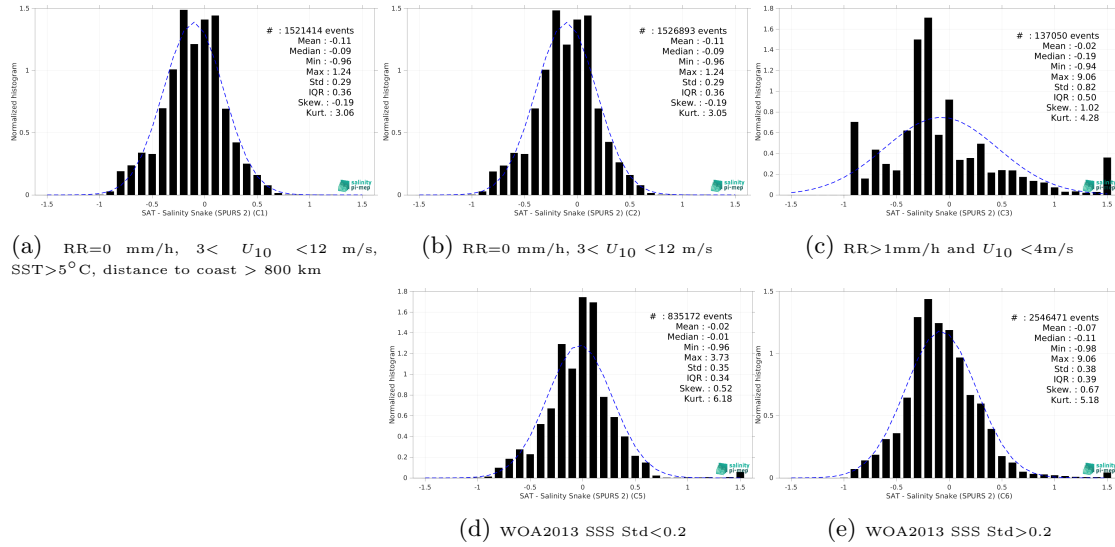
Figure 15: Normalized histogram of \Delta SSS (SMAP SSS L3 v5.3 - 8-Day running (RSS) - Salinity Snake (SPURS 2)) for 5 different subdatasets corresponding to: RR=0 mm/h, 3 < U_{10} < 12 m/s, SST > 5°C, distance to coast > 800 km (a), RR=0 mm/h, 3 < U_{10} < 12 m/s (b), RR > 1mm/h and U_{10} < 4 m/s (c), WOA2013 SSS Std < 0.2 (d), WOA2013 SSS Std > 0.2 (e).
