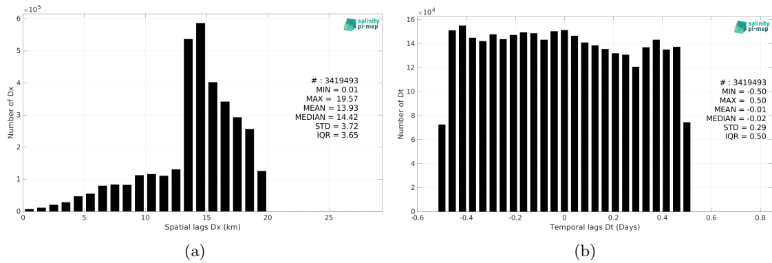
Figure 6: Histograms of the spatial (a) and temporal (b) lags between the location/time of the Salinity Snake (SPURS 2) measurement and the date of the corresponding SMAP SSS L3 v5.3 - 8-Day running (RSS) SSS pixel.
