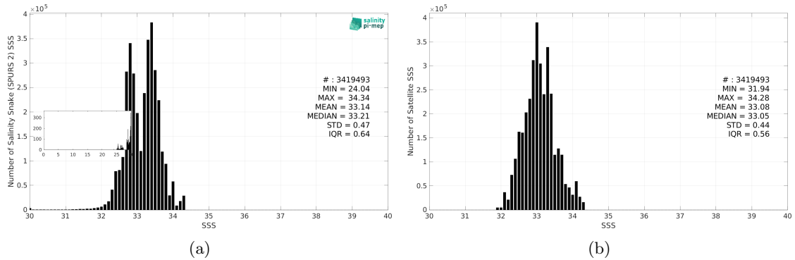
Figure 3: Histograms of SSS from Salinity Snake (SPURS 2) (a) and SMAP SSS L3 v5.3 - 8-Day running (RSS) (b) considering all match-up pairs per bins of 0.1 over the SPURS 2 Pi-MEP region and for the full satellite product period.
