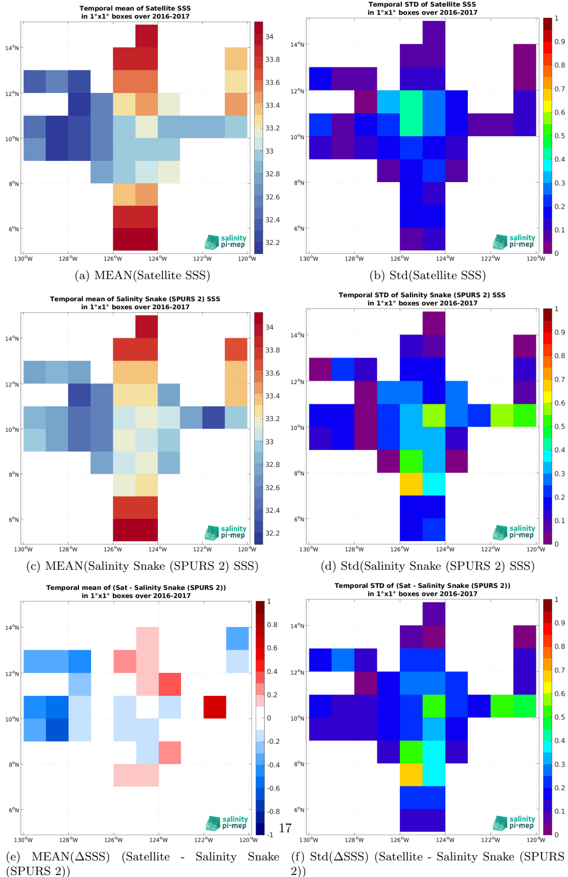
Figure 7: Temporal mean (left) and Std (right) of SSS from SMAP SSS L3 v5.3 - 8-Day running (RSS) (top), Salinity Snake (SPURS 2) (middle), and of \Delta SSS (Satellite - Salinity Snake (SPURS 2)). Only match-up pairs are used to generate these maps.
