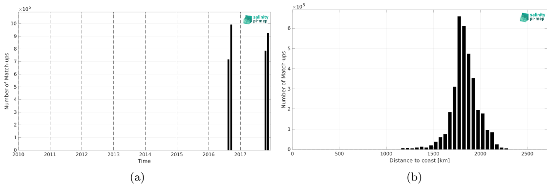
Figure 2: Number of match-ups between Salinity Snake (SPURS 2) and SMAP SSS L3 v5.3 - 8-Day running (RSS) SSS as a function of time (a) and as function of the distance to coast (b) over the SPURS 2 Pi-MEP region and for the full satellite product period.
