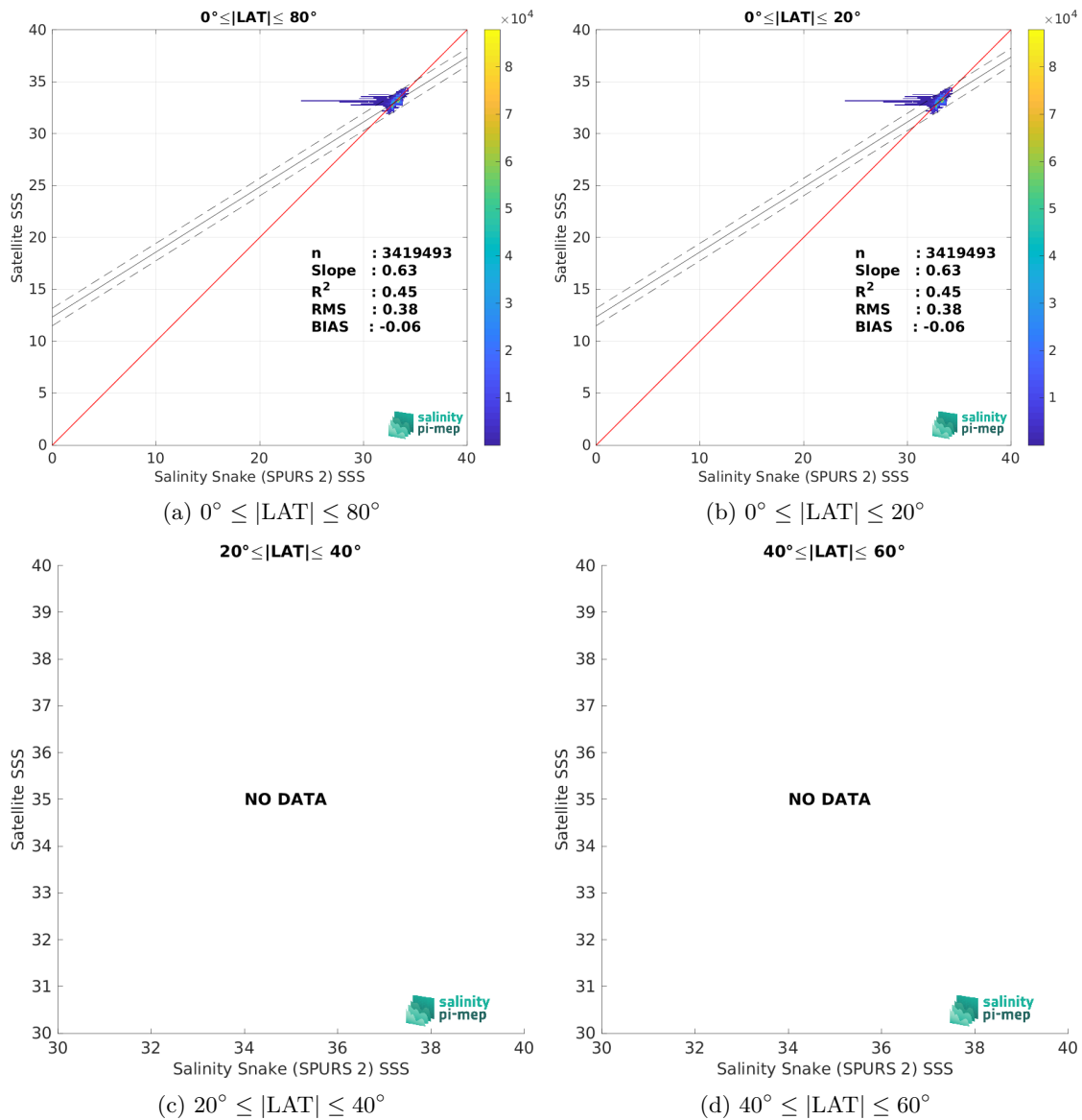
Figure 10: Contour maps of the concentration of SMAP SSS L3 v5.3 - 8-Day running (RSS) SSS (y-axis) versus Salinity Snake (SPURS 2) SSS (x-axis) at match-up pairs for different latitude bands. For each plot, the red line shows x=y . The black thin and dashed lines indicate a linear fit through the data cloud and the \pm 95\% confidence levels, respectively. The number match-up pairs n , the slope and R^2 coefficient of the linear fit, the root mean square (RMS) and the mean bias between satellite and in situ data are indicated for each latitude band in each plots.
