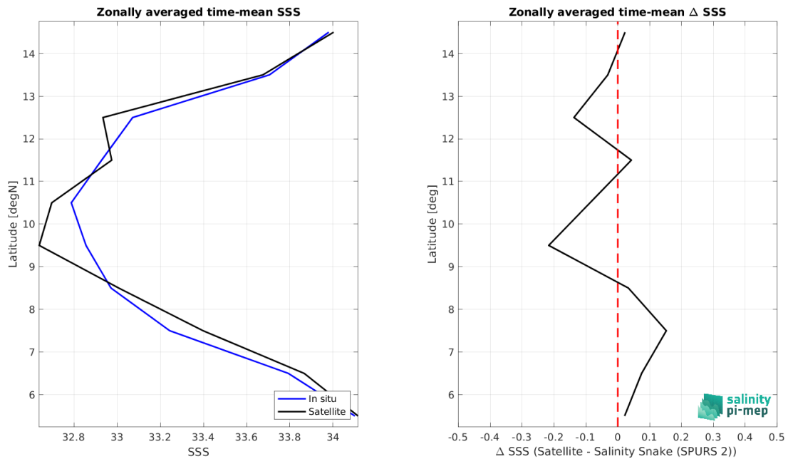
Figure 9: Left panel: Zonal mean SSS from SMAP SSS L3 v5.3 - 8-Day running (RSS) satellite product (black) and from Salinity Snake (SPURS 2) (blue). Right panel: Zonal mean of \Delta SSS (Satellite - Salinity Snake (SPURS 2)) for all the collected Pi-MEP match-up pairs estimated over the full satellite product period.
