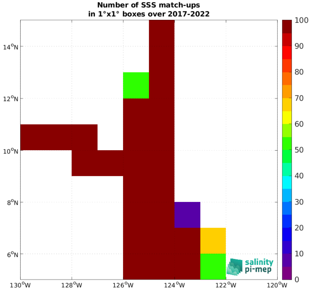
Figure 5: Number of SSS match-ups between Saildrone SSS and the SMAP SSS L3 v5.3 - 8-Day running (RSS) SSS product for the SPURS 2 Pi-MEP region over 1^\circ \times 1^\circ boxes and for the full satellite product period.
