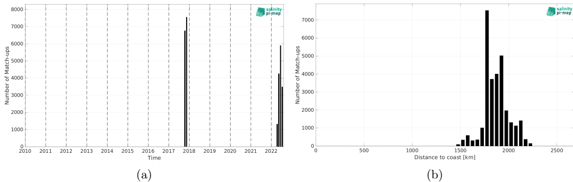
Figure 2: Number of match-ups between Saildrone and SMAP SSS L3 v5.3 - 8-Day running (RSS) SSS as a function of time (a) and as function of the distance to coast (b) over the SPURS 2 Pi-MEP region and for the full satellite product period.
