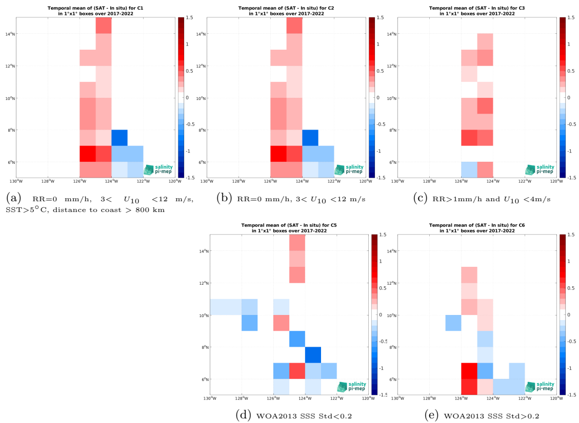
Figure 14: Temporal mean gridded over spatial boxes of size 1^\circ \times 1^\circ of \Delta SSS (SMAP SSS L3 v5.3 - 8-Day running (RSS) - Saildrone) for 5 different subdatasets corresponding to:RR=0 mm/h, 3 < U_{10} < 12 m/s, SST >5^\circ\text{C} , distance to coast > 800 km (a), RR=0 mm/h, 3 < U_{10} < 12 m/s (b), RR >1 mm/h and U_{10} < 4 m/s (c), WOA2013 SSS Std <0.2 (d), WOA2013 SSS Std >0.2 (e).
