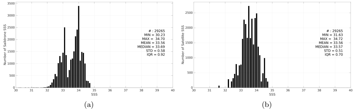
Figure 3: Histograms of SSS from Saildrone (a) and SMAP SSS L3 v5.3 - 8-Day running (RSS) (b) considering all match-up pairs per bins of 0.1 over the SPURS 2 Pi-MEP region and for the full satellite product period.
