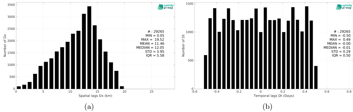
Figure 6: Histograms of the spatial (a) and temporal (b) lags between the location/time of the Sairdronne measurement and the date of the corresponding SMAP SSS L3 v5.3 - 8-Day running (RSS) SSS pixel.
