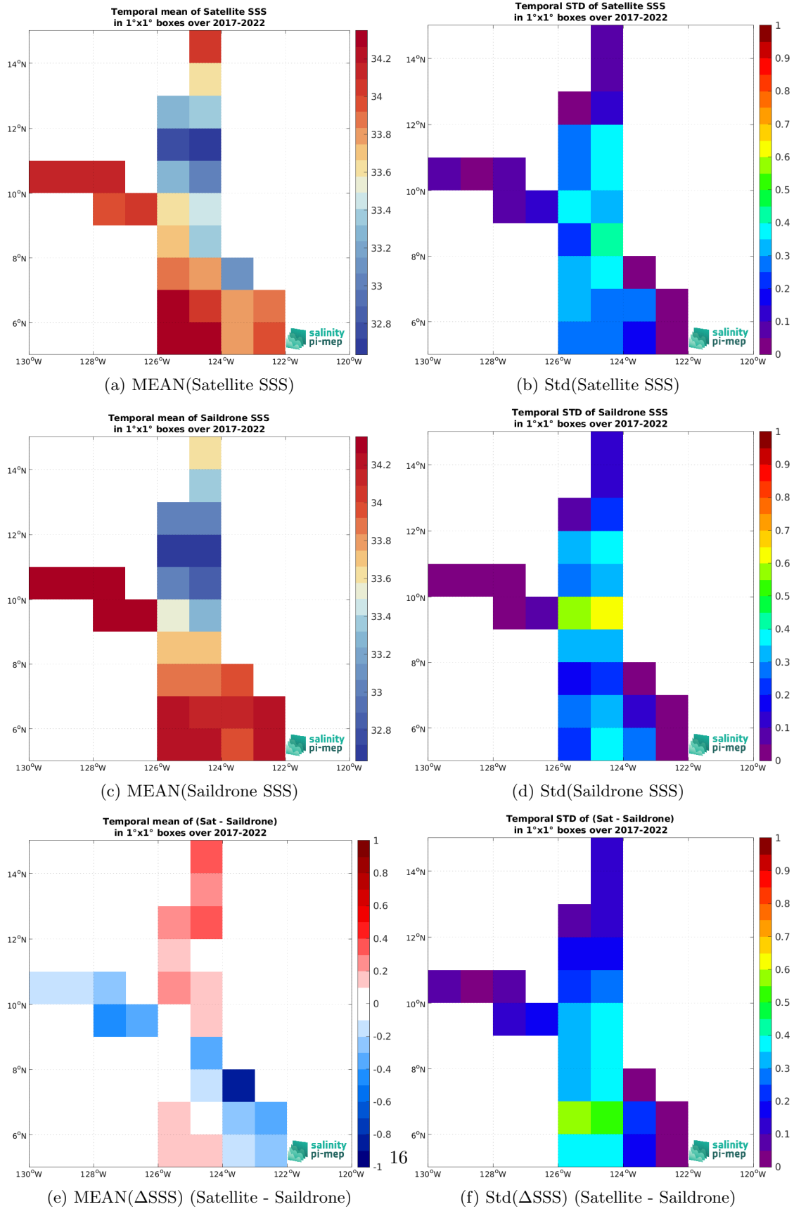
Figure 7: Temporal mean (left) and Std (right) of SSS from SMAP SSS L3 v5.3 - 8-Day running (RSS) (top), Saildrone (middle), and of \Delta SSS (Satellite - Saildrone). Only match-up pairs are used to generate these maps.
