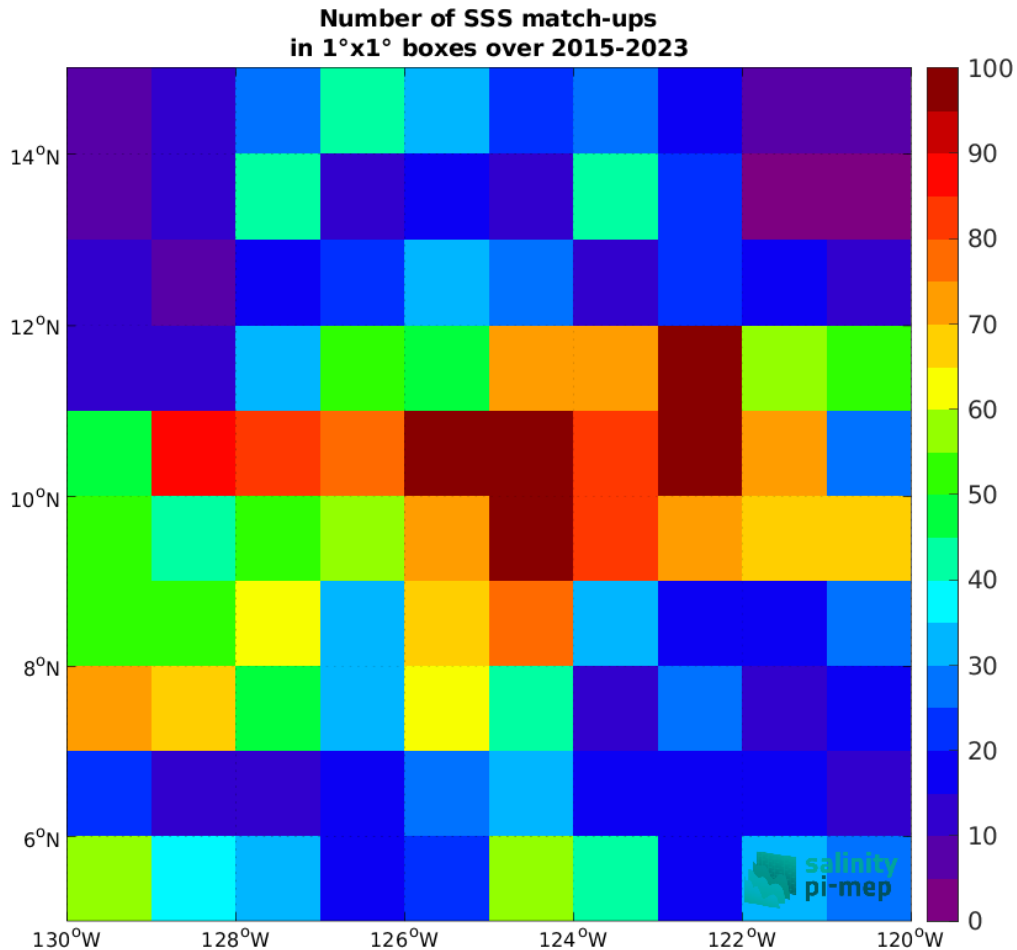
Figure 5: Number of SSS match-ups between Argo SSS and the SMAP SSS L3 v5.3 - 8-Day running (RSS) SSS product for the SPURS 2 Pi-MEP region over 1^\circ \times 1^\circ boxes and for the full satellite product period.
