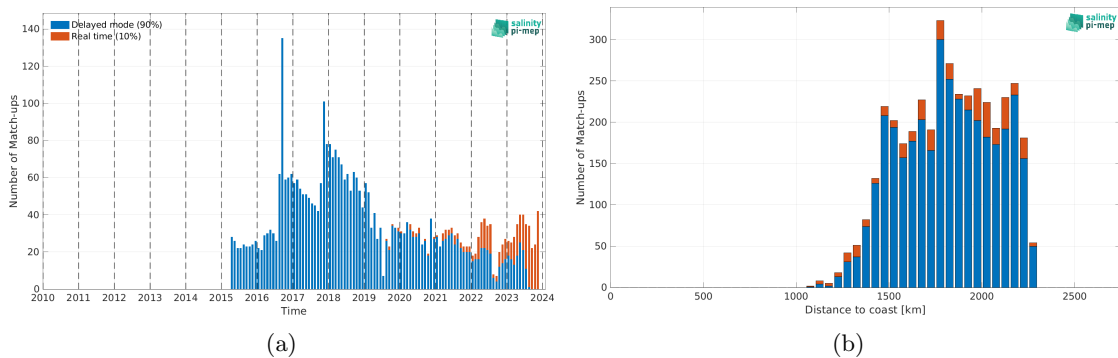
Figure 2: Number of match-ups between Argo and SMAP SSS L3 v5.3 - 8-Day running (RSS) SSS as a function of time (a) and as function of the distance to coast (b) over the SPURS 2 Pi-MEP region and for the full satellite product period.
