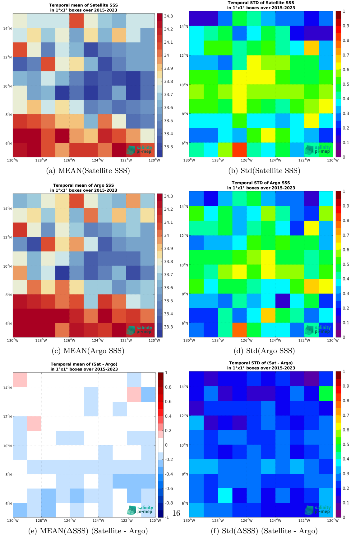
Figure 7: Temporal mean (left) and Std (right) of SSS from SMAP SSS L3 v5.3 - 8-Day running (RSS) (top), Argo (middle), and of \Delta SSS (Satellite - Argo). Only match-up pairs are used to generate these maps.
