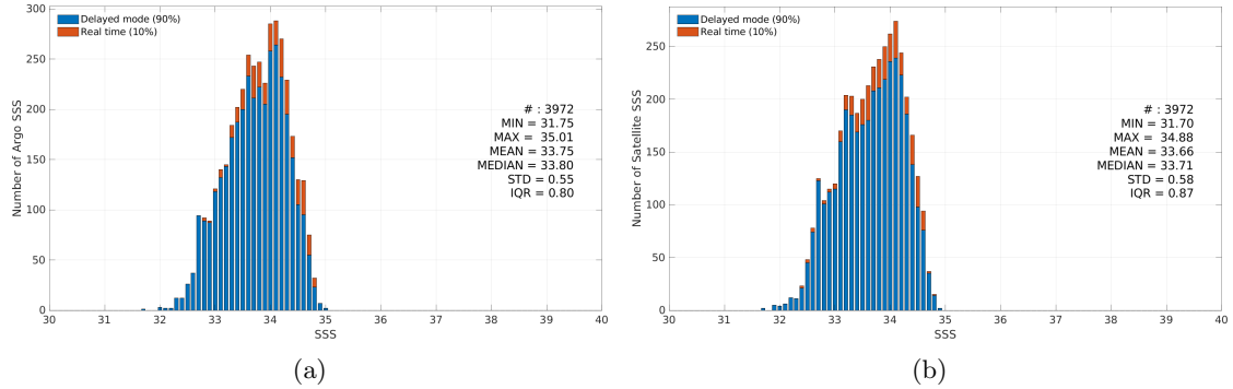
Figure 3: Histograms of SSS from Argo (a) and SMAP SSS L3 v5.3 - 8-Day running (RSS) (b) considering all match-up pairs per bins of 0.1 over the SPURS 2 Pi-MEP region and for the full satellite product period.
