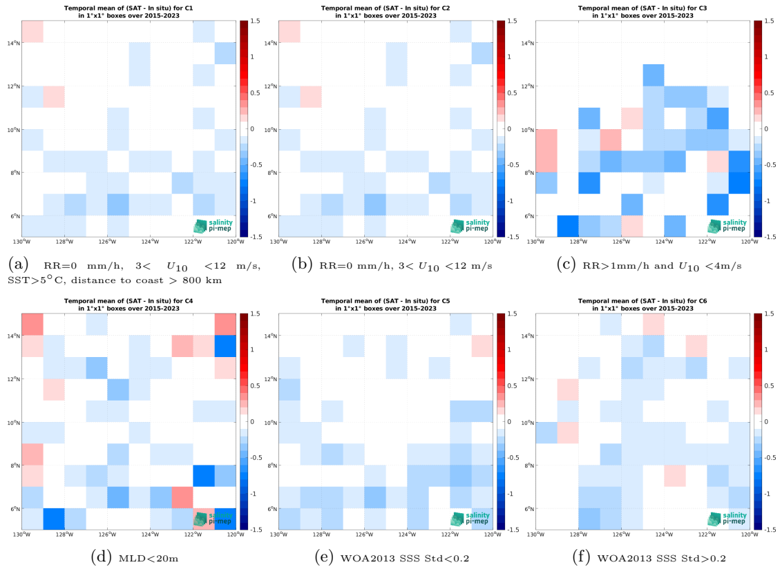
Figure 14: Temporal mean gridded over spatial boxes of size 1^\circ \times 1^\circ of \Delta SSS (SMAP SSS L3 v5.3 - 8-Day running (RSS) - Argo) for 6 different subdatasets corresponding to:RR=0 mm/h, 3 < U_{10} < 12 m/s, SST >5^\circ C, distance to coast > 800 km (a), RR=0 mm/h, 3 < U_{10} < 12 m/s (b), RR >1 mm/h and U_{10} < 4 m/s (c),MLD <20 m (d),WOA2013 SSS Std <0.2 (e),WOA2013 SSS Std >0.2 (f).
