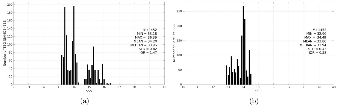
Figure 3: Histograms of SSS from TSG (SAMOS) (a) and SMAP SSS L3 v5.3 - Monthly (RSS) (b) considering all match-up pairs per bins of 0.1 over the SPURS 2 Pi-MEP region and for the full satellite product period.
