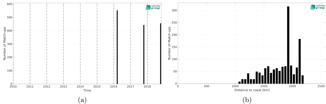
Figure 2: Number of match-ups between TSG (SAMOS) and SMAP SSS L3 v5.3 - Monthly (RSS) SSS as a function of time (a) and as function of the distance to coast (b) over the SPURS 2 Pi-MEP region and for the full satellite product period.
