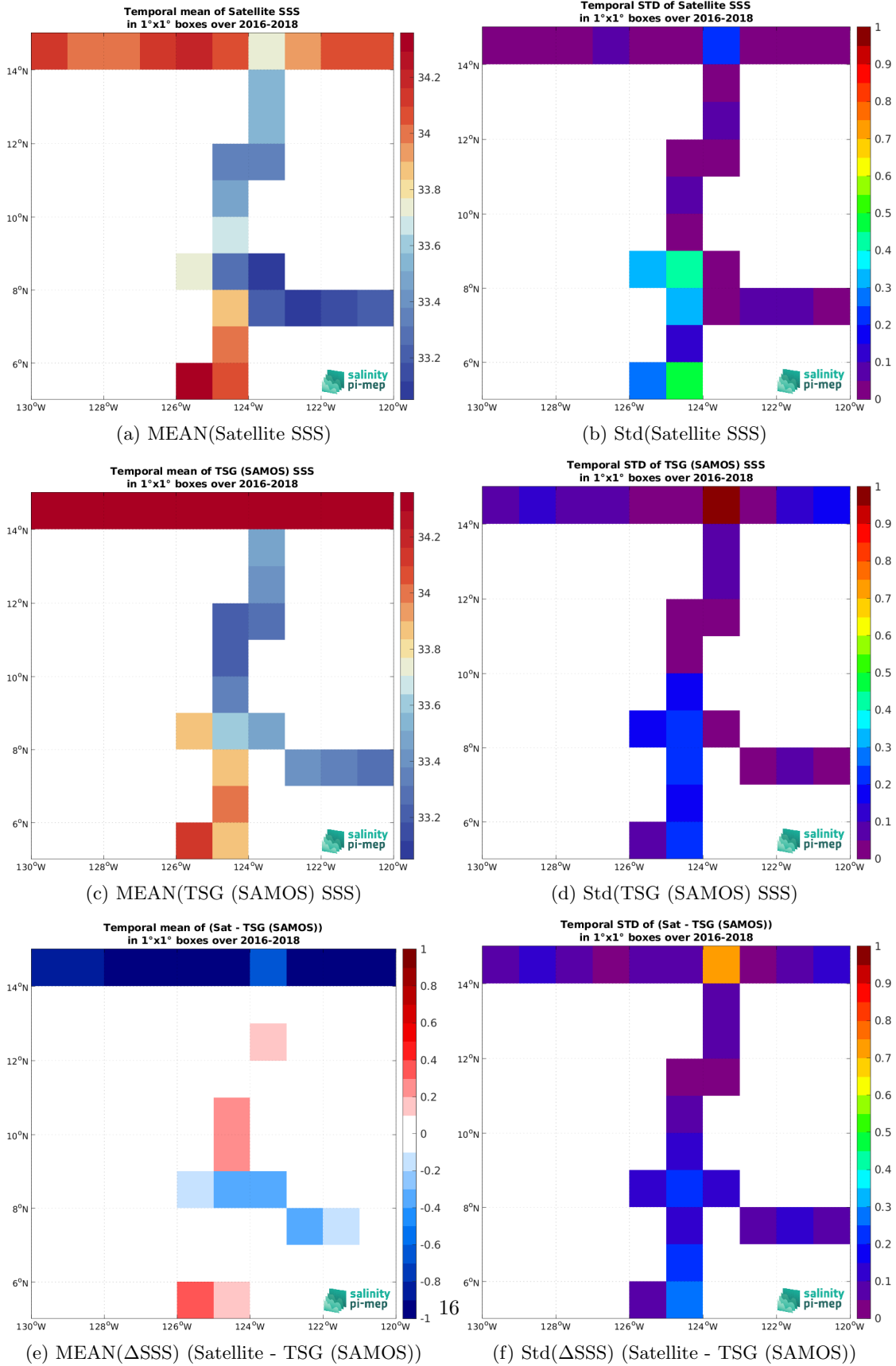
Figure 7: Temporal mean (left) and Std (right) of SSS from SMAP SSS L3 v5.3 - Monthly (RSS) (top), TSG (SAMOS) (middle), and of \Delta SSS (Satellite - TSG (SAMOS)). Only match-up pairs are used to generate these maps.
