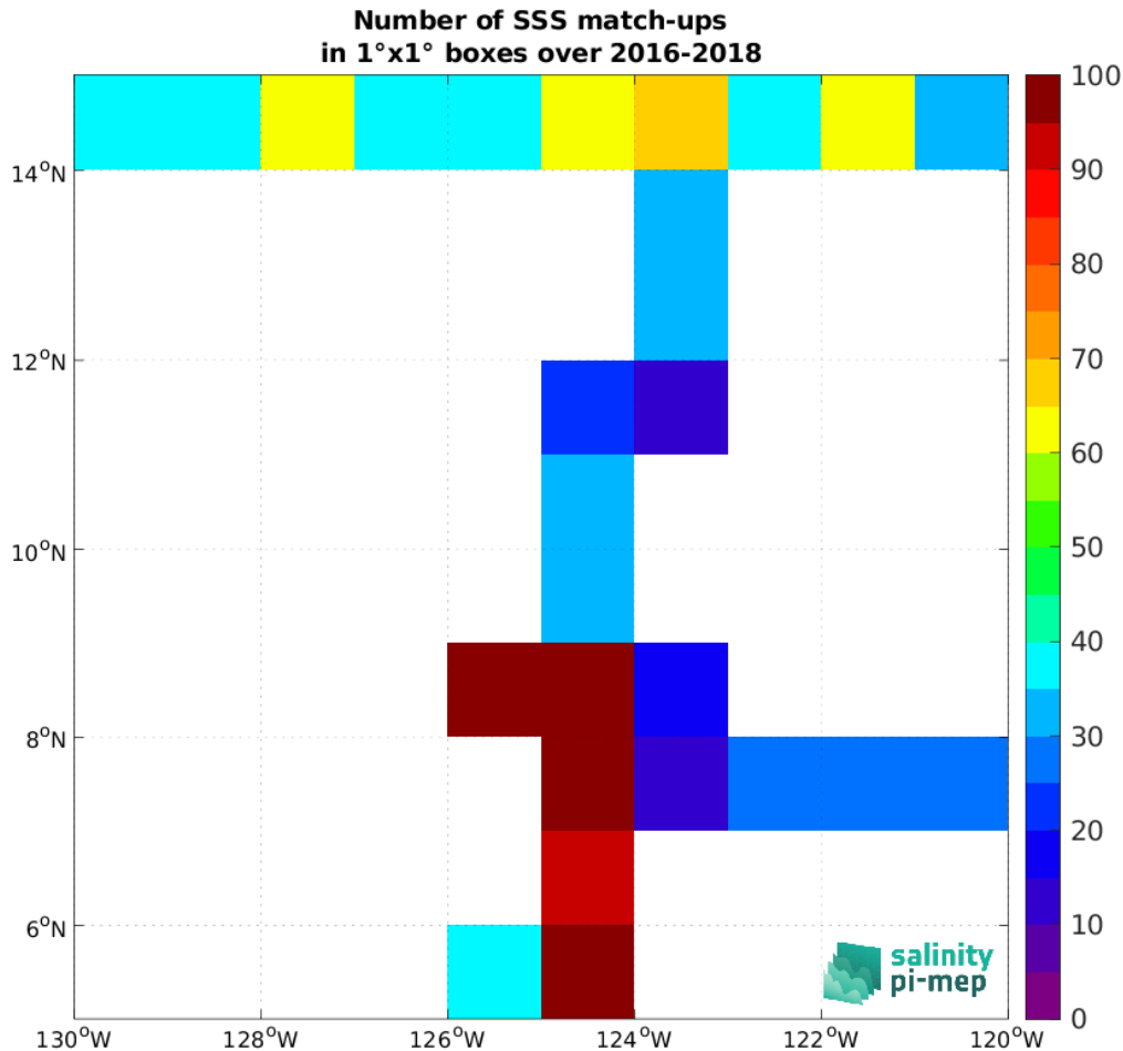
Figure 5: Number of SSS match-ups between TSG (SAMOS) SSS and the SMAP SSS L3 v5.3 - Monthly (RSS) SSS product for the SPURS 2 Pi-MEP region over 1^\circ \times 1^\circ boxes and for the full satellite product period.
