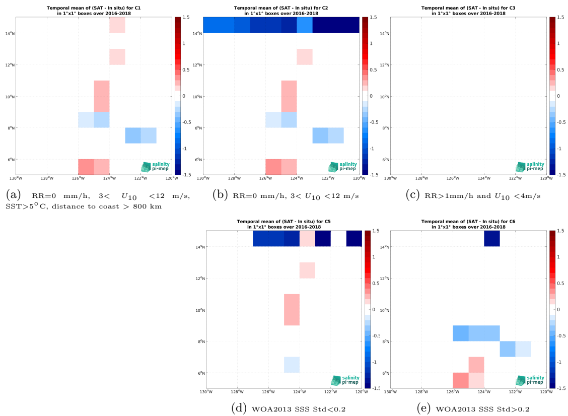
Figure 14: Temporal mean gridded over spatial boxes of size 1^\circ \times 1^\circ of \Delta\text{SSS} (SMAP SSS L3 v5.3 - Monthly (RSS) - TSG (SAMOS)) for 5 different subdatasets corresponding to:RR=0 mm/h, 3 < U_{10} < 12 m/s, SST>5°C, distance to coast > 800 km (a), RR=0 mm/h, 3 < U_{10} < 12 m/s (b), RR>1mm/h and U_{10} < 4 m/s (c), WOA2013 SSS Std<0.2 (d), WOA2013 SSS Std>0.2 (e).
