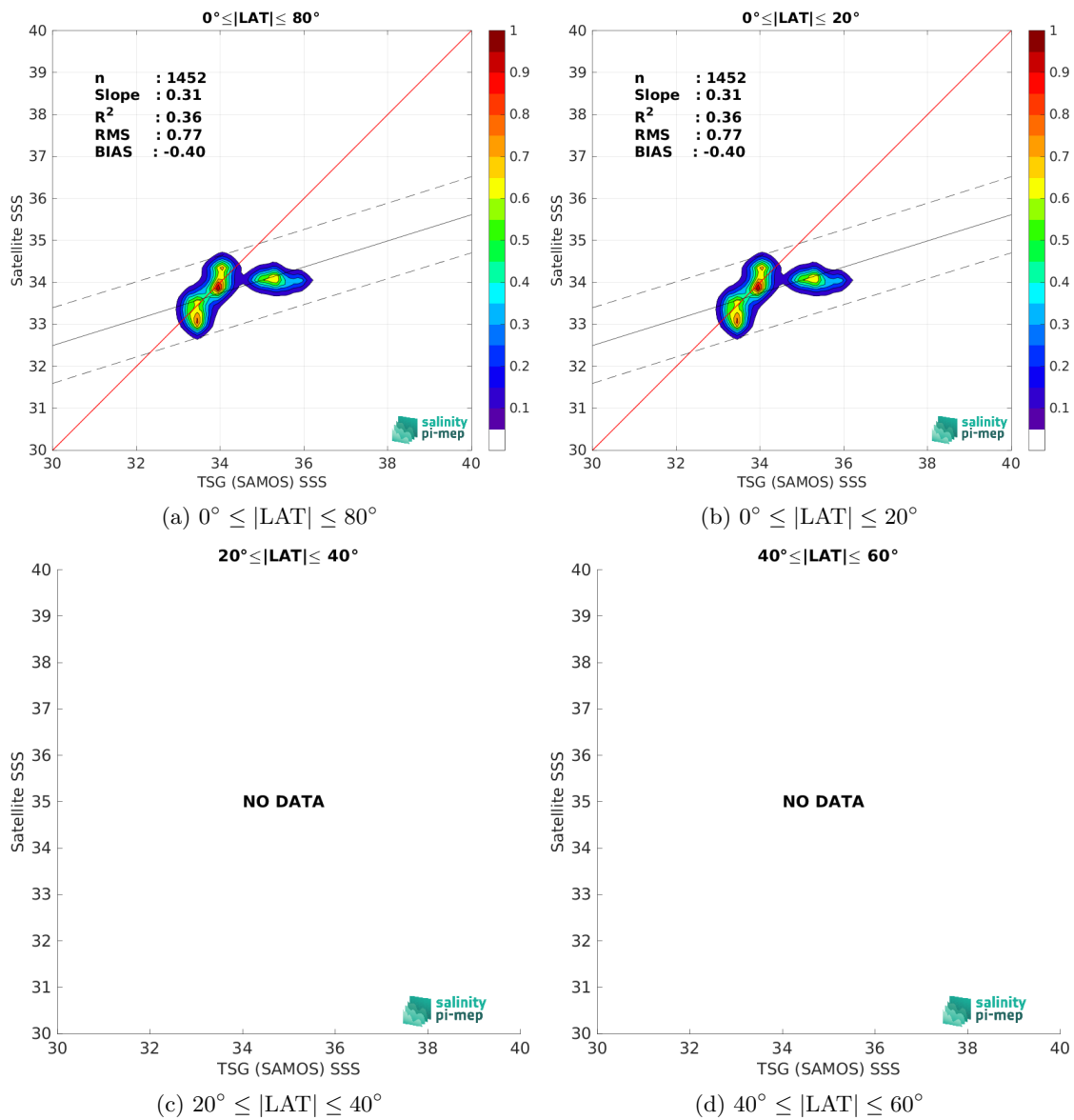
Figure 10: Contour maps of the concentration of SMAP SSS L3 v5.3 - Monthly (RSS) SSS (y-axis) versus TSG (SAMOS) SSS (x-axis) at match-up pairs for different latitude bands. For each plot, the red line shows x=y . The black thin and dashed lines indicate a linear fit through the data cloud and the \pm 95\% confidence levels, respectively. The number match-up pairs n , the slope and R^2 coefficient of the linear fit, the root mean square (RMS) and the mean bias between satellite and in situ data are indicated for each latitude band in each plots.
