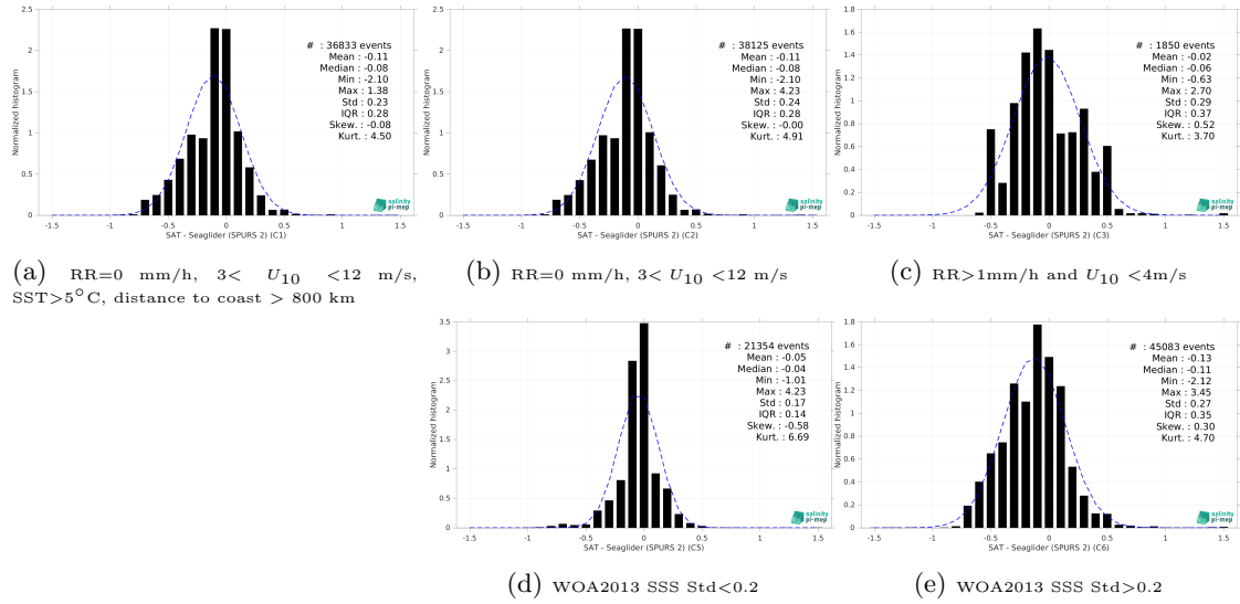
Figure 15: Normalized histogram of \Delta SSS (SMAP SSS L3 v5.3 - Monthly (RSS) - Seaglider (SPURS 2)) for 5 different subdatasets corresponding to: RR=0 mm/h, 3 < U_{10} < 12 m/s, SST > 5°C, distance to coast > 800 km (a), RR=0 mm/h, 3 < U_{10} < 12 m/s (b), RR > 1mm/h and U_{10} < 4 m/s (c), WOA2013 SSS Std < 0.2 (d), WOA2013 SSS Std > 0.2 (e).
