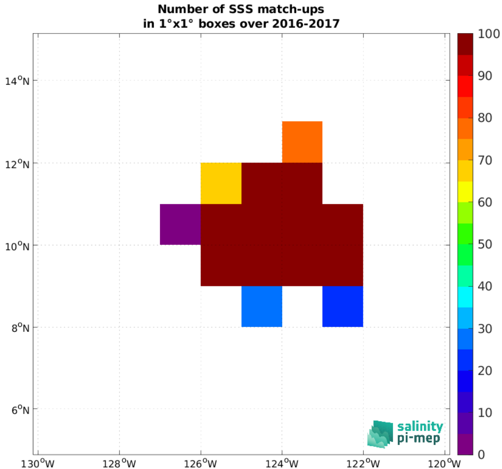
Figure 5: Number of SSS match-ups between Seaglider (SPURS 2) SSS and the SMAP SSS L3 v5.3 - Monthly (RSS) SSS product for the SPURS 2 Pi-MEP region over 1^\circ \times 1^\circ boxes and for the full satellite product period.
