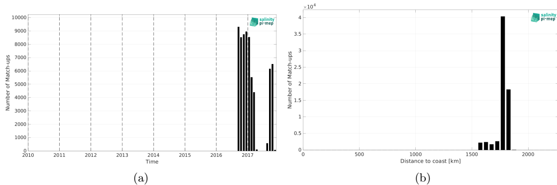
Figure 2: Number of match-ups between Seaglider (SPURS 2) and SMAP SSS L3 v5.3 - Monthly (RSS) SSS as a function of time (a) and as function of the distance to coast (b) over the SPURS 2 Pi-MEP region and for the full satellite product period.
