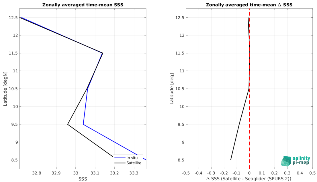
Figure 9: Left panel: Zonal mean SSS from SMAP SSS L3 v5.3 - Monthly (RSS) satellite product (black) and from Seaglider (SPURS 2) (blue). Right panel: Zonal mean of \Delta SSS (Satellite - Seaglider (SPURS 2)) for all the collected Pi-MEP match-up pairs estimated over the full satellite product period.
