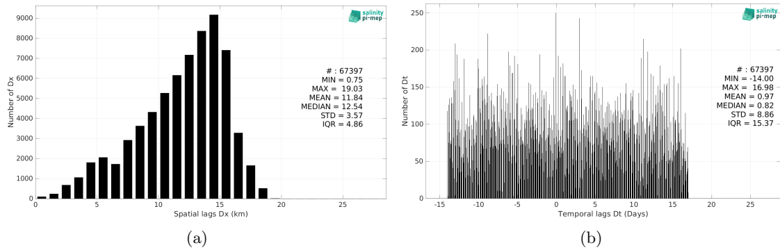
Figure 6: Histograms of the spatial (a) and temporal (b) lags between the location/time of the Seaglider (SPURS 2) measurement and the date of the corresponding SMAP SSS L3 v5.3 - Monthly (RSS) SSS pixel.
