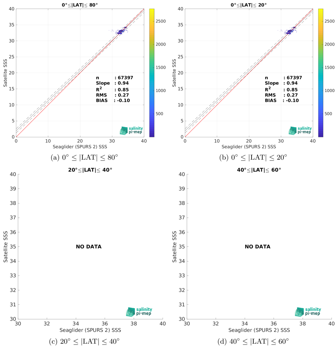
Figure 10: Contour maps of the concentration of SMAP SSS L3 v5.3 - Monthly (RSS) SSS (y-axis) versus Seaglider (SPURS 2) SSS (x-axis) at match-up pairs for different latitude bands. For each plot, the red line shows x=y . The black thin and dashed lines indicate a linear fit through the data cloud and the \pm 95\% confidence levels, respectively. The number match-up pairs n , the slope and R^2 coefficient of the linear fit, the root mean square (RMS) and the mean bias between satellite and in situ data are indicated for each latitude band in each plots.
