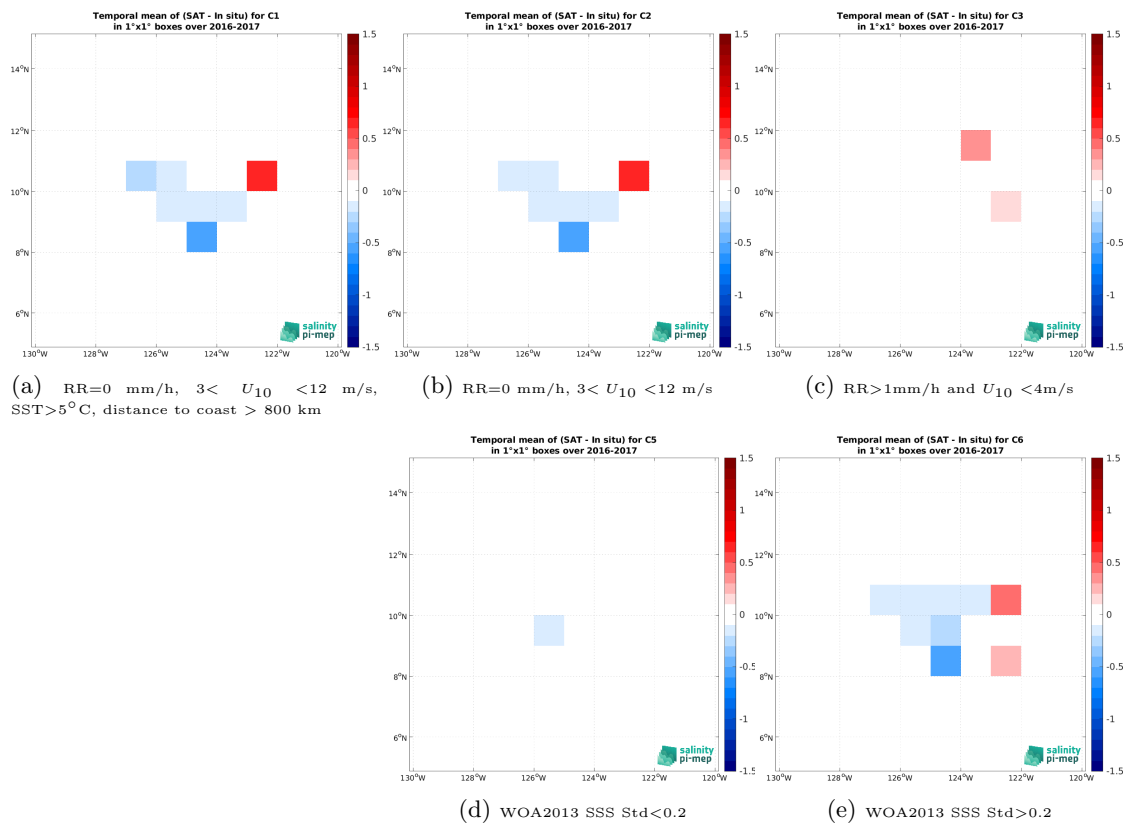
Figure 14: Temporal mean gridded over spatial boxes of size 1^\circ \times 1^\circ of \Delta SSS (SMAP SSS L3 v5.3 - Monthly (RSS) - Seaglider (SPURS 2)) for 5 different subdatasets corresponding to:RR=0 mm/h, 3 < U_{10} < 12 m/s, SST>5°C, distance to coast > 800 km (a), RR=0 mm/h, 3 < U_{10} < 12 m/s (b), RR>1mm/h and U_{10} < 4 m/s (c), WOA2013 SSS Std<0.2 (d), WOA2013 SSS Std>0.2 (e).
