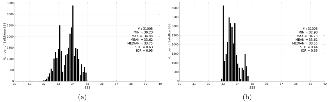
Figure 3: Histograms of SSS from Saildrone (a) and SMAP SSS L3 v5.3 - Monthly (RSS) (b) considering all match-up pairs per bins of 0.1 over the SPURS 2 Pi-MEP region and for the full satellite product period.
