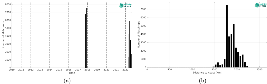
Figure 2: Number of match-ups between Saildrone and SMAP SSS L3 v5.3 - Monthly (RSS) SSS as a function of time (a) and as function of the distance to coast (b) over the SPURS 2 Pi-MEP region and for the full satellite product period.
