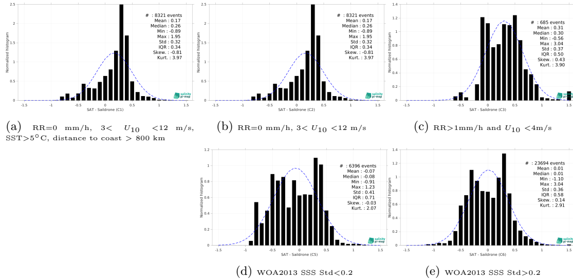
Figure 15: Normalized histogram of \Delta SSS (SMAP SSS L3 v5.3 - Monthly (RSS) - Salldrone) for 5 different subdatasets corresponding to: RR=0 mm/h, 3 < U_{10} < 12 m/s, SST > 5°C, distance to coast > 800 km (a), RR=0 mm/h, 3 < U_{10} < 12 m/s (b), RR > 1mm/h and U_{10} < 4 m/s (c), WOA2013 SSS Std < 0.2 (d), WOA2013 SSS Std > 0.2 (e).
