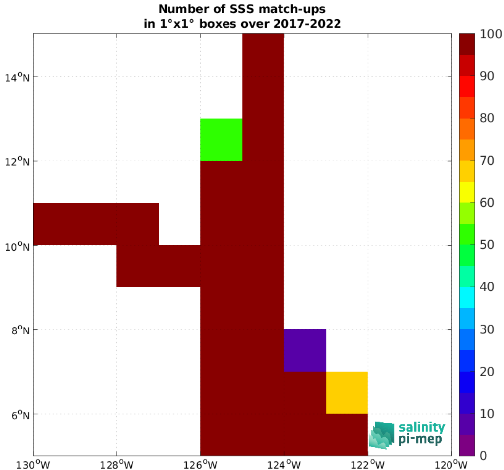
Figure 5: Number of SSS match-ups between Saildrone SSS and the SMAP SSS L3 v5.3 - Monthly (RSS) SSS product for the SPURS 2 Pi-MEP region over 1^\circ \times 1^\circ boxes and for the full satellite product period.
