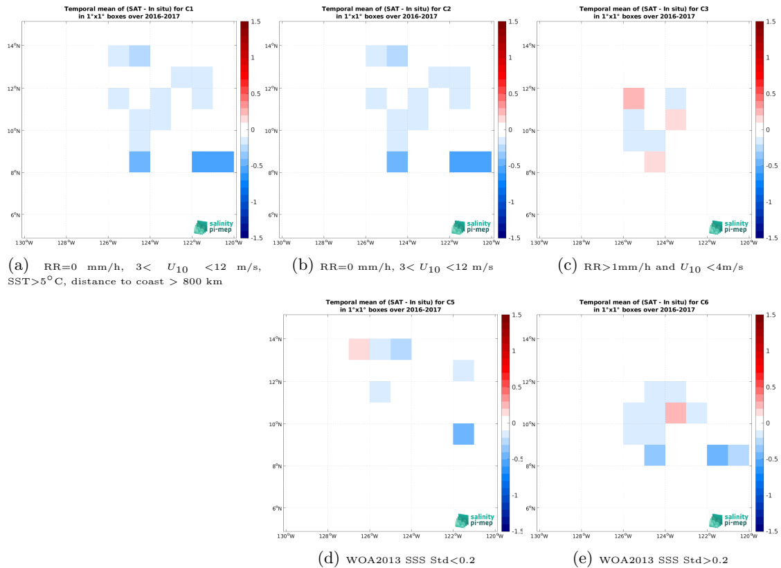
Figure 12: Temporal mean gridded over spatial boxes of size 1^\circ \times 1^\circ of \Delta SSS (SMAP SSS L3 v5 - 8-Day running (RSS) - Waveglider (SPURS 2)) for 5 different subdatasets corresponding to: RR=0 mm/h, 3 < U_{10} < 12 m/s, SST > 5^\circ\text{C} , distance to coast > 800 km (a), RR=0 mm/h, 3 < U_{10} < 12 m/s (b), RR > 1 mm/h and U_{10} < 4 m/s (c), WOA2013 SSS Std < 0.2 (d), WOA2013 SSS Std > 0.2 (e).
