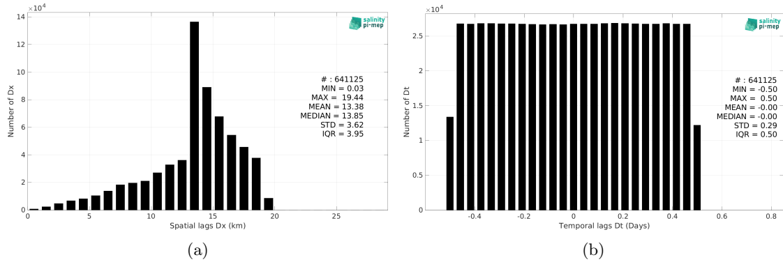
Figure 5: Histograms of the spatial (a) and temporal (b) lags between the location/time of the Waveglider (SPURS 2) measurement and the date of the corresponding SMAP SSS L3 v5 - 8-Day running (RSS) SSS pixel.
