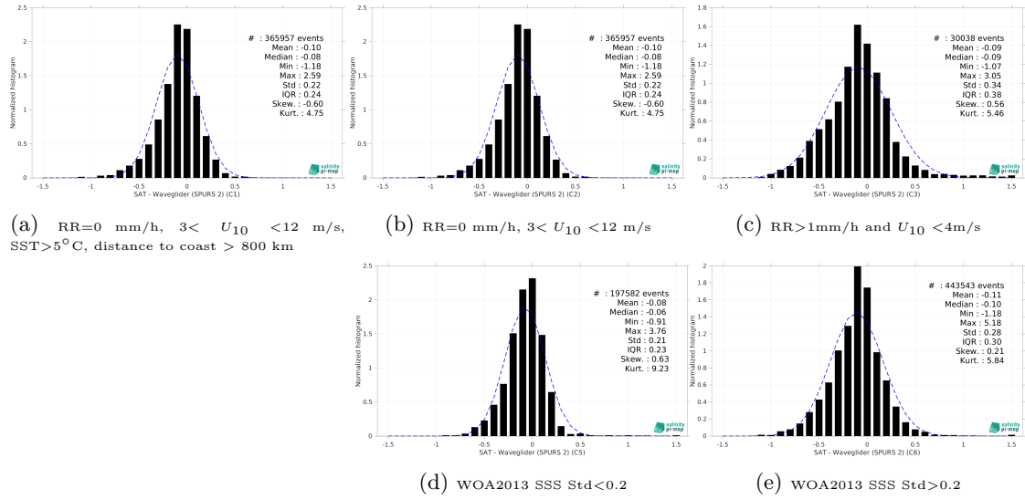
Figure 13: Normalized histogram of \Delta\text{SSS} (SMAP SSS L3 v5 - 8-Day running (RSS) - Waveglider (SPURS 2)) for 5 different subdatasets corresponding to: RR=0 mm/h, 3 < U_{10} < 12 m/s, SST >5^{\circ}\text{C} , distance to coast > 800 km (a), RR=0 mm/h, 3 < U_{10} < 12 m/s (b), RR >1 mm/h and U_{10} < 4 m/s (c), WOA2013 SSS Std <0.2 (d), WOA2013 SSS Std >0.2 (e).
