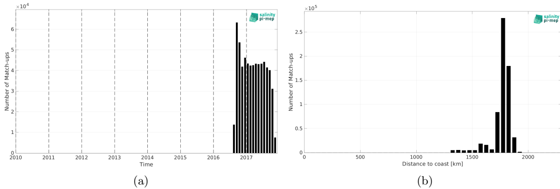
Figure 1: Number of match-ups between Waveglider (SPURS 2) and SMAP SSS L3 v5 - 8-Day running (RSS) SSS as a function of time (a) and as function of the distance to coast (b) over the SPURS 2 Pi-MEP region and for the full satellite product period.
