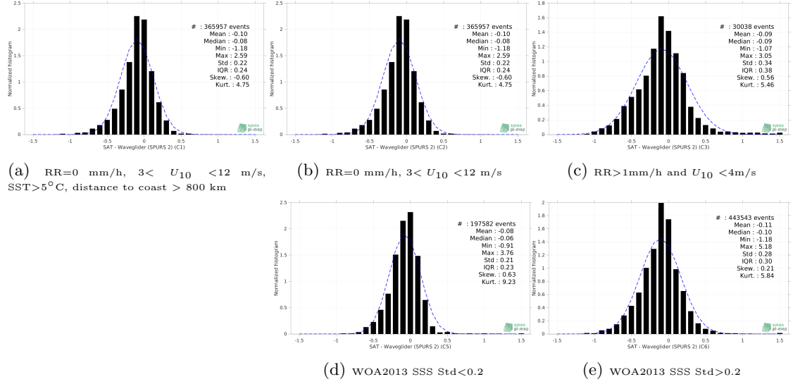
Figure 13: Normalized histogram of \Delta\text{SSS} (SMAP SSS L3 v5 - 8-Day running (RSS) - Waveglider (SPURS 2)) for 5 different subdatasets corresponding to: RR=0 mm/h, 3 < U_{10} < 12 m/s, SST >5^{\circ}\text{C} , distance to coast > 800 km (a), RR=0 mm/h, 3 < U_{10} < 12 m/s (b), RR >1 mm/h and U_{10} < 4 m/s (c), WOA2013 SSS Std <0.2 (d), WOA2013 SSS Std >0.2 (e).
