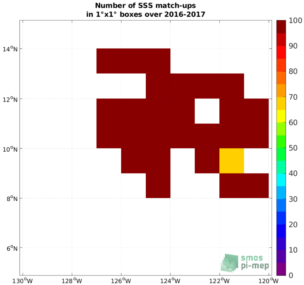
Figure 4: Number of SSS match-ups between Waveglider (SPURS 2) SSS and the SMAP SSS L3 v5 - 8-Day running (RSS) SSS product for the SPURS 2 Pi-MEP region over 1^{\circ} \times 1^{\circ} boxes and for the full satellite product period.
