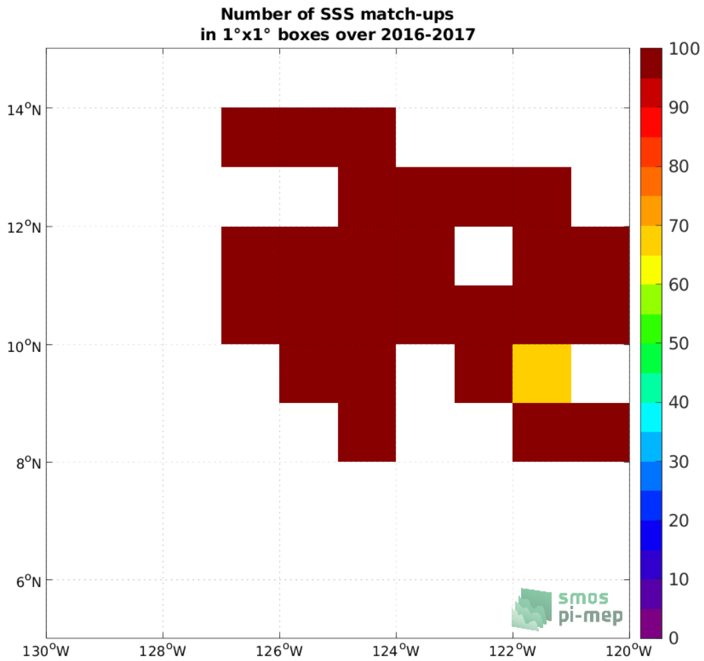
Figure 4: Number of SSS match-ups between Waveglider SSS and the SMAP SSS L3 v5 - 8-Day running (RSS) SSS product for the SPURS 2 Pi-MEP region over 1°×1° boxes and for the full satellite product period.
