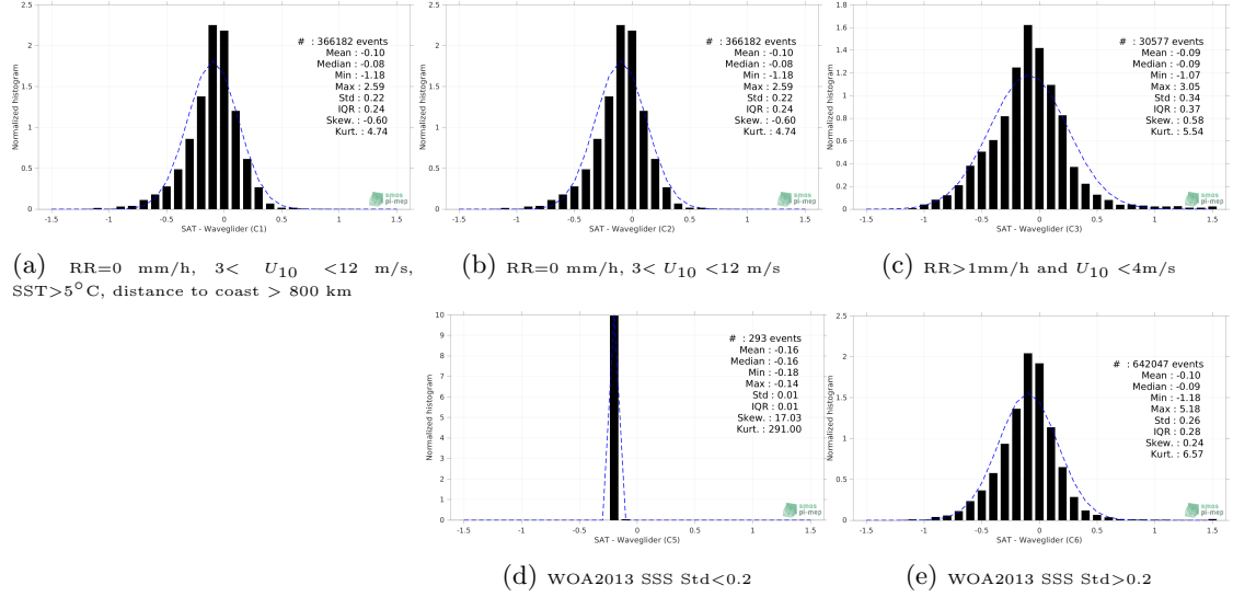
Figure 13: Normalized histogram of \Delta SSS (SMAP SSS L3 v5 - 8-Day running (RSS) - Waveglider) for 5 different subdatasets corresponding to: RR=0 mm/h, 3 < U_{10} < 12 m/s, SST > 5°C, distance to coast > 800 km (a), RR=0 mm/h, 3 < U_{10} < 12 m/s (b), RR > 1mm/h and U_{10} < 4 m/s (c), WOA2013 SSS Std < 0.2 (d), WOA2013 SSS Std > 0.2 (e).
