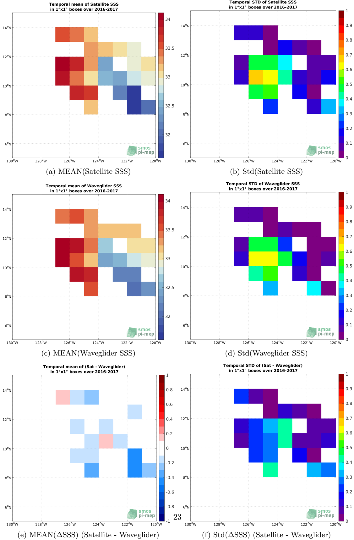
Figure 6: Temporal mean (left) and Std (right) of SSS from SMAP SSS L3 v5 - 8-Day running (RSS) (top), Waveglider (middle), and of \Delta SSS (Satellite - Waveglider). Only match-up pairs are used to generate these maps.
