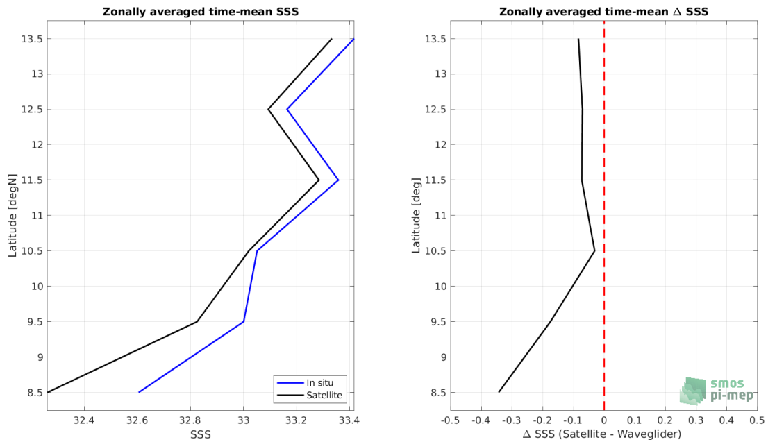
Figure 8: Left panel: Zonal mean SSS from SMAP SSS L3 v5 - 8-Day running (RSS) satellite product (black) and from Waveglider (blue). Right panel: Zonal mean of \Delta SSS (Satellite - Waveglider) for all the collected Pi-MEP match-up pairs estimated over the full satellite product period.
