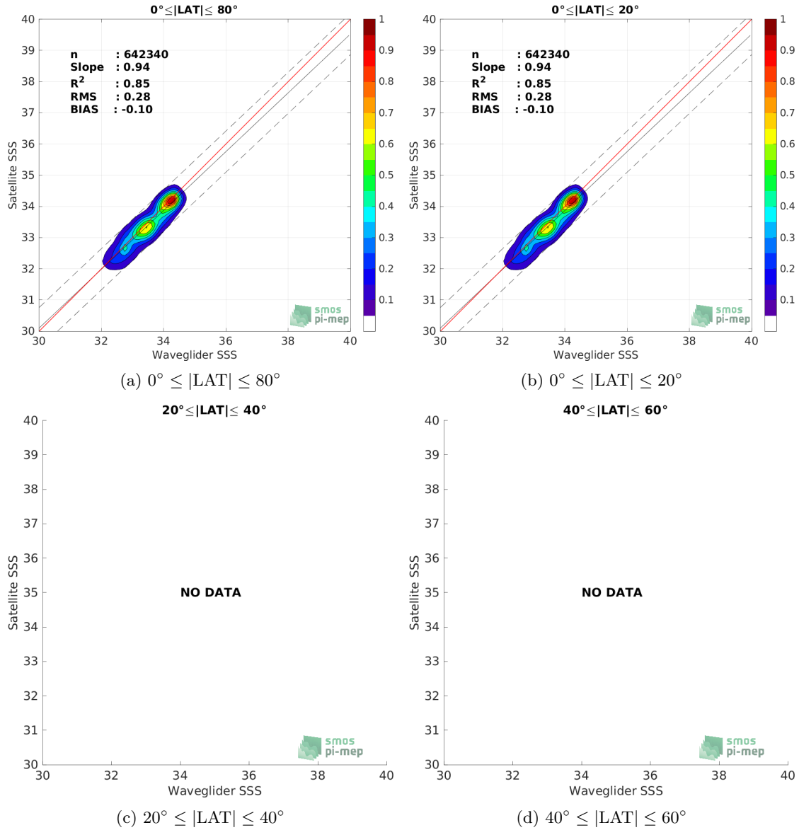
Figure 9: Contour maps of the concentration of SMAP SSS L3 v5 - 8-Day running (RSS) SSS (y-axis) versus Waveglider SSS (x-axis) at match-up pairs for different latitude bands. For each plot, the red line shows x=y . The black thin and dashed lines indicate a linear fit through the data cloud and the \pm 95\% confidence levels, respectively. The number match-up pairs n , the slope and R^2 coefficient of the linear fit, the root mean square (RMS) and the mean bias between satellite and in situ data are indicated for each latitude band in each plots.
