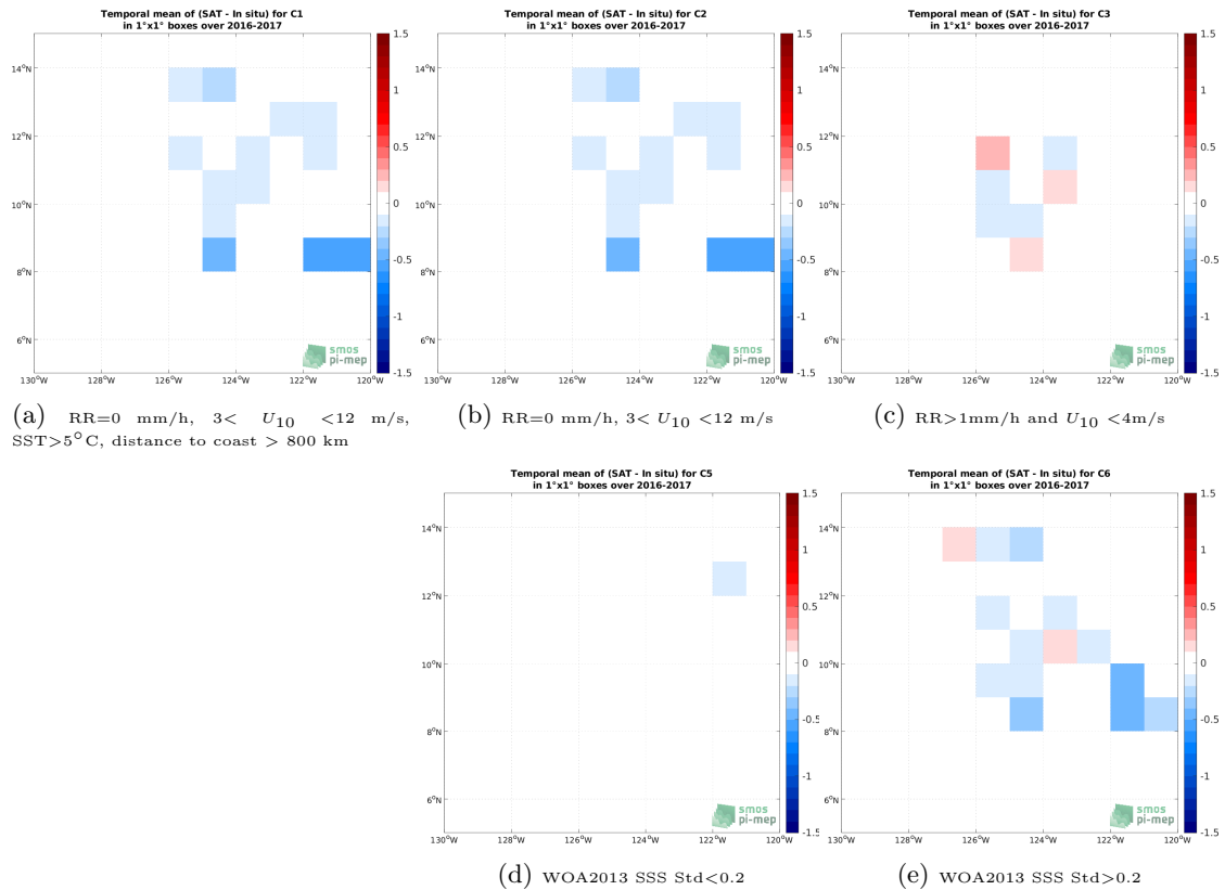
Figure 12: Temporal mean gridded over spatial boxes of size 1^\circ \times 1^\circ of \Delta\text{SSS} (SMAP SSS L3 v5 - 8-Day running (RSS) - Waveglider) for 5 different subdatasets corresponding to:RR=0 mm/h, 3 < U_{10} < 12 m/s, SST >5^\circ\text{C} , distance to coast > 800 km (a), RR=0 mm/h, 3 < U_{10} < 12 m/s (b), RR >1 mm/h and U_{10} < 4 m/s (c), WOA2013 SSS Std <0.2 (d), WOA2013 SSS Std >0.2 (e).
