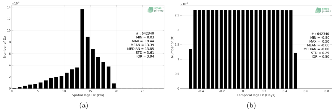
Figure 5: Histograms of the spatial (a) and temporal (b) lags between the location/time of the Waveglider measurement and the date of the corresponding SMAP SSS L3 v5 - 8-Day running (RSS) SSS pixel.
