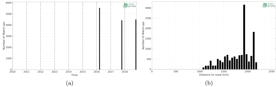
Figure 1: Number of match-ups between TSG (SAMOS) and SMAP SSS L3 v5 - 8-Day running (RSS) SSS as a function of time (a) and as function of the distance to coast (b) over the SPURS 2 Pi-MEP region and for the full satellite product period.
