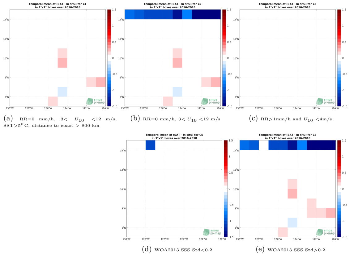
Figure 12: Temporal mean gridded over spatial boxes of size 1^\circ \times 1^\circ of \Delta\text{SSS} (SMAP SSS L3 v5 - 8-Day running (RSS) - TSG (SAMOS)) for 5 different subdatasets corresponding to:RR=0 mm/h, 3 < U_{10} < 12 m/s, SST >5^\circ\text{C} , distance to coast > 800 km (a), RR=0 mm/h, 3 < U_{10} < 12 m/s (b), RR >1 mm/h and U_{10} < 4 m/s (c), WOA2013 SSS Std <0.2 (d), WOA2013 SSS Std >0.2 (e).
