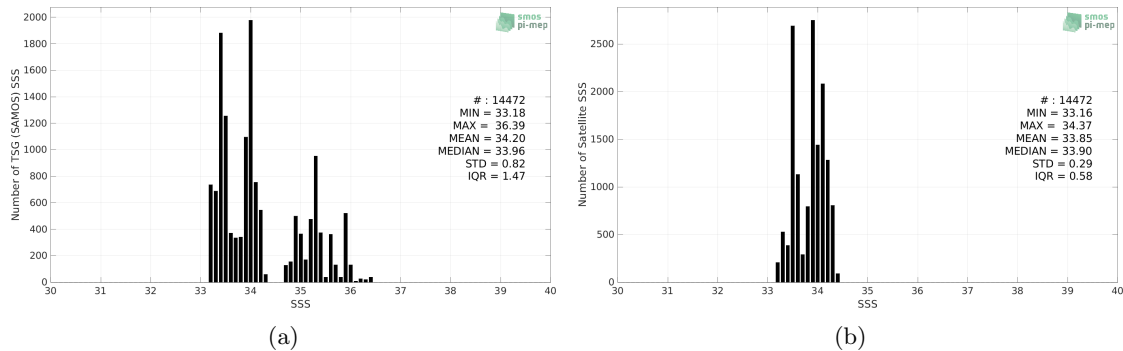
Figure 2: Histograms of SSS from TSG (SAMOS) (a) and SMAP SSS L3 v5 - 8-Day running (RSS) (b) considering all match-up pairs per bins of 0.1 over the SPURS 2 Pi-MEP region and for the full satellite product period.
