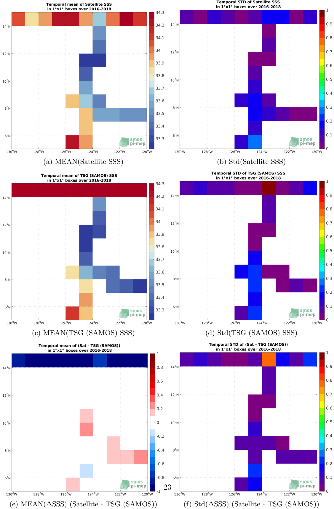
Figure 6: Temporal mean (left) and Std (right) of SSS from SMAP SSS L3 v5 - 8-Day running (RSS) (top), TSG (SAMOS) (middle), and of \Delta SSS (Satellite - TSG (SAMOS)). Only match-up pairs are used to generate these maps.
