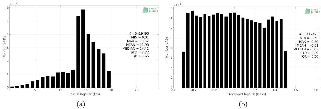
Figure 5: Histograms of the spatial (a) and temporal (b) lags between the location/time of the Salinity Snake (SPURS 2) measurement and the date of the corresponding SMAP SSS L3 v5 - 8-Day running (RSS) SSS pixel.
