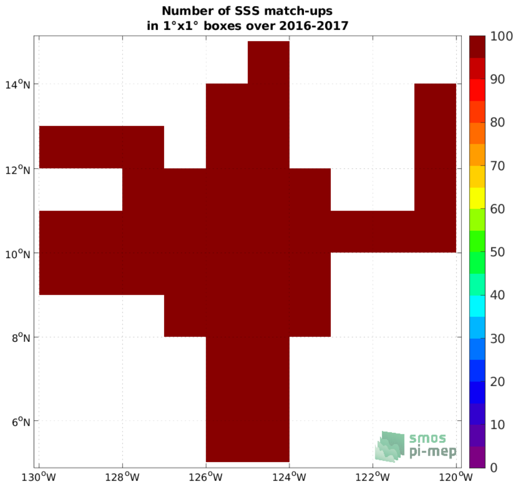
Figure 4: Number of SSS match-ups between Salinity Snake (SPURS 2) SSS and the SMAP SSS L3 v5 - 8-Day running (RSS) SSS product for the SPURS 2 Pi-MEP region over 1°x1° boxes and for the full satellite product period.
