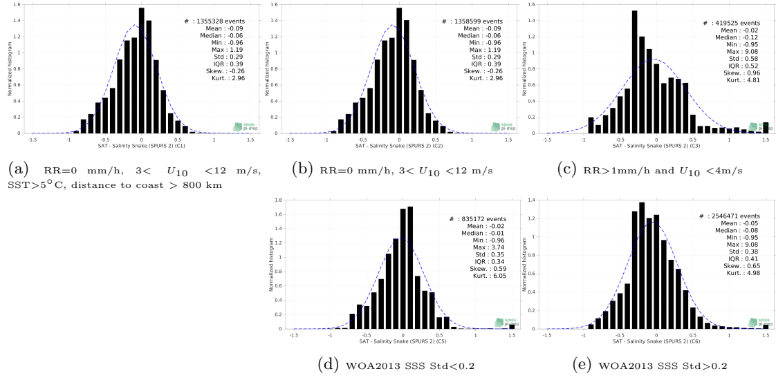
Figure 13: Normalized histogram of \Delta SSS (SMAP SSS L3 v5 - 8-Day running (RSS) - Salinity Snake (SPURS 2)) for 5 different subdatasets corresponding to: RR=0 mm/h, 3 < U_{10} < 12 m/s, SST>5°C, distance to coast > 800 km (a), RR=0 mm/h, 3 < U_{10} < 12 m/s (b), RR>1mm/h and U_{10} < 4 m/s (c), WOA2013 SSS Std<0.2 (d), WOA2013 SSS Std>0.2 (e).
