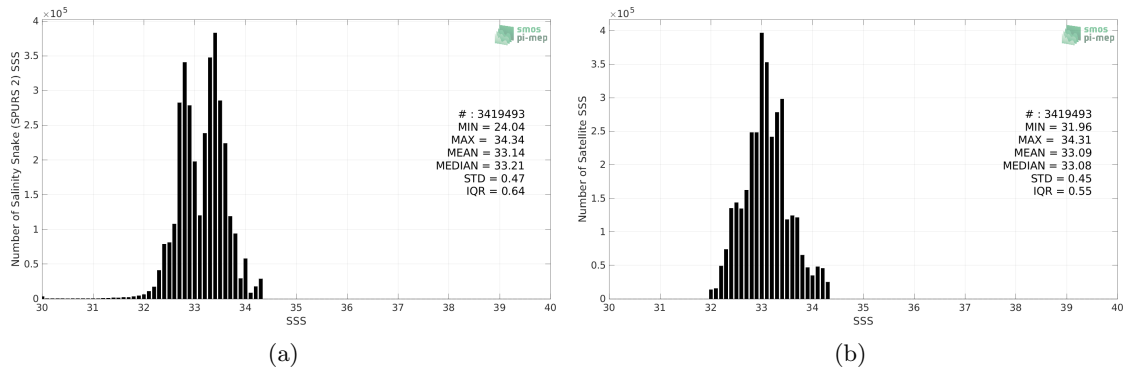
Figure 2: Histograms of SSS from Salinity Snake (SPURS 2) (a) and SMAP SSS L3 v5 - 8-Day running (RSS) (b) considering all match-up pairs per bins of 0.1 over the SPURS 2 Pi-MEP region and for the full satellite product period.
