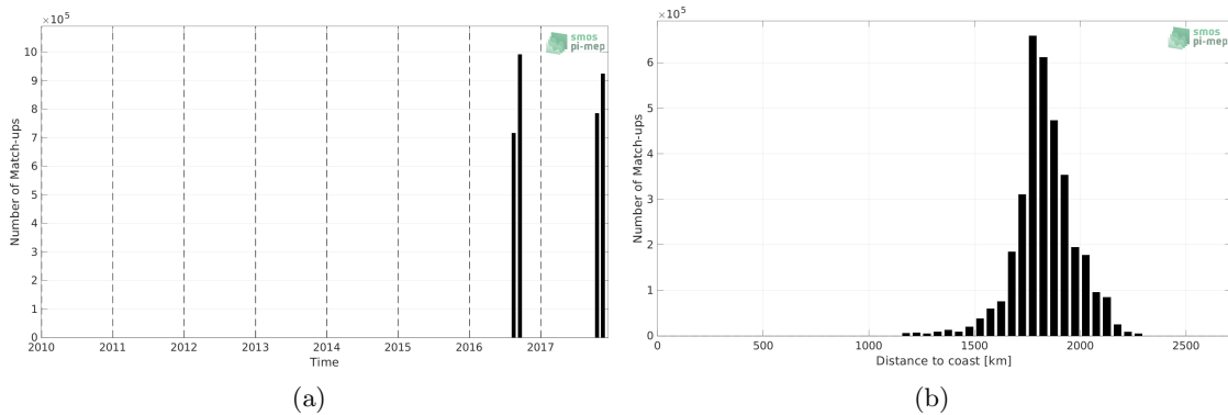
Figure 1: Number of match-ups between Salinity Snake (SPURS 2) and SMAP SSS L3 v5 - 8-Day running (RSS) SSS as a function of time (a) and as function of the distance to coast (b) over the SPURS 2 Pi-MEP region and for the full satellite product period.
