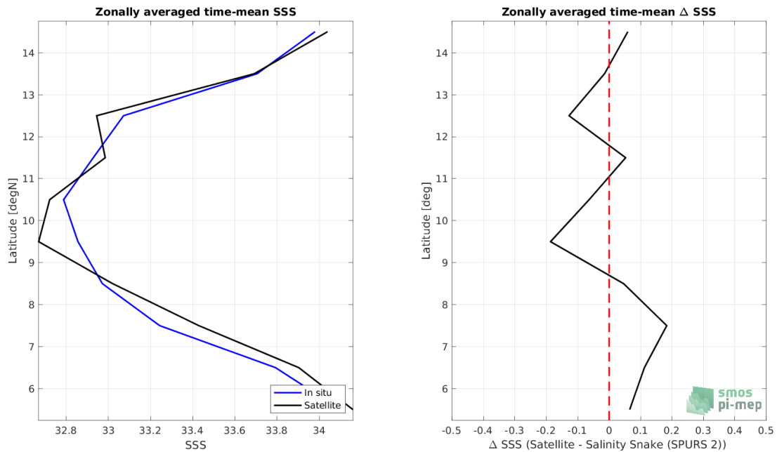
Figure 8: Left panel: Zonal mean SSS from SMAP SSS L3 v5 - 8-Day running (RSS) satellite product (black) and from Salinity Snake (SPURS 2) (blue). Right panel: Zonal mean of \Delta SSS (Satellite - Salinity Snake (SPURS 2)) for all the collected Pi-MEP match-up pairs estimated over the full satellite product period.
