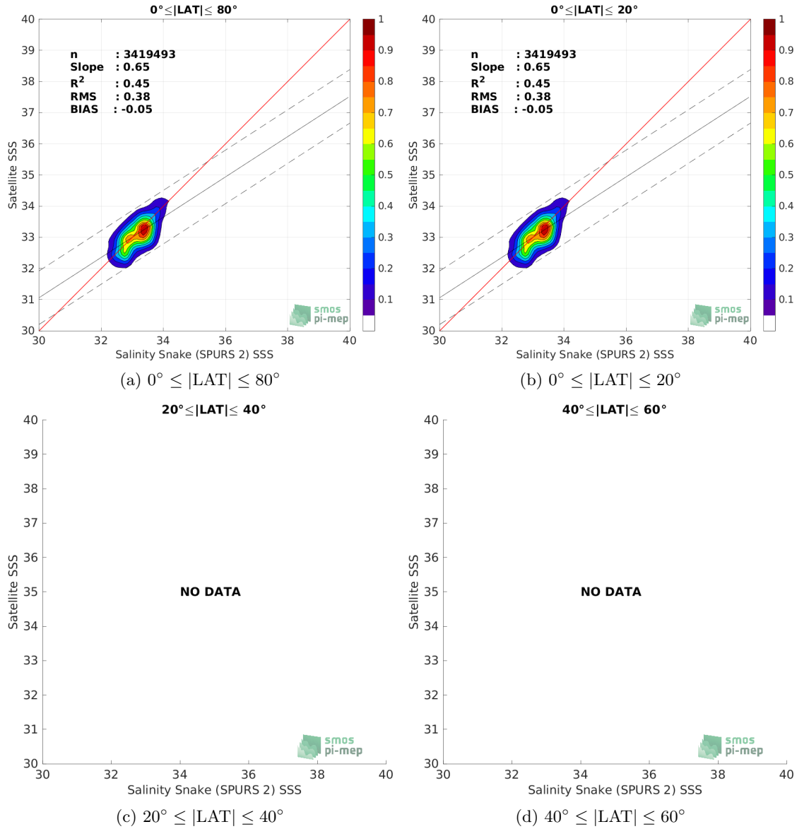
Figure 9: Contour maps of the concentration of SMAP SSS L3 v5 - 8-Day running (RSS) SSS (y-axis) versus Salinity Snake (SPURS 2) SSS (x-axis) at match-up pairs for different latitude bands. For each plot, the red line shows x=y . The black thin and dashed lines indicate a linear fit through the data cloud and the \pm 95\% confidence levels, respectively. The number match-up pairs n , the slope and R^2 coefficient of the linear fit, the root mean square (RMS) and the mean bias between satellite and in situ data are indicated for each latitude band in each plots.
