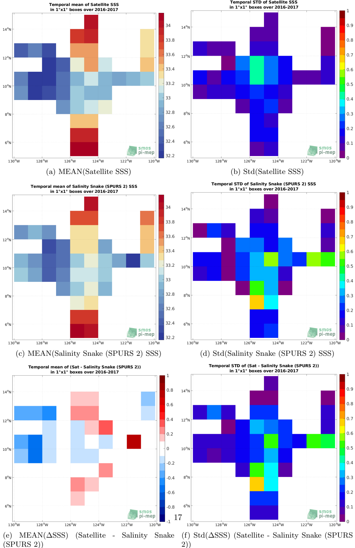
Figure 6: Temporal mean (left) and Std (right) of SSS from SMAP SSS L3 v5 - 8-Day running (RSS) (top), Salinity Snake (SPURS 2) (middle), and of \Delta SSS (Satellite - Salinity Snake (SPURS 2)). Only match-up pairs are used to generate these maps.
