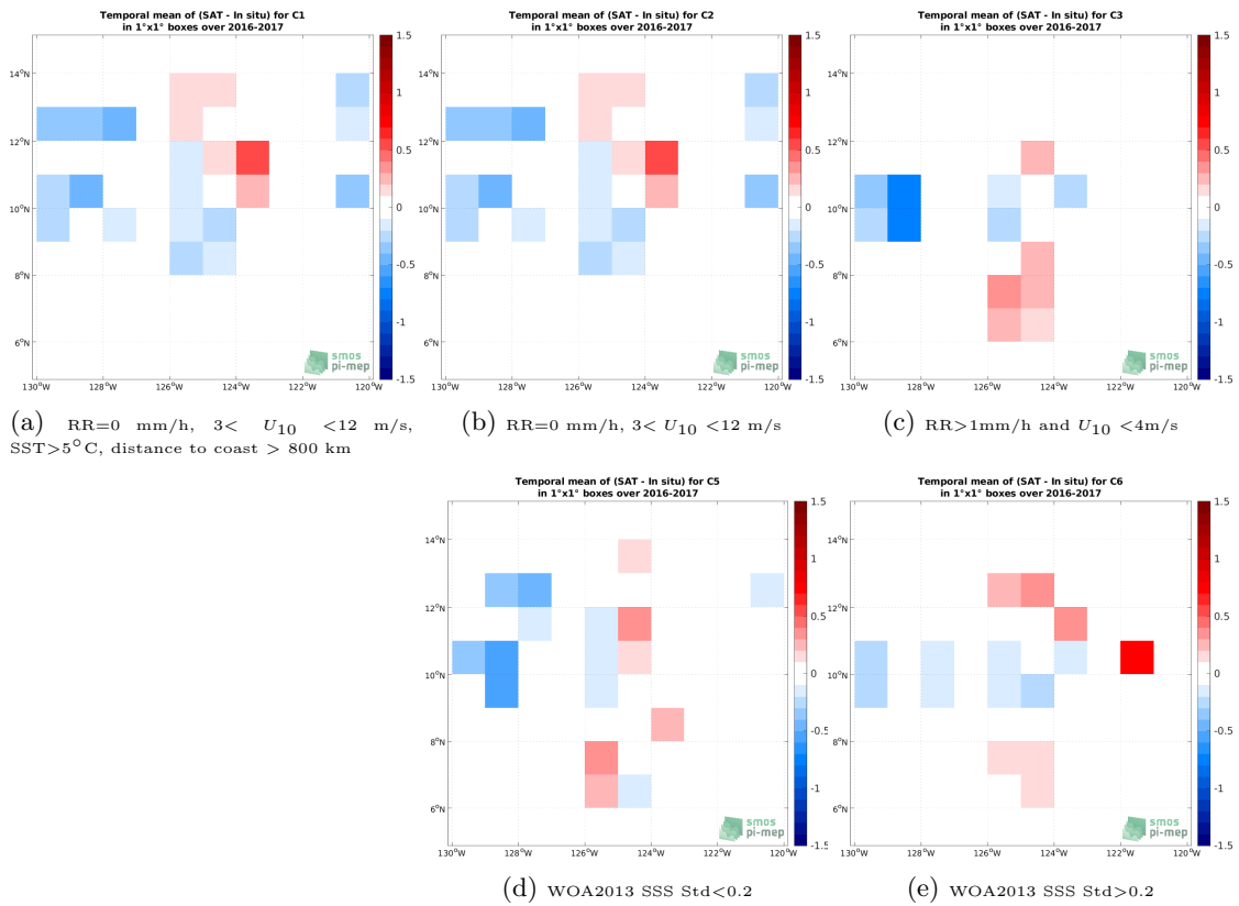
Figure 12: Temporal mean gridded over spatial boxes of size 1^\circ \times 1^\circ of \Delta SSS (SMAP SSS L3 v5 - 8-Day running (RSS) - Salinity Snake (SPURS 2)) for 5 different subdatasets corresponding to:RR=0 mm/h, 3 < U_{10} < 12 m/s, SST >5^\circ C, distance to coast > 800 km (a), RR=0 mm/h, 3 < U_{10} < 12 m/s (b), RR >1 mm/h and U_{10} < 4 m/s (c), WOA2013 SSS Std <0.2 (d), WOA2013 SSS Std >0.2 (e).
