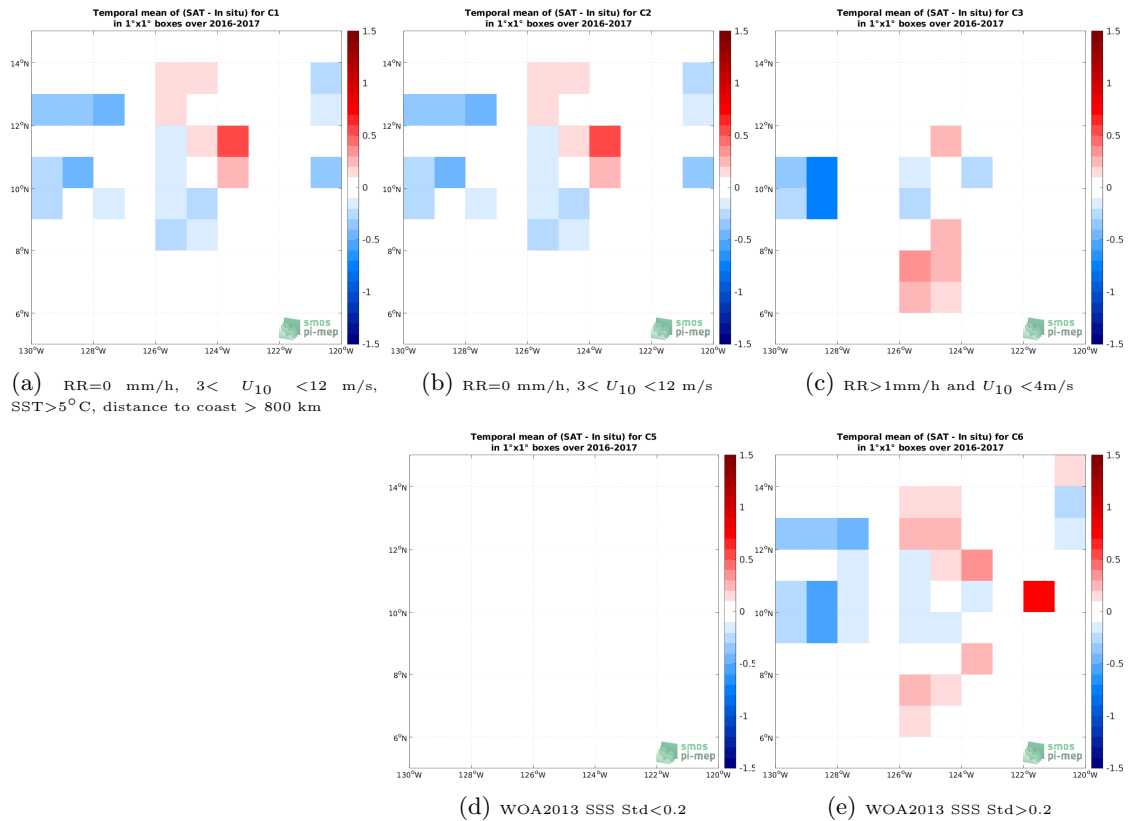
Figure 12: Temporal mean gridded over spatial boxes of size 1^\circ \times 1^\circ of \Delta SSS (SMAP SSS L3 v5 - 8-Day running (RSS) - Salinity Snake) for 5 different subdatasets corresponding to:RR=0 mm/h, 3 < U_{10} < 12 m/s, SST >5^\circ C, distance to coast > 800 km (a), RR=0 mm/h, 3 < U_{10} < 12 m/s (b), RR >1 mm/h and U_{10} < 4 m/s (c), WOA2013 SSS Std <0.2 (d), WOA2013 SSS Std >0.2 (e).
