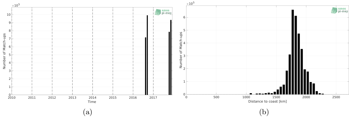
Figure 1: Number of match-ups between Salinity Snake and SMAP SSS L3 v5 - 8-Day running (RSS) SSS as a function of time (a) and as function of the distance to coast (b) over the SPURS 2 Pi-MEP region and for the full satellite product period.
