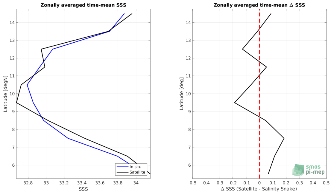
Figure 8: Left panel: Zonal mean SSS from SMAP SSS L3 v5 - 8-Day running (RSS) satellite product (black) and from Salinity Snake (blue). Right panel: Zonal mean of \Delta SSS (Satellite - Salinity Snake) for all the collected Pi-MEP match-up pairs estimated over the full satellite product period.
