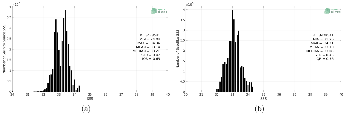
Figure 2: Histograms of SSS from Salinity Snake (a) and SMAP SSS L3 v5 - 8-Day running (RSS) (b) considering all match-up pairs per bins of 0.1 over the SPURS 2 Pi-MEP region and for the full satellite product period.
