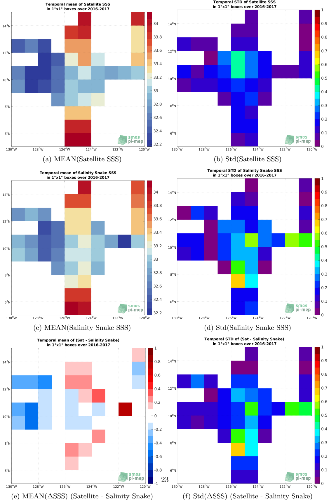
Figure 6: Temporal mean (left) and Std (right) of SSS from SMAP SSS L3 v5 - 8-Day running (RSS) (top), Salinity Snake (middle), and of \Delta SSS (Satellite - Salinity Snake). Only match-up pairs are used to generate these maps.
