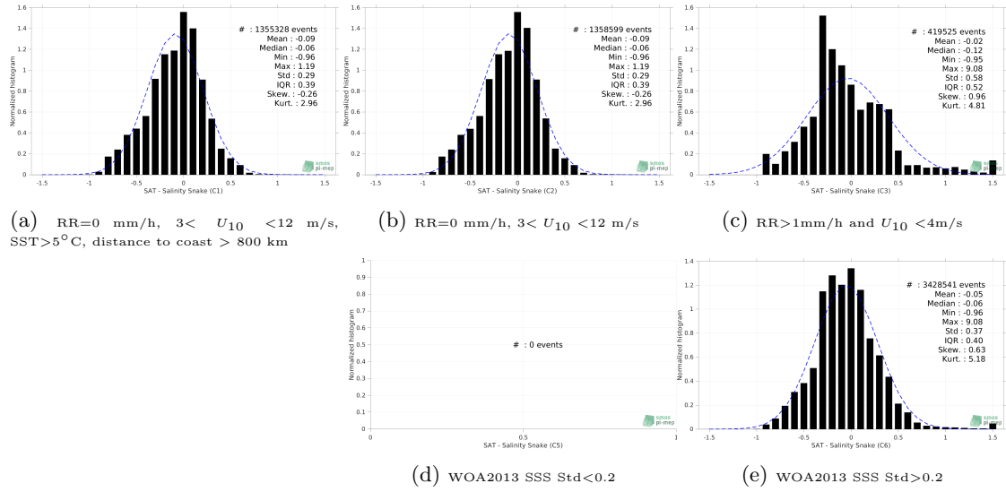
Figure 13: Normalized histogram of \Delta SSS (SMAP SSS L3 v5 - 8-Day running (RSS) - Salinity Snake) for 5 different subdatasets corresponding to: RR=0 mm/h, 3 < U_{10} < 12 m/s, SST > 5°C, distance to coast > 800 km (a), RR=0 mm/h, 3 < U_{10} < 12 m/s (b), RR > 1mm/h and U_{10} < 4 m/s (c), WOA2013 SSS Std < 0.2 (d), WOA2013 SSS Std > 0.2 (e).
