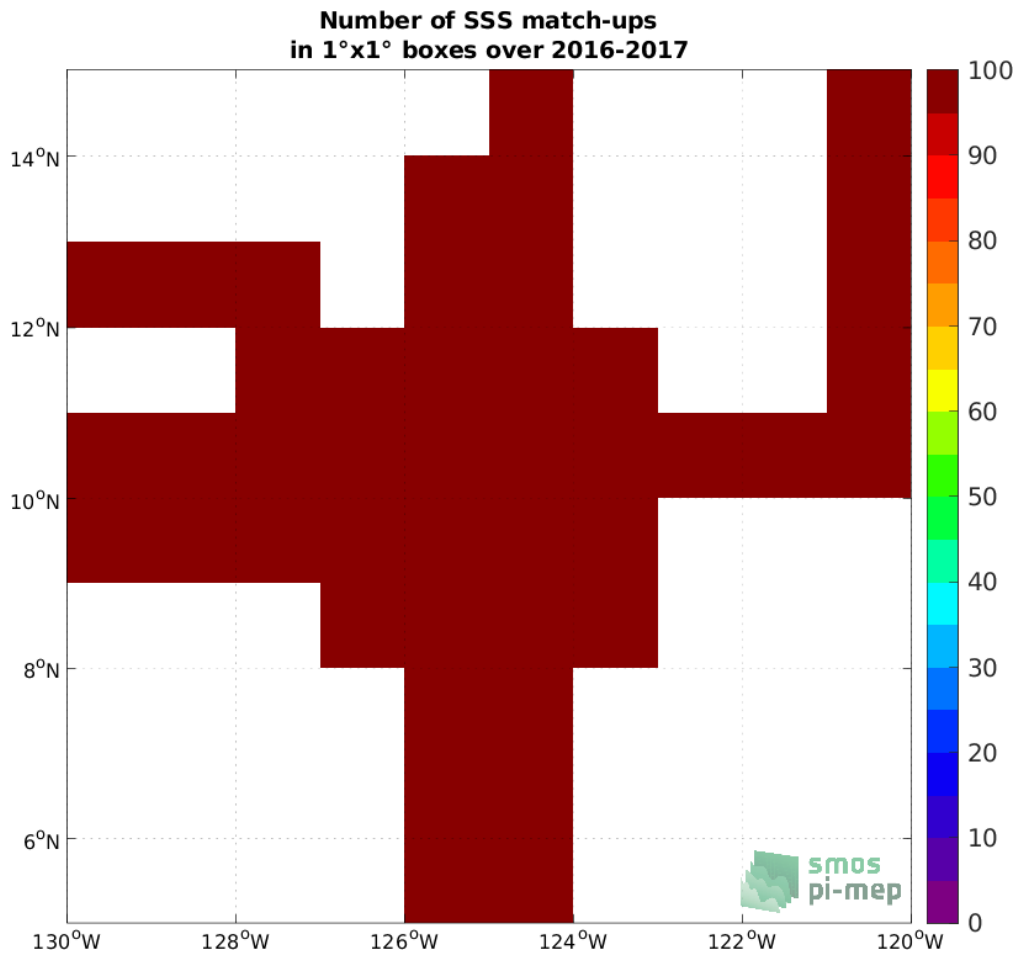
Figure 4: Number of SSS match-ups between Salinity Snake SSS and the SMAP SSS L3 v5 - 8-Day running (RSS) SSS product for the SPURS 2 Pi-MEP region over 1°x1° boxes and for the full satellite product period.
