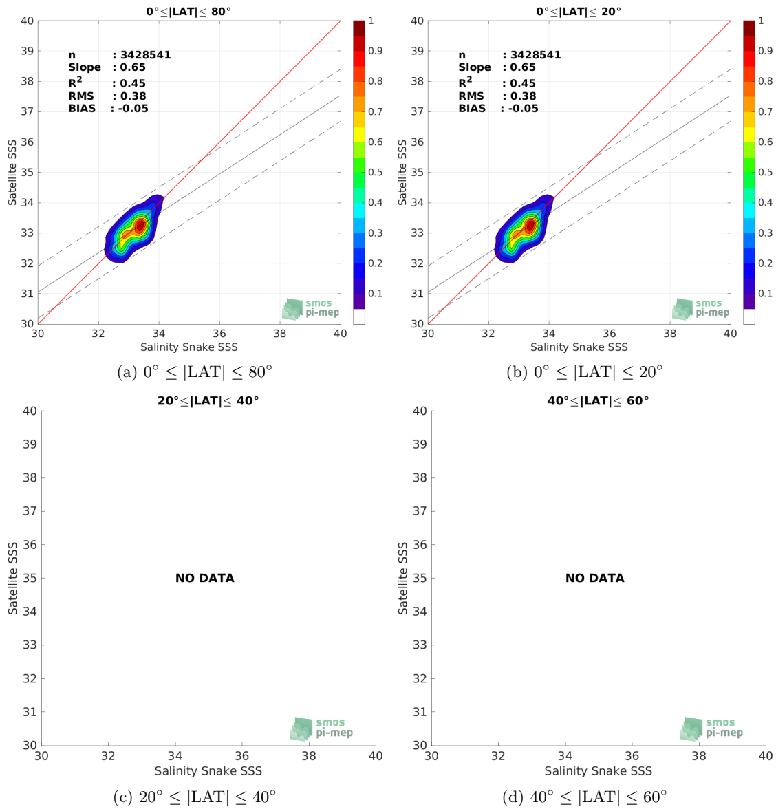
Figure 9: Contour maps of the concentration of SMAP SSS L3 v5 - 8-Day running (RSS) SSS (y-axis) versus Salinity Snake SSS (x-axis) at match-up pairs for different latitude bands. For each plot, the red line shows x=y . The black thin and dashed lines indicate a linear fit through the data cloud and the \pm 95\% confidence levels, respectively. The number match-up pairs n , the slope and R^2 coefficient of the linear fit, the root mean square (RMS) and the mean bias between satellite and in situ data are indicated for each latitude band in each plots.
