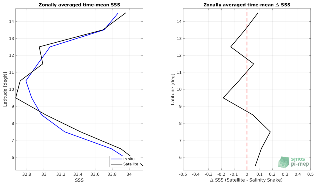
Figure 7: Left panel: Zonal mean SSS from SMAP SSS L3 v5 - 8-Day running (RSS) satellite product (black) and from Salinity Snake (blue). Right panel: Zonal mean of \Delta SSS (Satellite - Salinity Snake) for all the collected Pi-MEP match-up pairs estimated over the full satellite product period.
