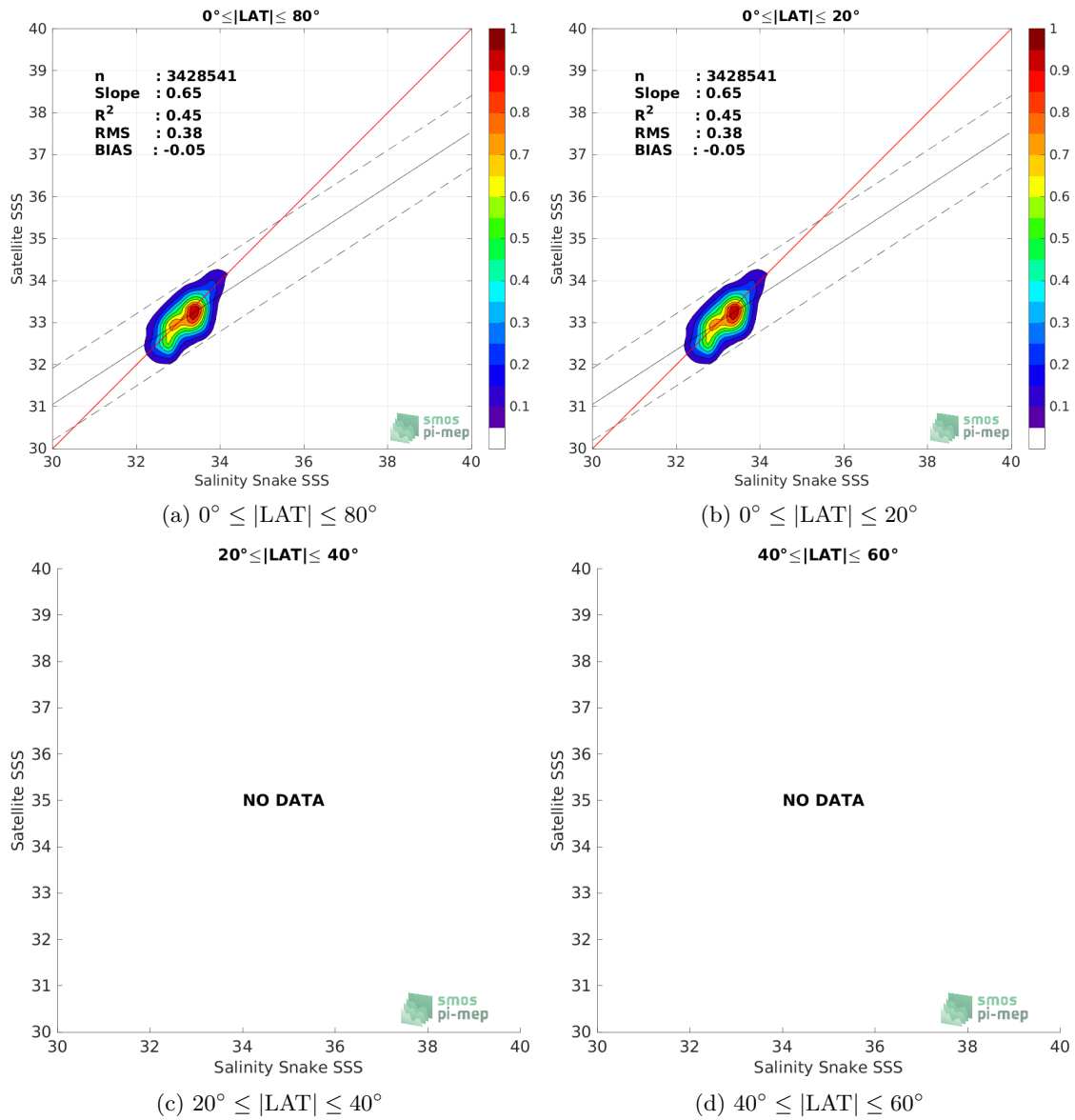
Figure 8: Contour maps of the concentration of SMAP SSS L3 v5 - 8-Day running (RSS) SSS (y-axis) versus Salinity Snake SSS (x-axis) at match-up pairs for different latitude bands. For each plot, the red line shows x=y . The black thin and dashed lines indicate a linear fit through the data cloud and the \pm 95\% confidence levels, respectively. The number match-up pairs n , the slope and R^2 coefficient of the linear fit, the root mean square (RMS) and the mean bias between satellite and in situ data are indicated for each latitude band in each plots.
