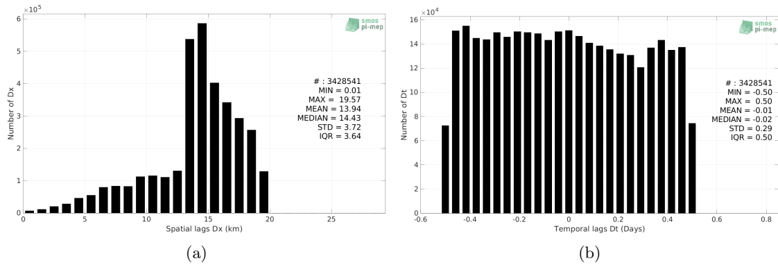
Figure 4: Histograms of the spatial (a) and temporal (b) lags between the location/time of the Salinity Snake measurement and the date of the corresponding SMAP SSS L3 v5 - 8-Day running (RSS) SSS pixel.
