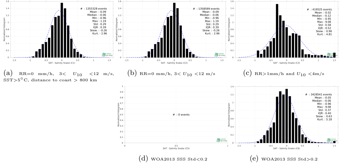
Figure 12: Normalized histogram of \Delta SSS (SMAP SSS L3 v5 - 8-Day running (RSS) - Salinity Snake) for 5 different subdatasets corresponding to: RR=0 mm/h, 3 < U_{10} < 12 m/s, SST > 5°C, distance to coast > 800 km (a), RR=0 mm/h, 3 < U_{10} < 12 m/s (b), RR > 1mm/h and U_{10} < 4 m/s (c), WOA2013 SSS Std < 0.2 (d), WOA2013 SSS Std > 0.2 (e).
