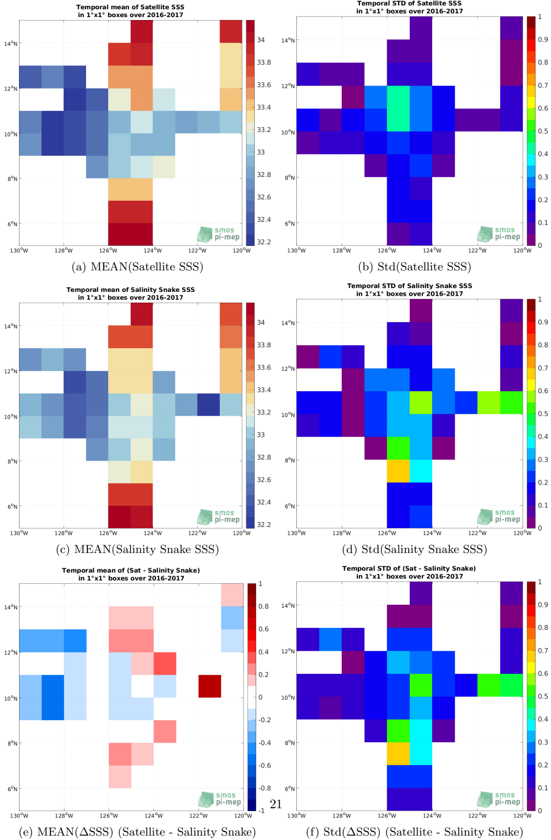
Figure 5: Temporal mean (left) and Std (right) of SSS from SMAP SSS L3 v5 - 8-Day running (RSS) (top), Salinity Snake (middle), and of \Delta SSS (Satellite - Salinity Snake). Only match-up pairs are used to generate these maps.
