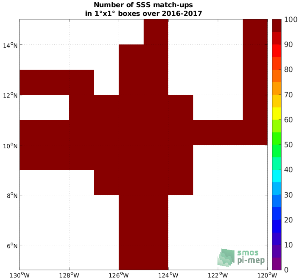
Figure 3: Number of SSS match-ups between Salinity Snake SSS and the SMAP SSS L3 v5 - 8-Day running (RSS) SSS product for the SPURS 2 Pi-MEP region over 1^\circ \times 1^\circ boxes and for the full satellite product period.
