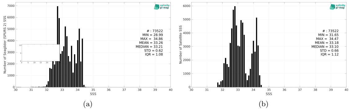
Figure 2: Histograms of SSS from Seaglider (SPURS 2) (a) and SMAP SSS L3 v5 - 8-Day running (RSS) (b) considering all match-up pairs per bins of 0.1 over the SPURS 2 Pi-MEP region and for the full satellite product period.
