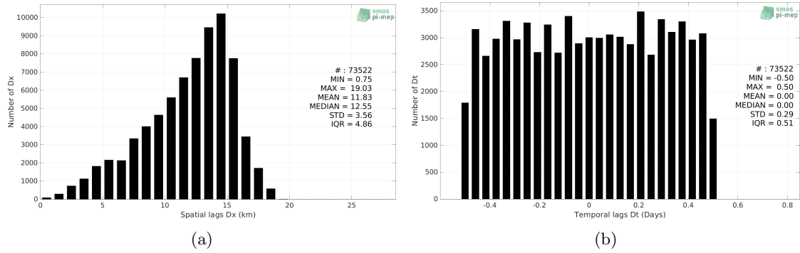
Figure 5: Histograms of the spatial (a) and temporal (b) lags between the location/time of the Seaglider (SPURS 2) measurement and the date of the corresponding SMAP SSS L3 v5 - 8-Day running (RSS) SSS pixel.
