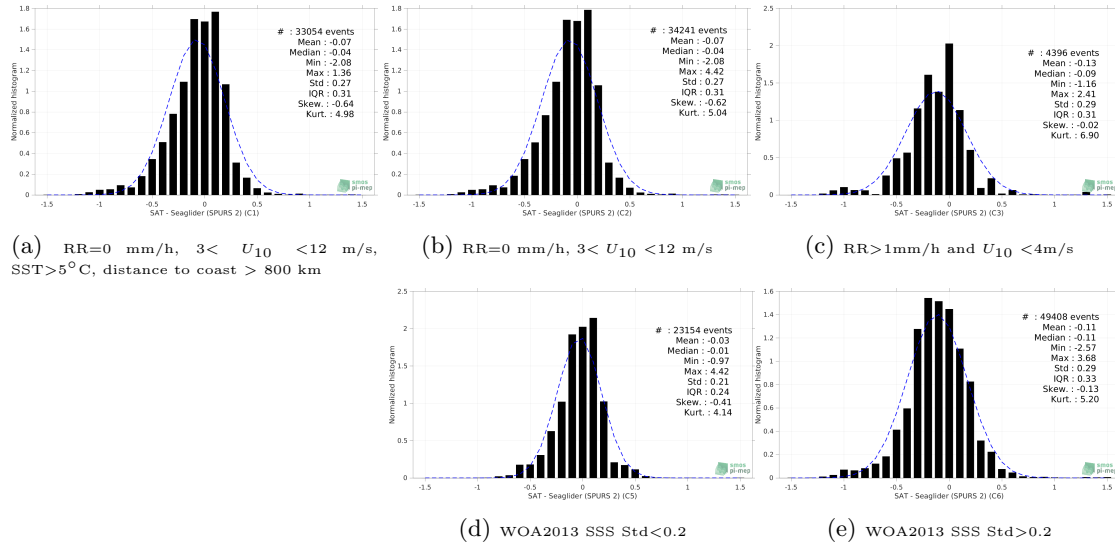
Figure 13: Normalized histogram of \Delta SSS (SMAP SSS L3 v5 - 8-Day running (RSS) - Seaglider (SPURS 2)) for 5 different subdatasets corresponding to: RR=0 mm/h, 3 < U_{10} < 12 m/s, SST > 5°C, distance to coast > 800 km (a), RR=0 mm/h, 3 < U_{10} < 12 m/s (b), RR > 1mm/h and U_{10} < 4 m/s (c), WOA2013 SSS Std < 0.2 (d), WOA2013 SSS Std > 0.2 (e).
