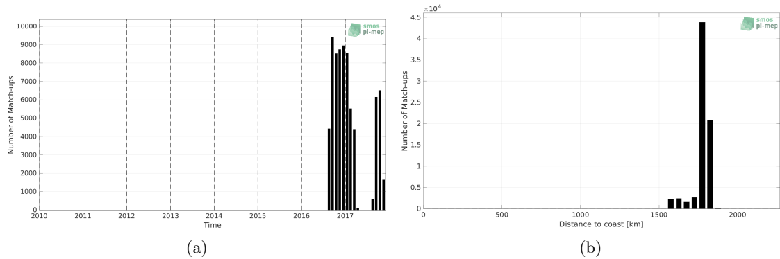
Figure 1: Number of match-ups between Seaglider (SPURS 2) and SMAP SSS L3 v5 - 8-Day running (RSS) SSS as a function of time (a) and as function of the distance to coast (b) over the SPURS 2 Pi-MEP region and for the full satellite product period.
