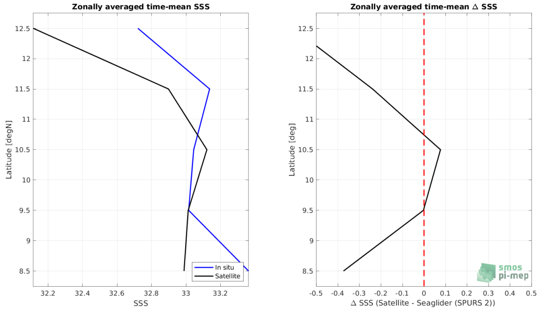
Figure 8: Left panel: Zonal mean SSS from SMAP SSS L3 v5 - 8-Day running (RSS) satellite product (black) and from Seaglider (SPURS 2) (blue). Right panel: Zonal mean of \Delta SSS (Satellite - Seaglider (SPURS 2)) for all the collected Pi-MEP match-up pairs estimated over the full satellite product period.
