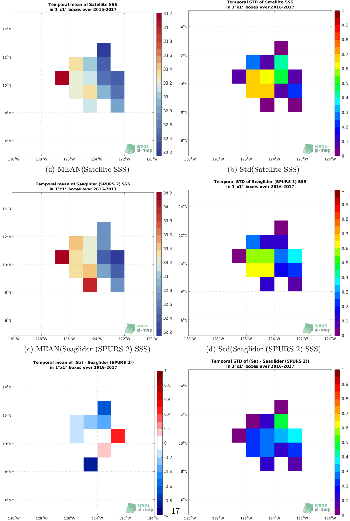
Figure 6: Temporal mean (left) and Std (right) of SSS from SMAP SSS L3 v5 - 8-Day running (RSS) (top), Seaglider (SPURS 2) (middle), and of \Delta SSS (Satellite - Seaglider (SPURS 2)). Only match-up pairs are used to generate these maps.
