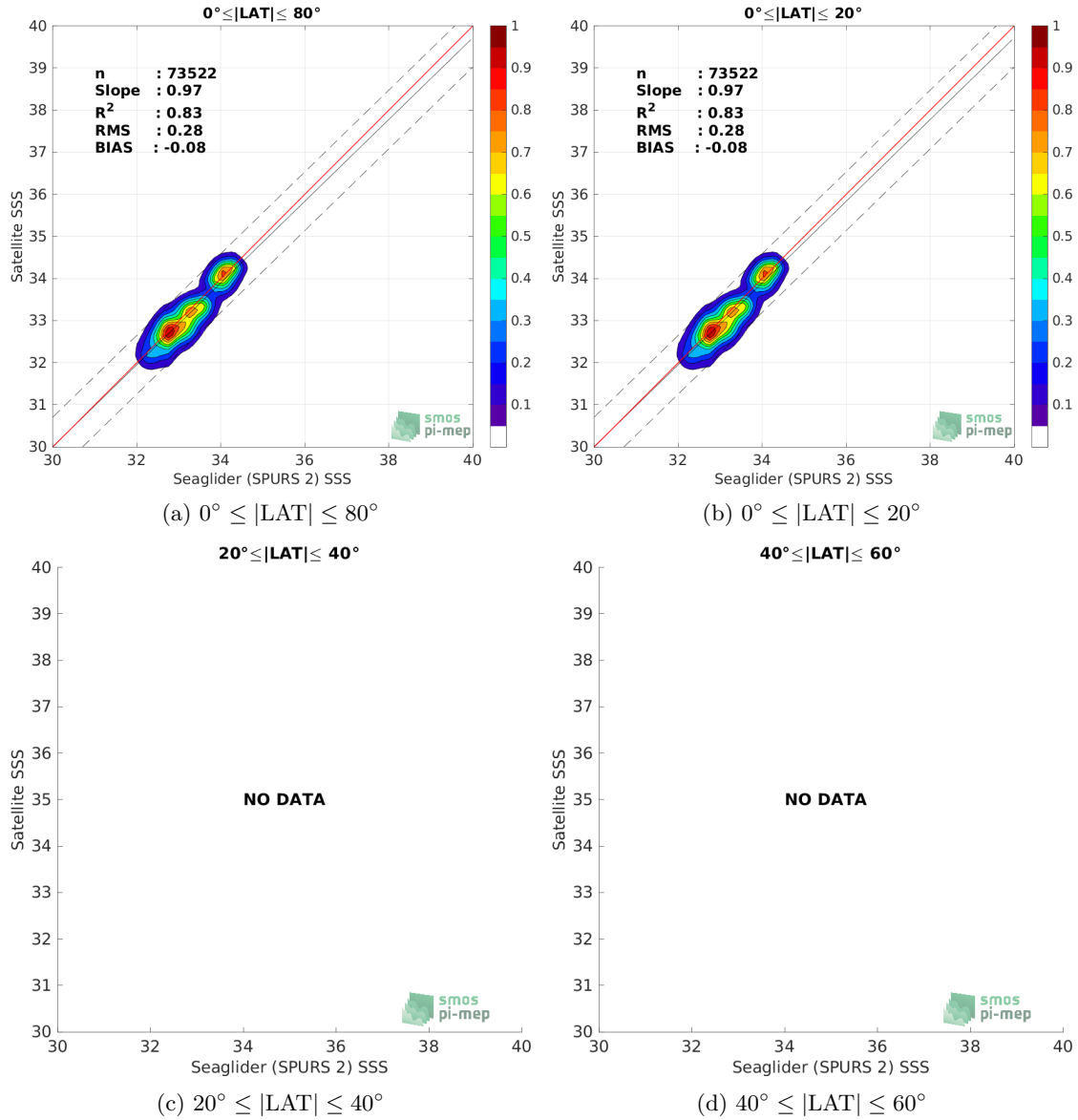
Figure 9: Contour maps of the concentration of SMAP SSS L3 v5 - 8-Day running (RSS) SSS (y-axis) versus Seaglider (SPURS 2) SSS (x-axis) at match-up pairs for different latitude bands. For each plot, the red line shows x=y . The black thin and dashed lines indicate a linear fit through the data cloud and the \pm 95\% confidence levels, respectively. The number match-up pairs n , the slope and R^2 coefficient of the linear fit, the root mean square (RMS) and the mean bias between satellite and in situ data are indicated for each latitude band in each plots.
