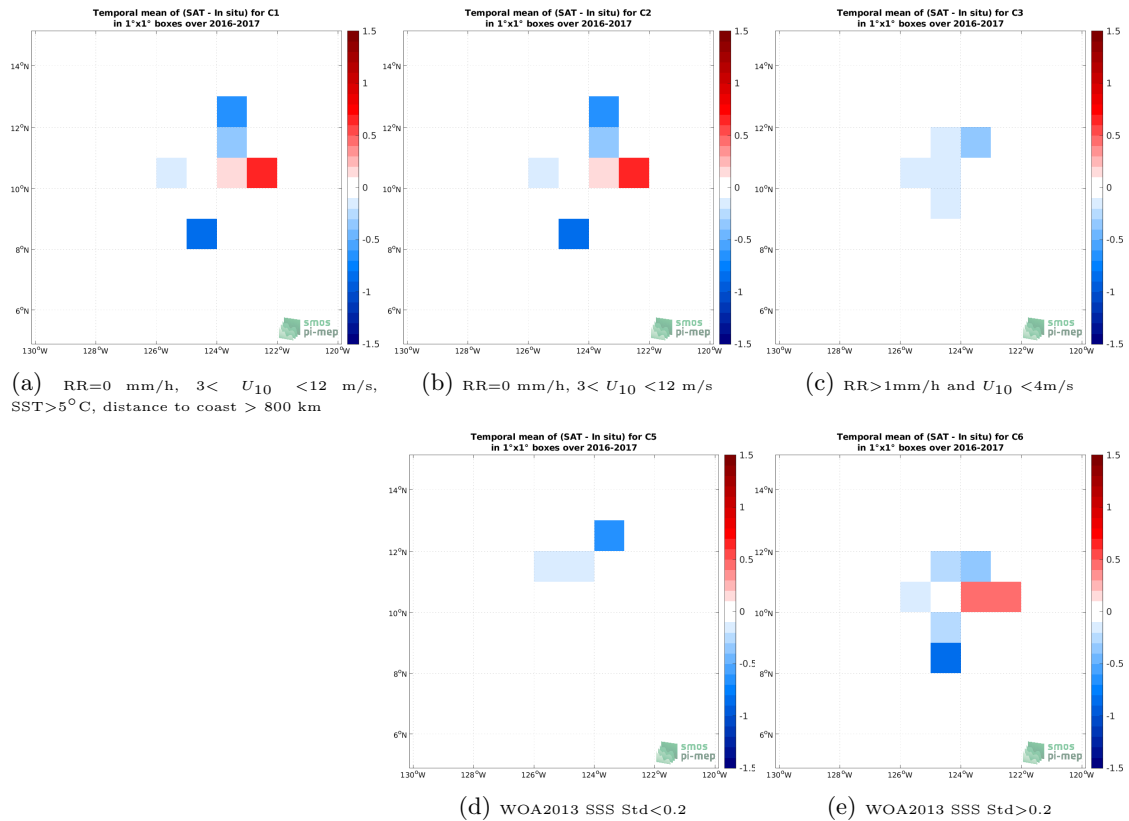
Figure 12: Temporal mean gridded over spatial boxes of size 1^\circ \times 1^\circ of \Delta SSS (SMAP SSS L3 v5 - 8-Day running (RSS) - Seaglider (SPURS 2)) for 5 different subdatasets corresponding to:RR=0 mm/h, 3 < U_{10} < 12 m/s, SST >5^\circ\text{C} , distance to coast > 800 km (a), RR=0 mm/h, 3 < U_{10} < 12 m/s (b), RR >1 mm/h and U_{10} < 4 m/s (c), WOA2013 SSS Std <0.2 (d), WOA2013 SSS Std >0.2 (e).
