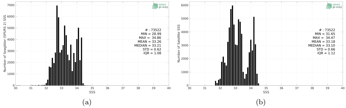
Figure 2: Histograms of SSS from Seagliders (SPURS 2) (a) and SMAP SSS L3 v5 - 8-Day running (RSS) (b) considering all match-up pairs per bins of 0.1 over the SPURS 2 Pi-MEP region and for the full satellite product period.
