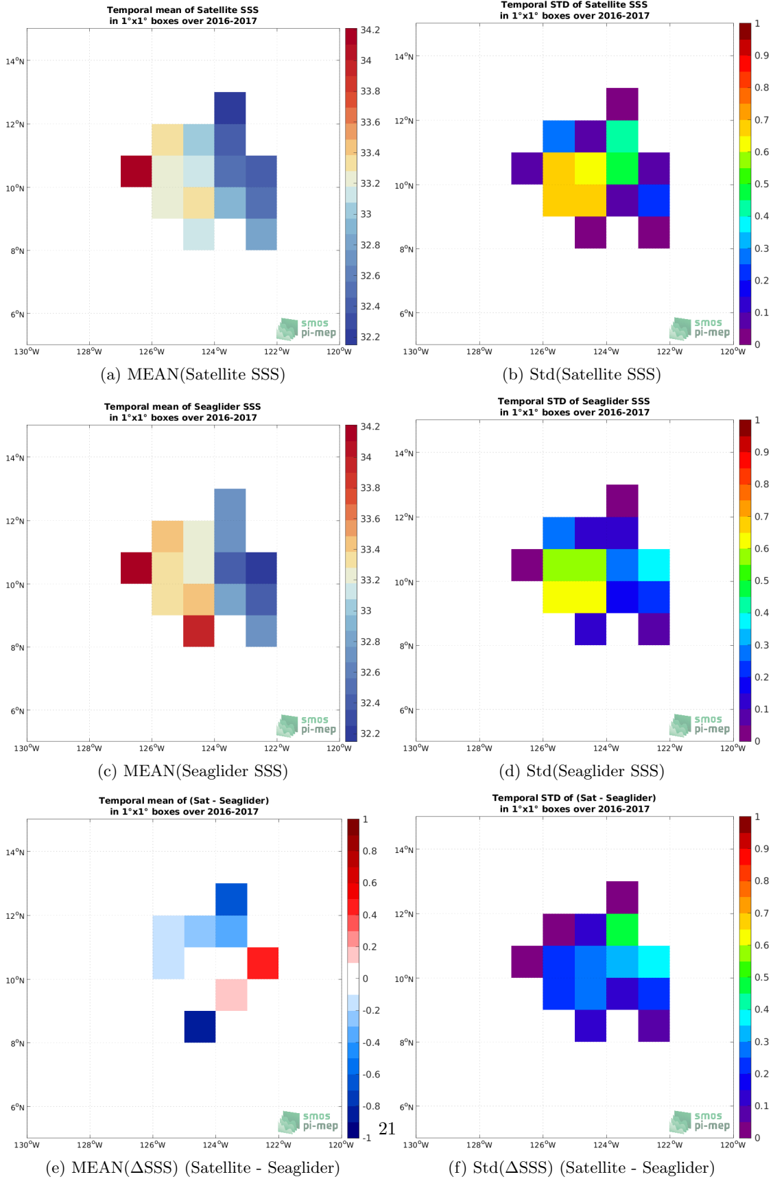
Figure 5: Temporal mean (left) and Std (right) of SSS from SMAP SSS L3 v5 - 8-Day running (RSS) (top), Seaglider (middle), and of \Delta SSS (Satellite - Seaglider). Only match-up pairs are used to generate these maps.
