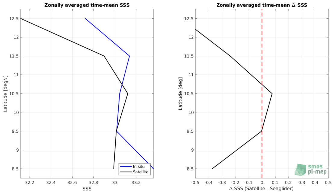
Figure 7: Left panel: Zonal mean SSS from SMAP SSS L3 v5 - 8-Day running (RSS) satellite product (black) and from Seaglider (blue). Right panel: Zonal mean of \Delta SSS (Satellite - Seaglider) for all the collected Pi-MEP match-up pairs estimated over the full satellite product period.
