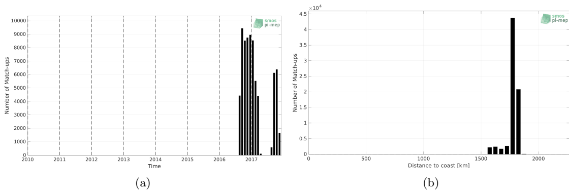
Figure 1: Number of match-ups between Seaglider and SMAP SSS L3 v5 - 8-Day running (RSS) SSS as a function of time (a) and as function of the distance to coast (b) over the SPURS 2 Pi-MEP region and for the full satellite product period.
