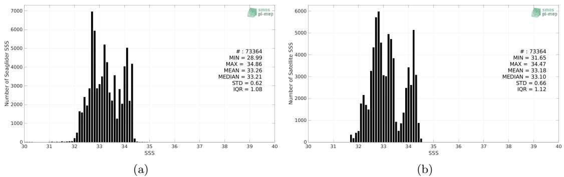
Figure 2: Histograms of SSS from Seaglider (a) and SMAP SSS L3 v5 - 8-Day running (RSS) (b) considering all match-up pairs per bins of 0.1 over the SPURS 2 Pi-MEP region and for the full satellite product period.
