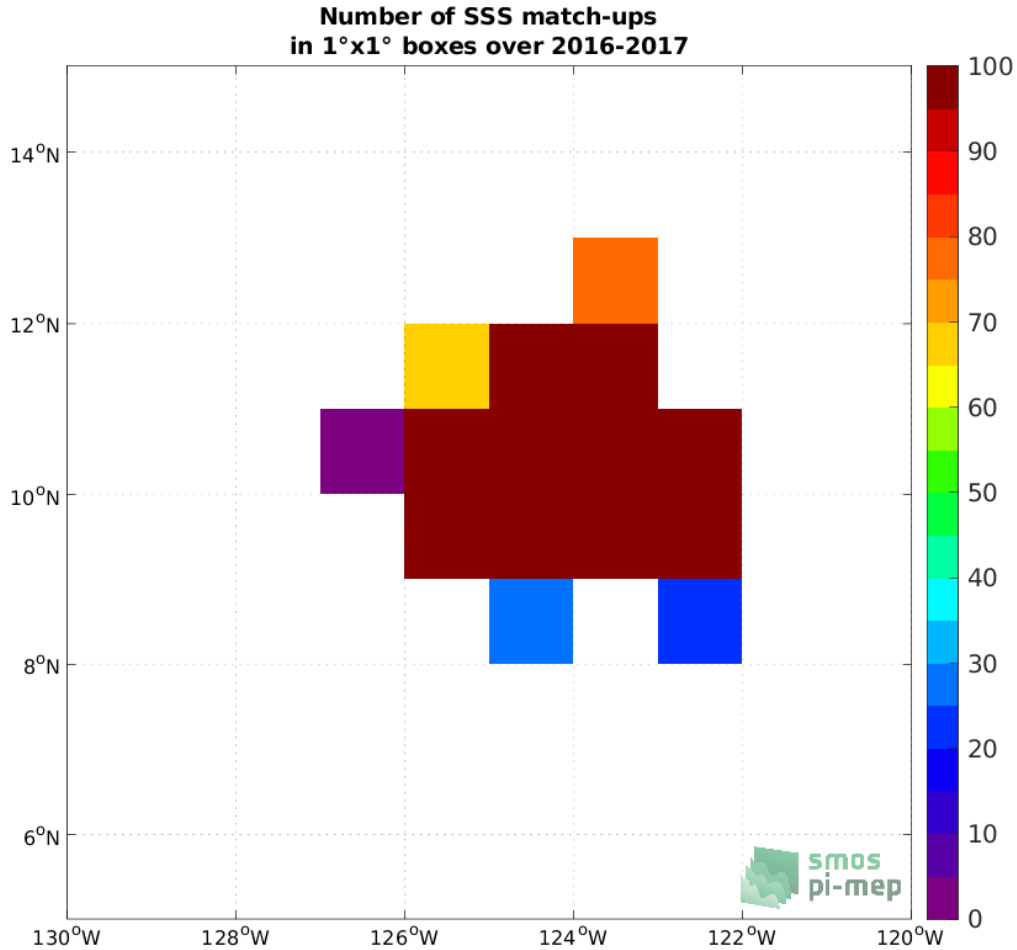
Figure 3: Number of SSS match-ups between Seagliders SSS and the SMAP SSS L3 v5 - 8-Day running (RSS) SSS product for the SPURS 2 Pi-MEP region over 1^\circ \times 1^\circ boxes and for the full satellite product period.
