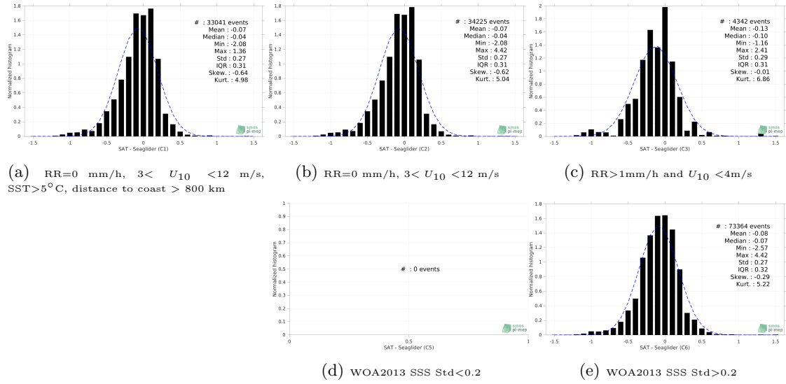
Figure 12: Normalized histogram of \Delta SSS (SMAP SSS L3 v5 - 8-Day running (RSS) - Seaglider) for 5 different subdatasets corresponding to: RR=0 mm/h, 3 < U_{10} < 12 m/s, SST > 5°C, distance to coast > 800 km (a), RR=0 mm/h, 3 < U_{10} < 12 m/s (b), RR > 1mm/h and U_{10} < 4 m/s (c), WOA2013 SSS Std < 0.2 (d), WOA2013 SSS Std > 0.2 (e).
