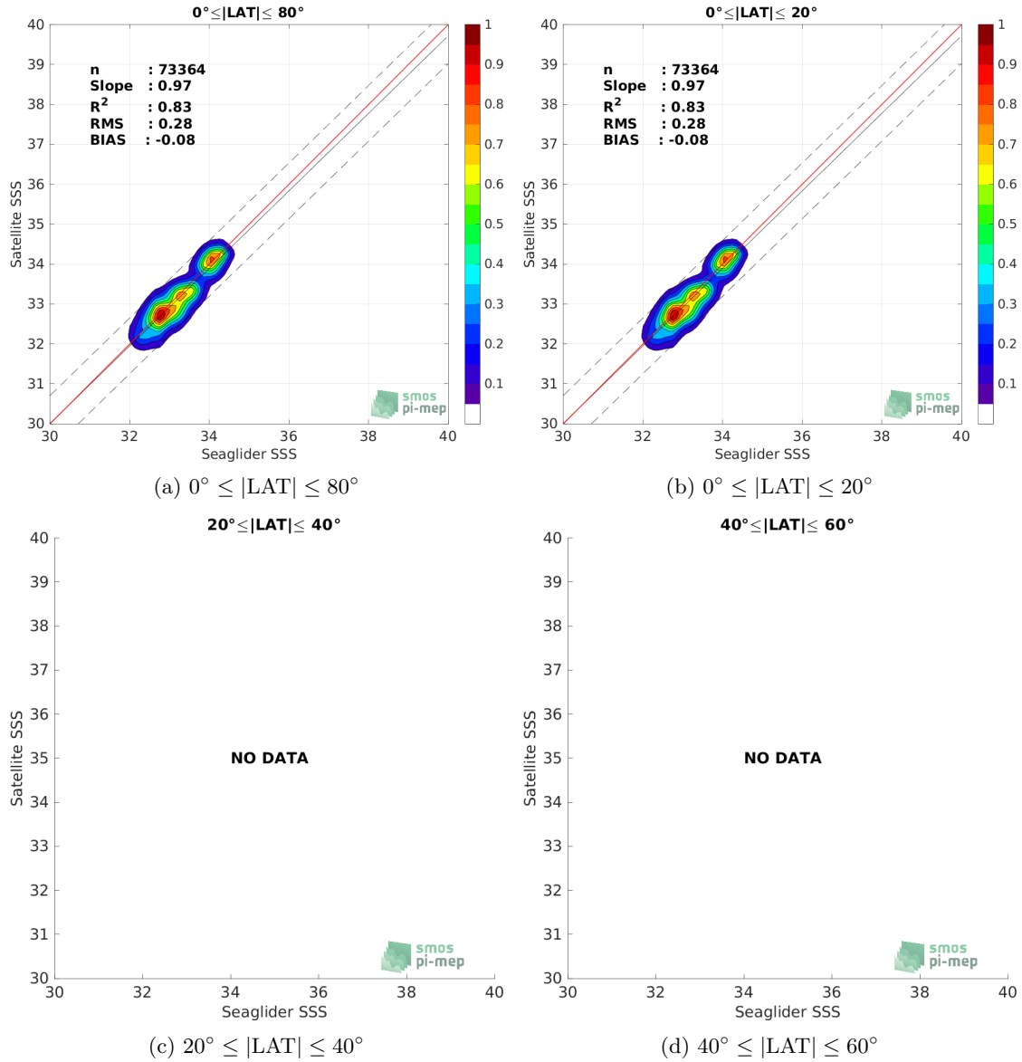
Figure 8: Contour maps of the concentration of SMAP SSS L3 v5 - 8-Day running (RSS) SSS (y-axis) versus Seaglider SSS (x-axis) at match-up pairs for different latitude bands. For each plot, the red line shows x=y . The black thin and dashed lines indicate a linear fit through the data cloud and the \pm 95\% confidence levels, respectively. The number match-up pairs n , the slope and R^2 coefficient of the linear fit, the root mean square (RMS) and the mean bias between satellite and in situ data are indicated for each latitude band in each plots.
