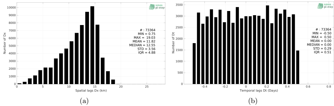
Figure 4: Histograms of the spatial (a) and temporal (b) lags between the location/time of the Seaglider measurement and the date of the corresponding SMAP SSS L3 v5 - 8-Day running (RSS) SSS pixel.
