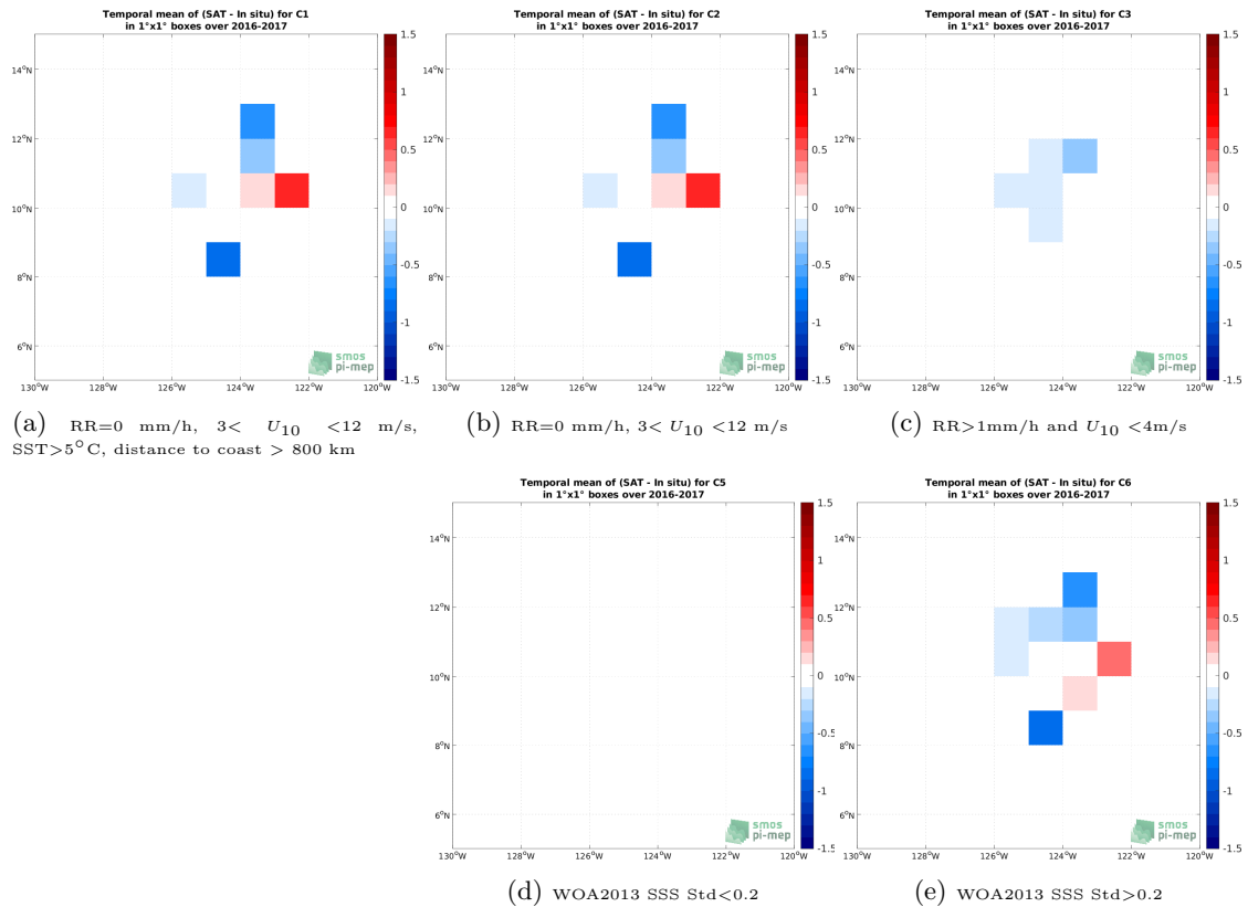
Figure 11: Temporal mean gridded over spatial boxes of size 1^\circ \times 1^\circ of \Delta\text{SSS} (SMAP SSS L3 v5 - 8-Day running (RSS) - Seaglider) for 5 different subdatasets corresponding to:RR=0 mm/h, 3 < U_{10} < 12 m/s, SST > 5^\circ\text{C} , distance to coast > 800 km (a), RR=0 mm/h, 3 < U_{10} < 12 m/s (b), RR > 1 mm/h and U_{10} < 4 m/s (c), WOA2013 SSS Std < 0.2 (d), WOA2013 SSS Std > 0.2 (e).
